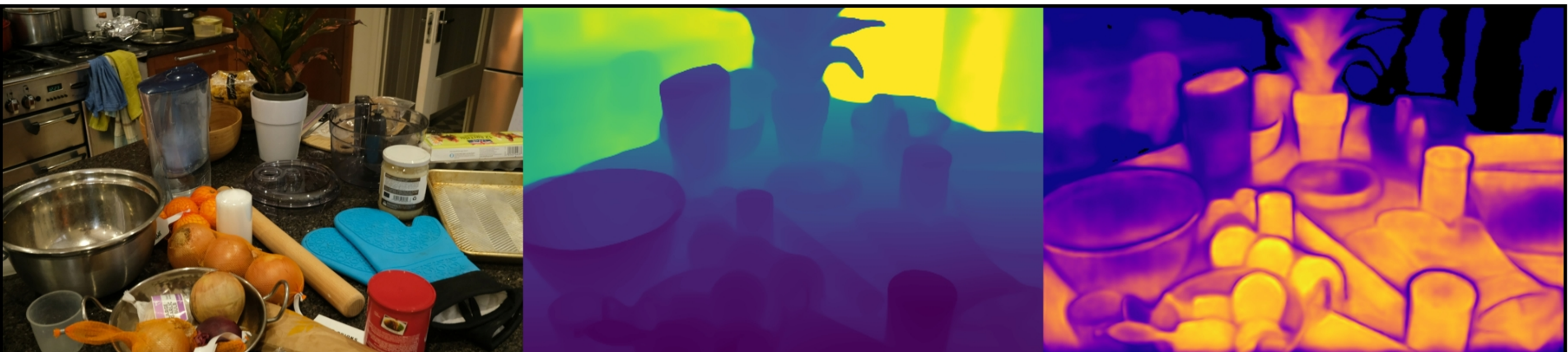
counter: VGGT Original | Depth (max=2.77) | Confidence (max=15.05)
