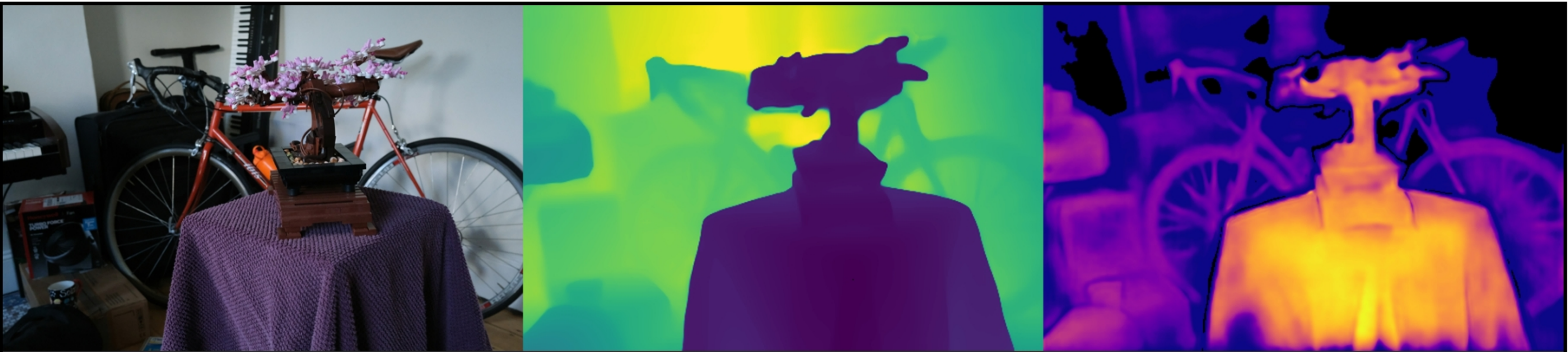
bonsai: VGGT Original | Depth (max=2.22) | Confidence (max=3.91)
