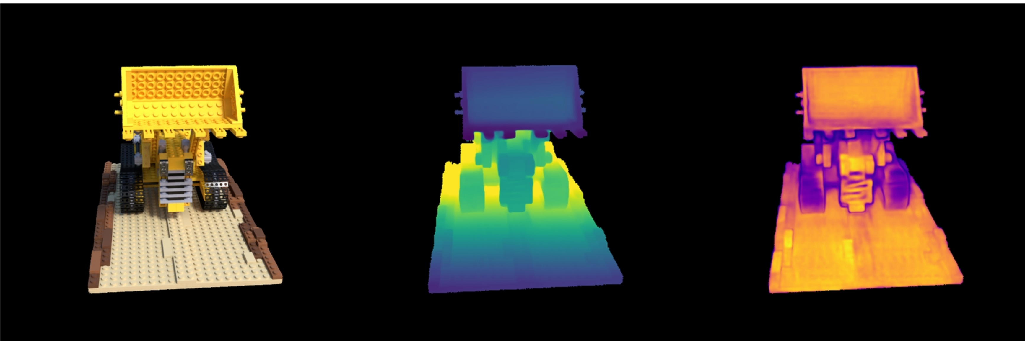
lego: VGGT Original | Depth (max=1.28) | Confidence (max=17.85)
