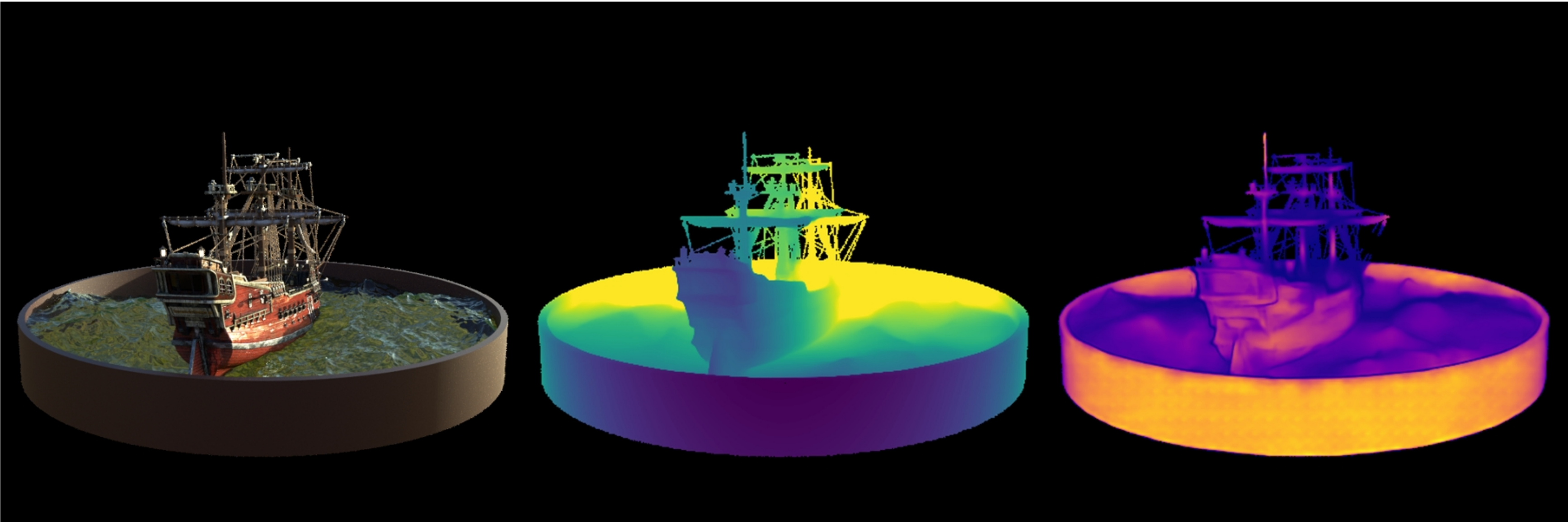
ship: VGGT Original | Depth (max=1.30) | Confidence (max=149.31)
