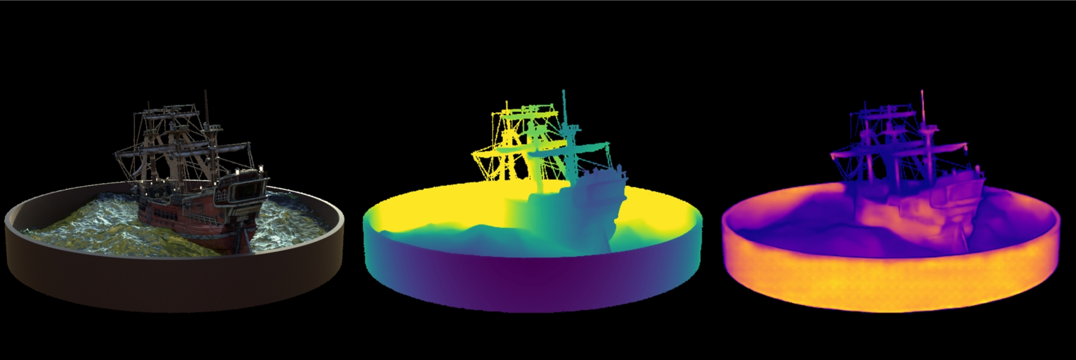
ship: VGGT | num_images=20 Original | Depth (max=1.29) | Confidence (max=160.96)
