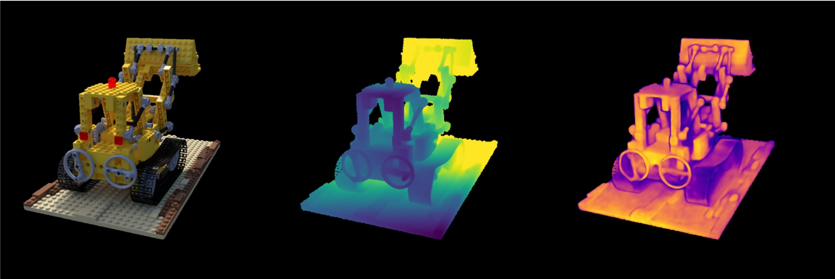
lego: VGGT | num_images=40 Original | Depth (max=1.32) | Confidence (max=38.45)
