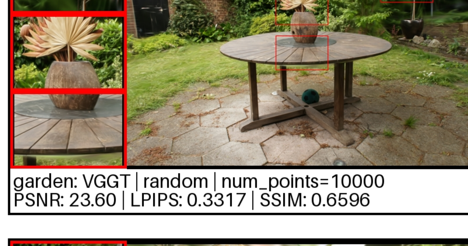
garden: VGGT | random | num_points=10000 PSNR: 23.60 | LPIPS: 0.3317 | SSIM: 0.6596
