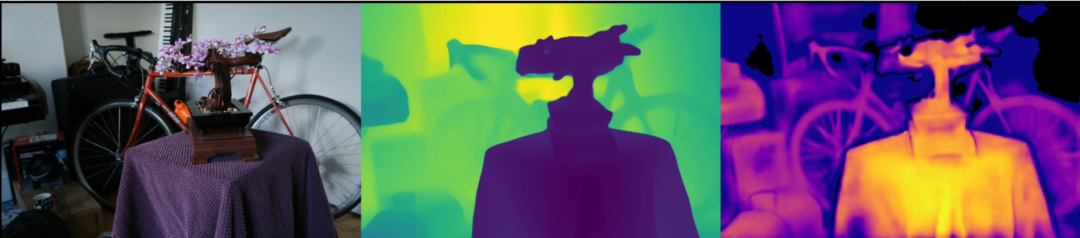
bonsai: VGGT | random | num_points=1000000 Original | Depth (max=2.21) | Confidence (max=5.14)
