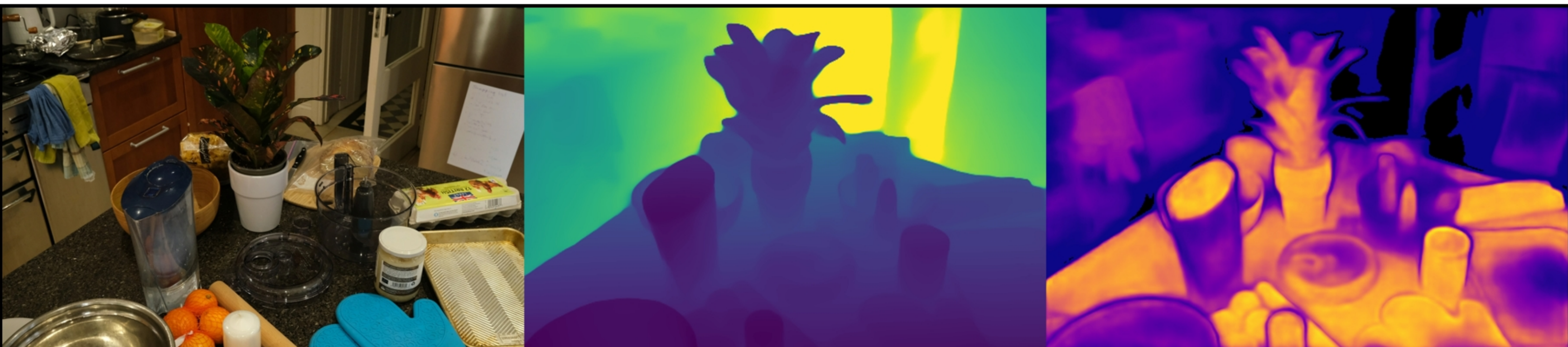
counter: VGGT | random | num_points=1000 Original | Depth (max=2.88) | Confidence (max=15.71)
