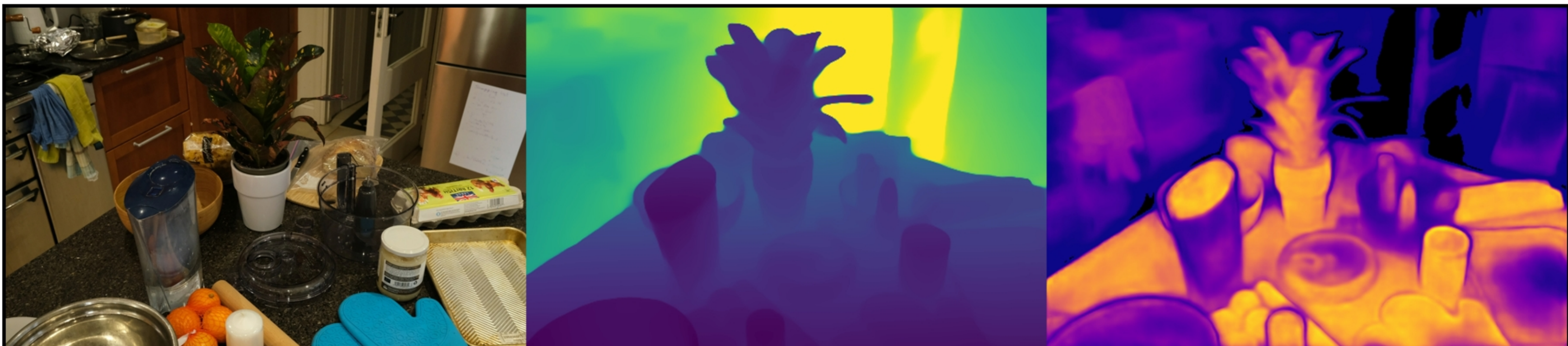
counter: VGGT | random | num_points=100000 Original | Depth (max=2.88) | Confidence (max=15.71)
