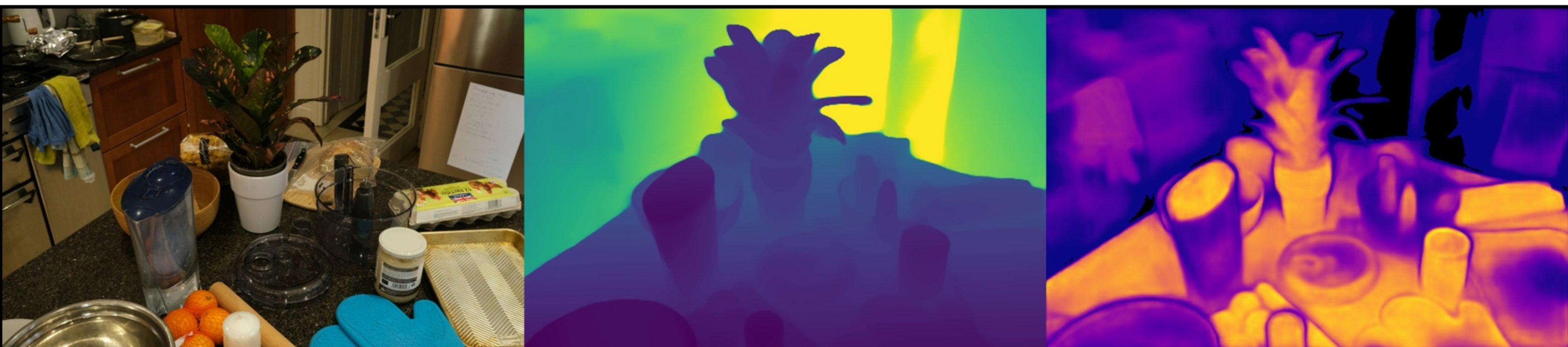
counter: VGGT | random | num_points=1000000 Original | Depth (max=2.88) | Confidence (max=15.71)
