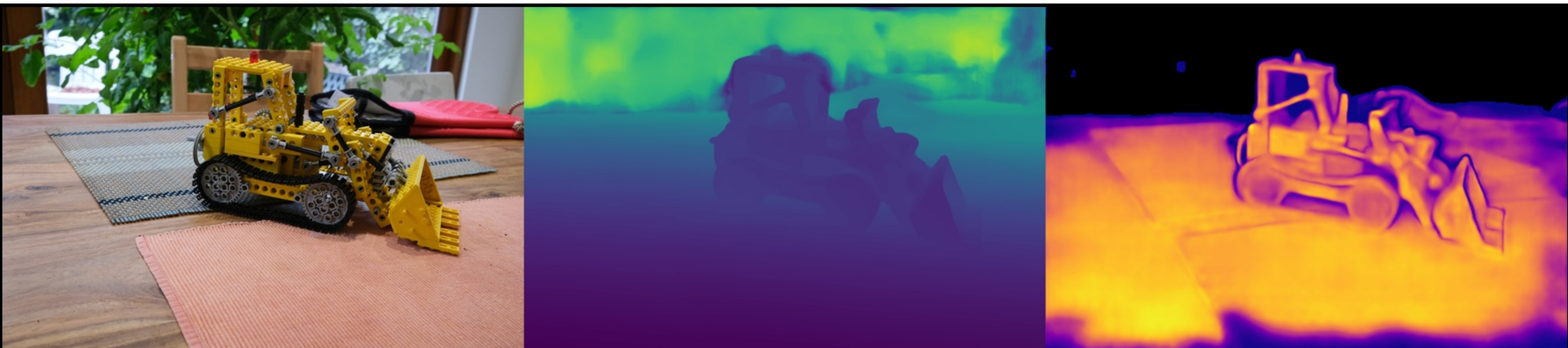
kitchen: VGGT | random | num_points=1000 Original | Depth (max=2.43) | Confidence (max=30.80)
