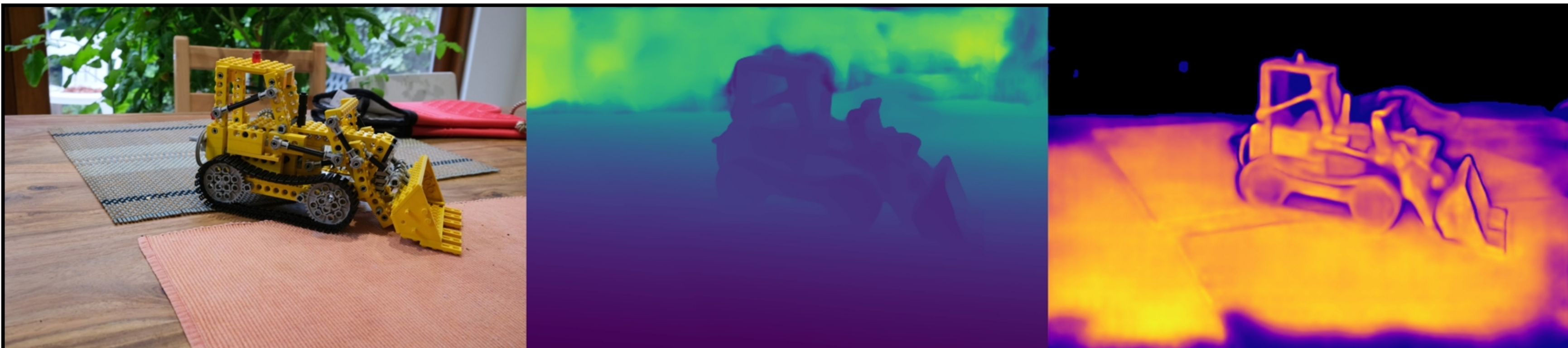
kitchen: VGGT | random | num_points=10000 Original | Depth (max=2.43) | Confidence (max=30.80)
