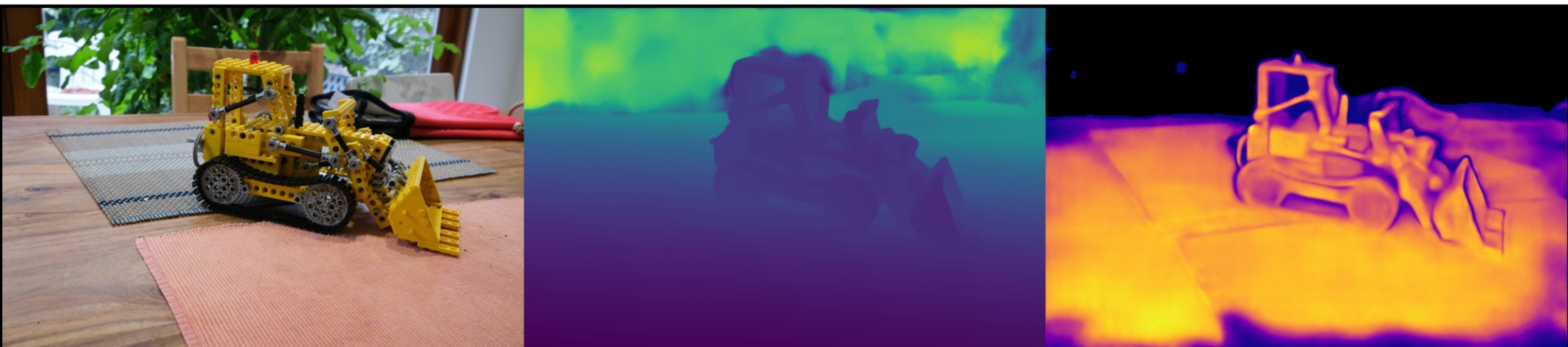
kitchen: VGGT | random | num_points=1000000 Original | Depth (max=2.43) | Confidence (max=30.80)
