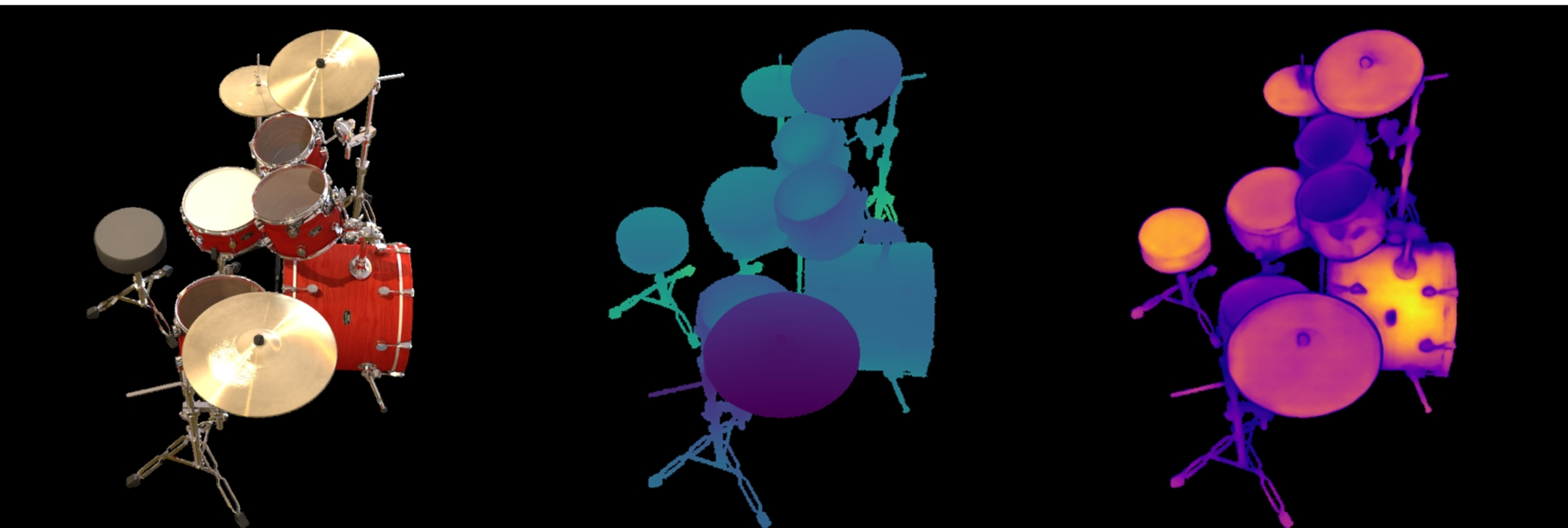
drums: VGGT | random | num_points=870 Original | Depth (max=1.20) | Confidence (max=303.06)
