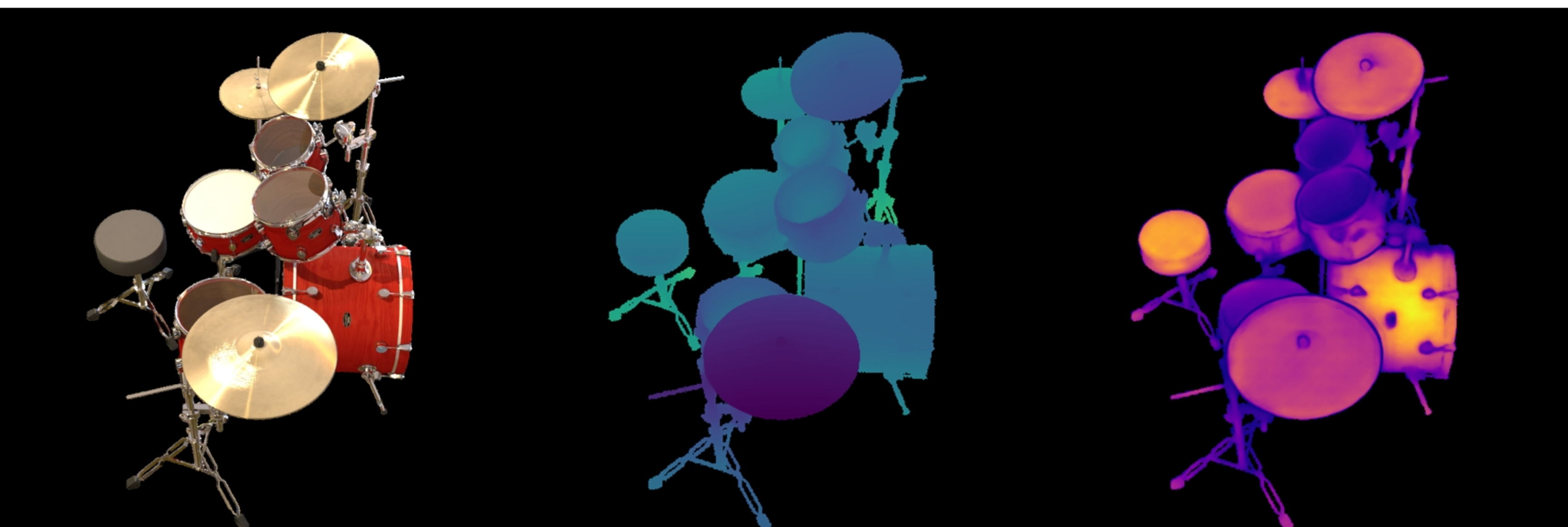
drums: VGGT | random | num_points=870000 Original | Depth (max=1.20) | Confidence (max=303.06)
