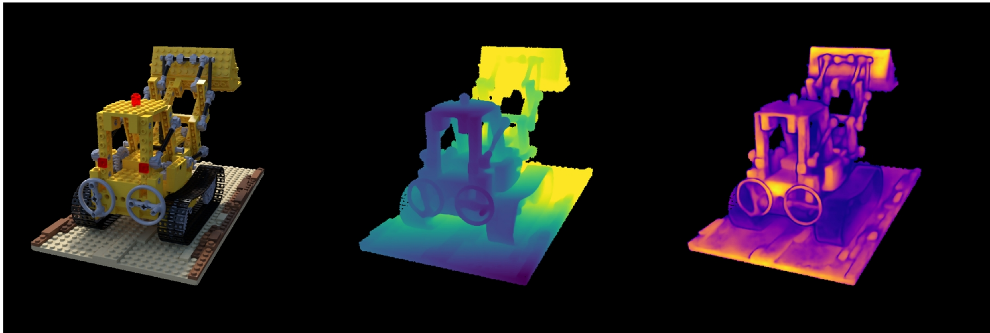
lego: VGGT | random | num_points=8700 Original | Depth (max=1.28) | Confidence (max=155.74)
