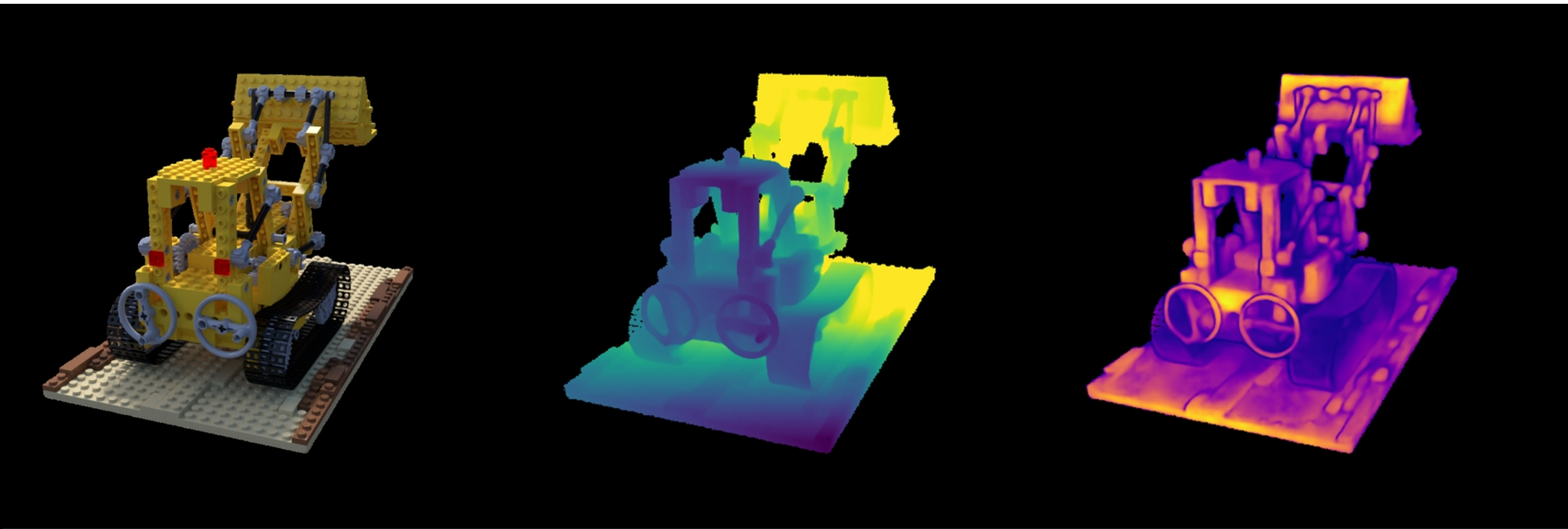
lego: VGGT | random | num_points=870 Original | Depth (max=1.28) | Confidence (max=155.74)
