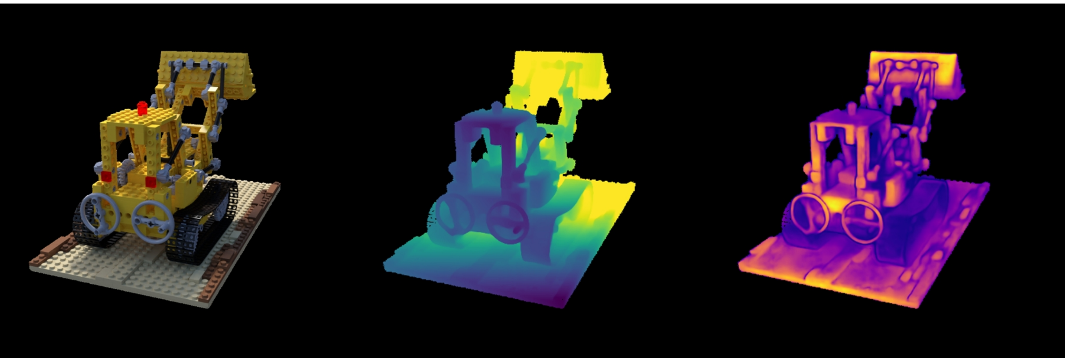
lego: VGGT | random | num_points=870000 Original | Depth (max=1.28) | Confidence (max=155.74)
