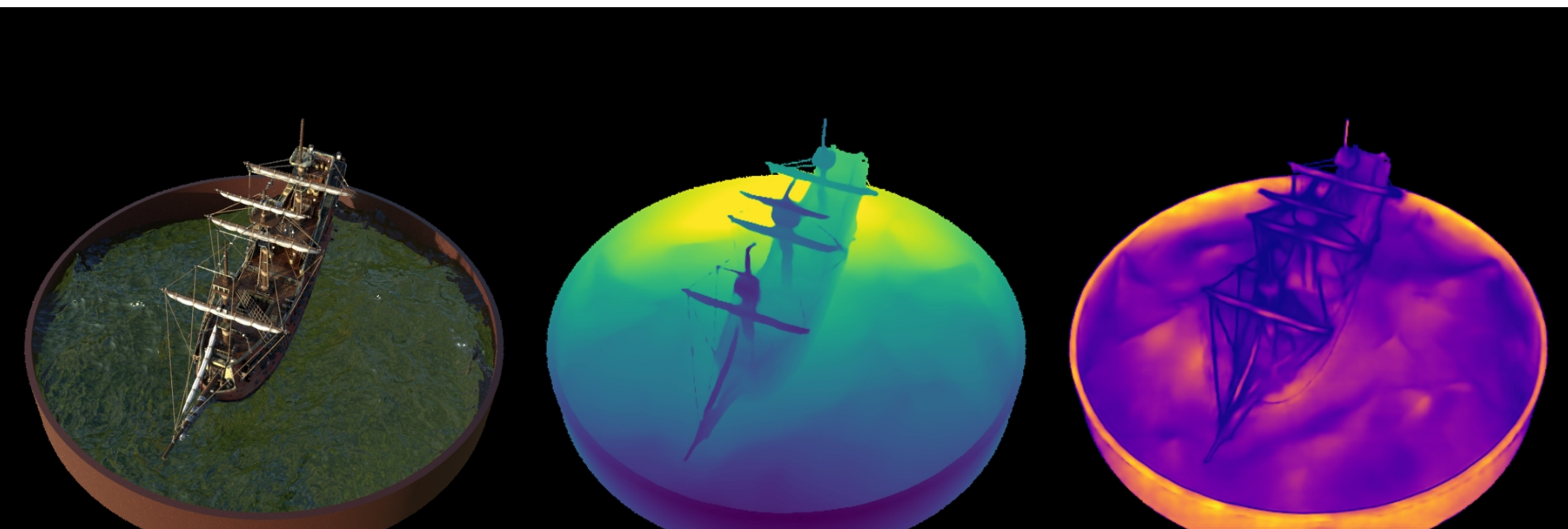
ship: VGGT | random | num_points=870000 Original | Depth (max=1.23) | Confidence (max=146.85)
