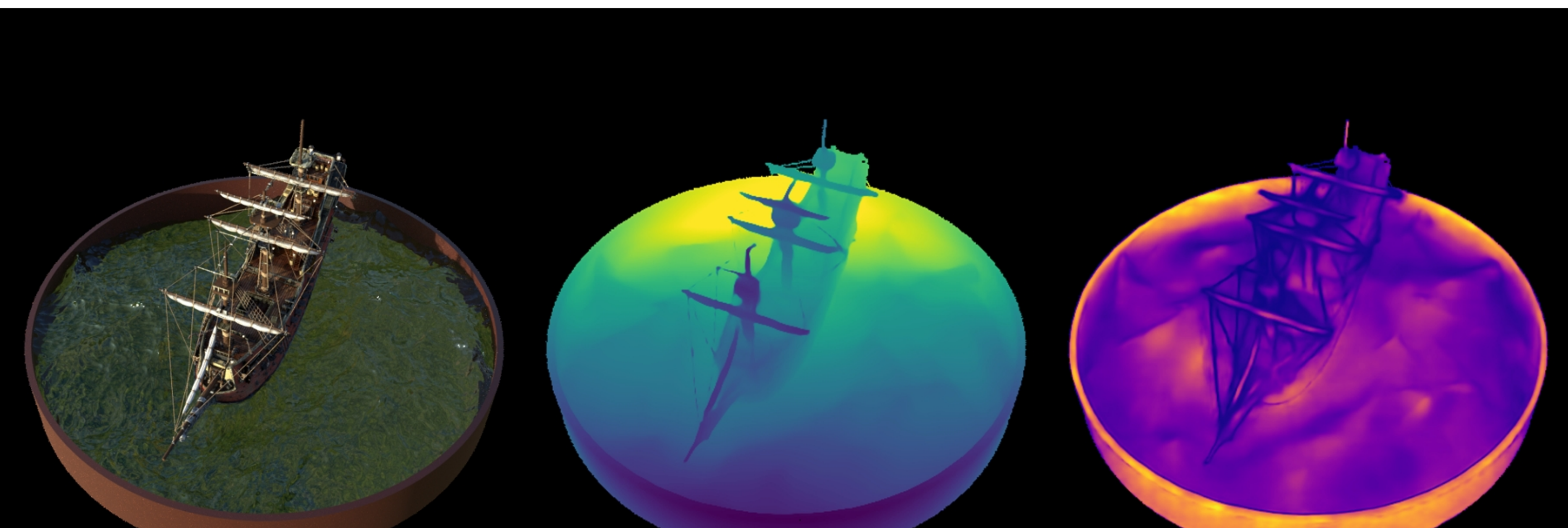
ship: VGGT | random | num_points=870 Original | Depth (max=1.23) | Confidence (max=146.85)
