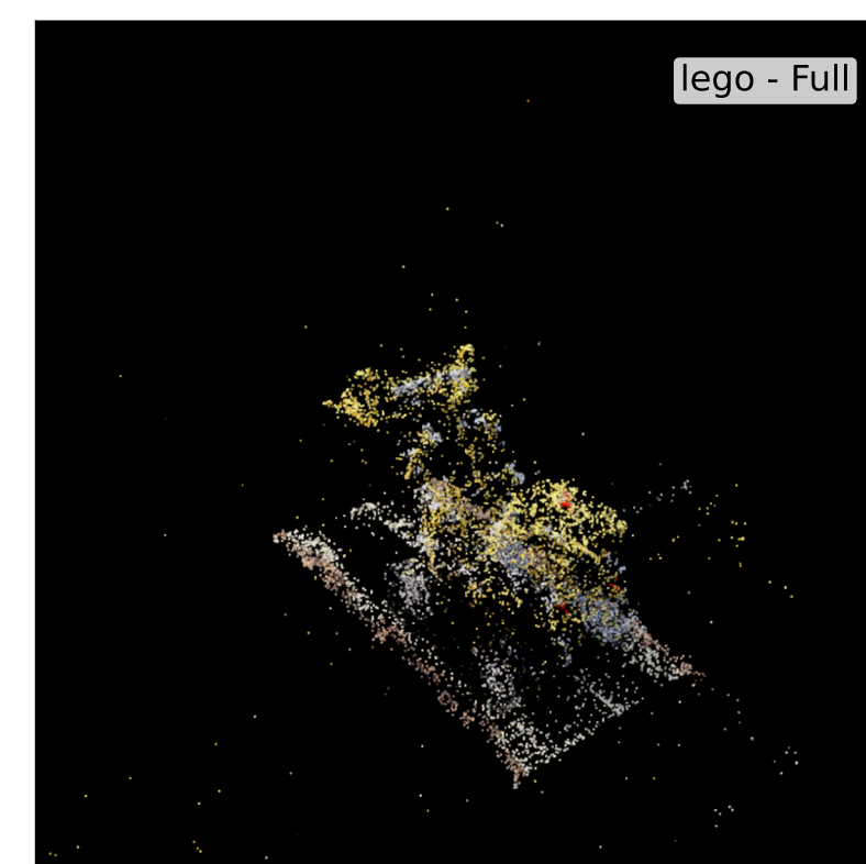
COLMAP | | num_points=10313
