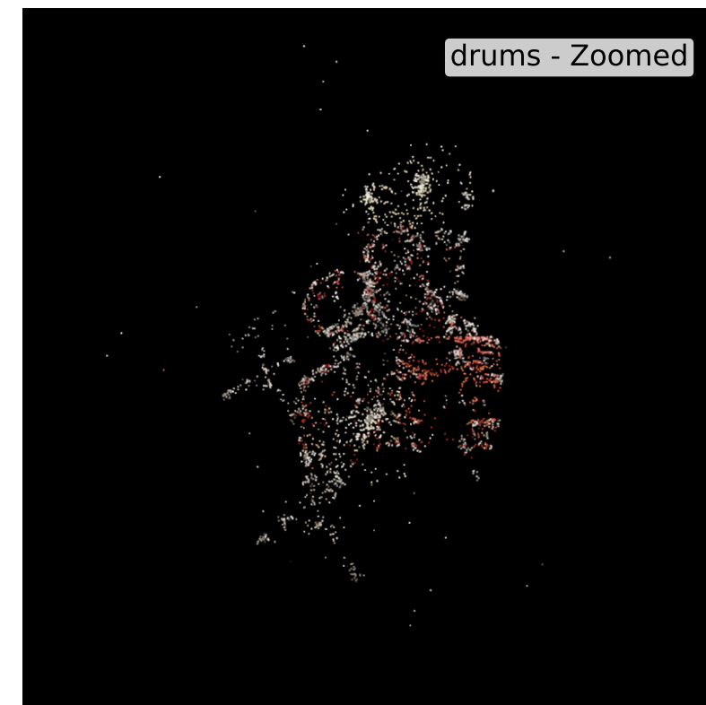
COLMAP | | num_points=3866
