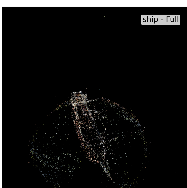
COLMAP | | num_points=5146
