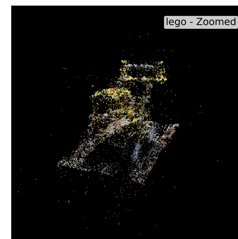
COLMAP | | num_points=10313
