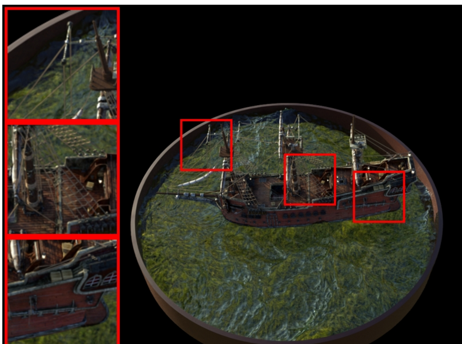
ship: VGGT | random | num_points=870000 PSNR: 29.70 | LPIPS: 0.0873 | SSIM: 0.8873
