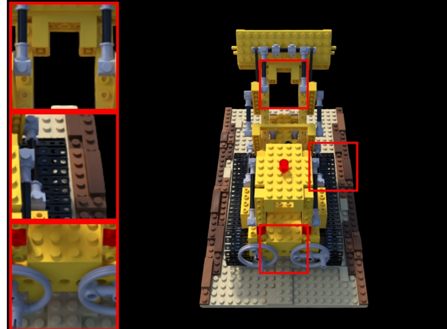
lego: VGGT | random | num_points=8700 PSNR: 33.13 | LPIPS: 0.0334 | SSIM: 0.9798
