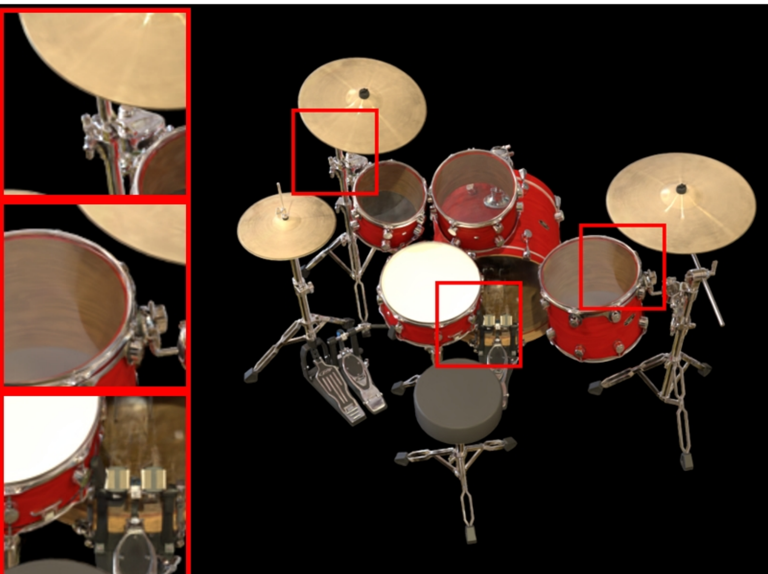
drums: VGGT | random | num_points=87000 PSNR: 25.03 | LPIPS: 0.0705 | SSIM: 0.9415
