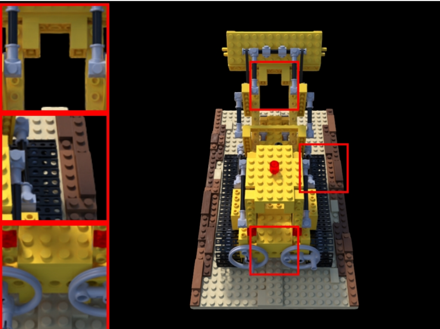
lego: VGGT | random | num_points=87000 PSNR: 33.30 | LPIPS: 0.0319 | SSIM: 0.9808
