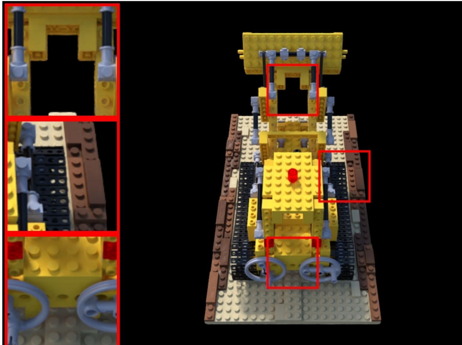
lego: VGGT | random | num_points=870000 PSNR: 33.19 | LPIPS: 0.0310 | SSIM: 0.9797
