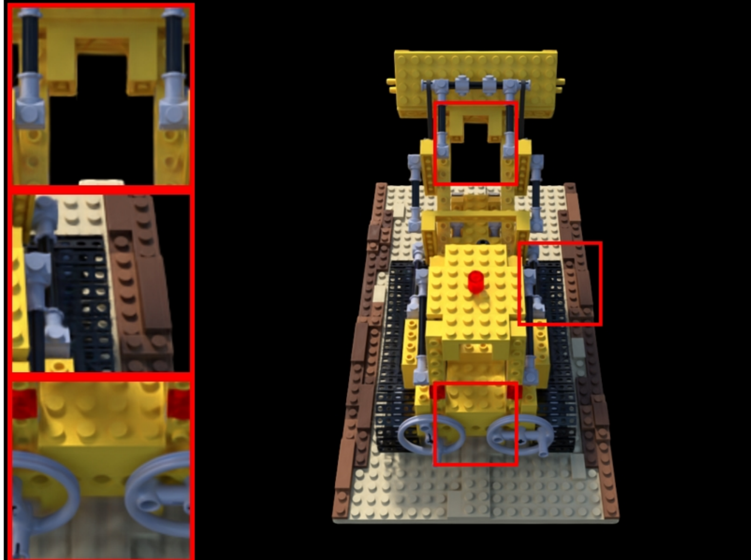
lego: VGGT | random | num_points=870 PSNR: 31.90 | LPIPS: 0.0483 | SSIM: 0.9696
