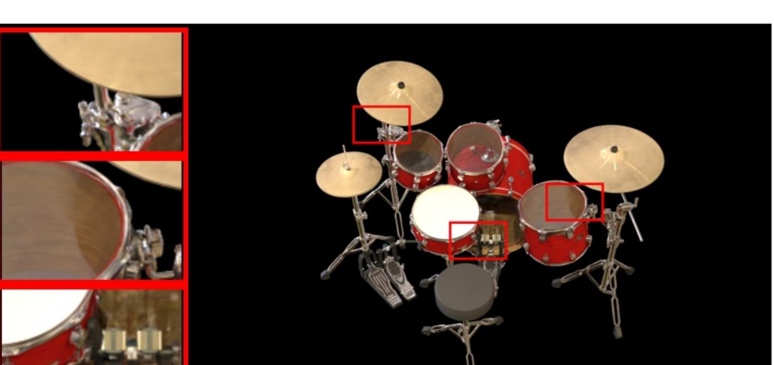
drums: VGGT | confidence | num_points=87000 PSNR: 25.04 | LPIPS: 0.0708 | SSIM: 0.9417
