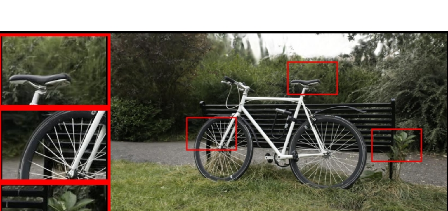
bicycle: VGGT | random | num_points=100000 PSNR: 22.77 | LPIPS: 0.2482 | SSIM: 0.6338
