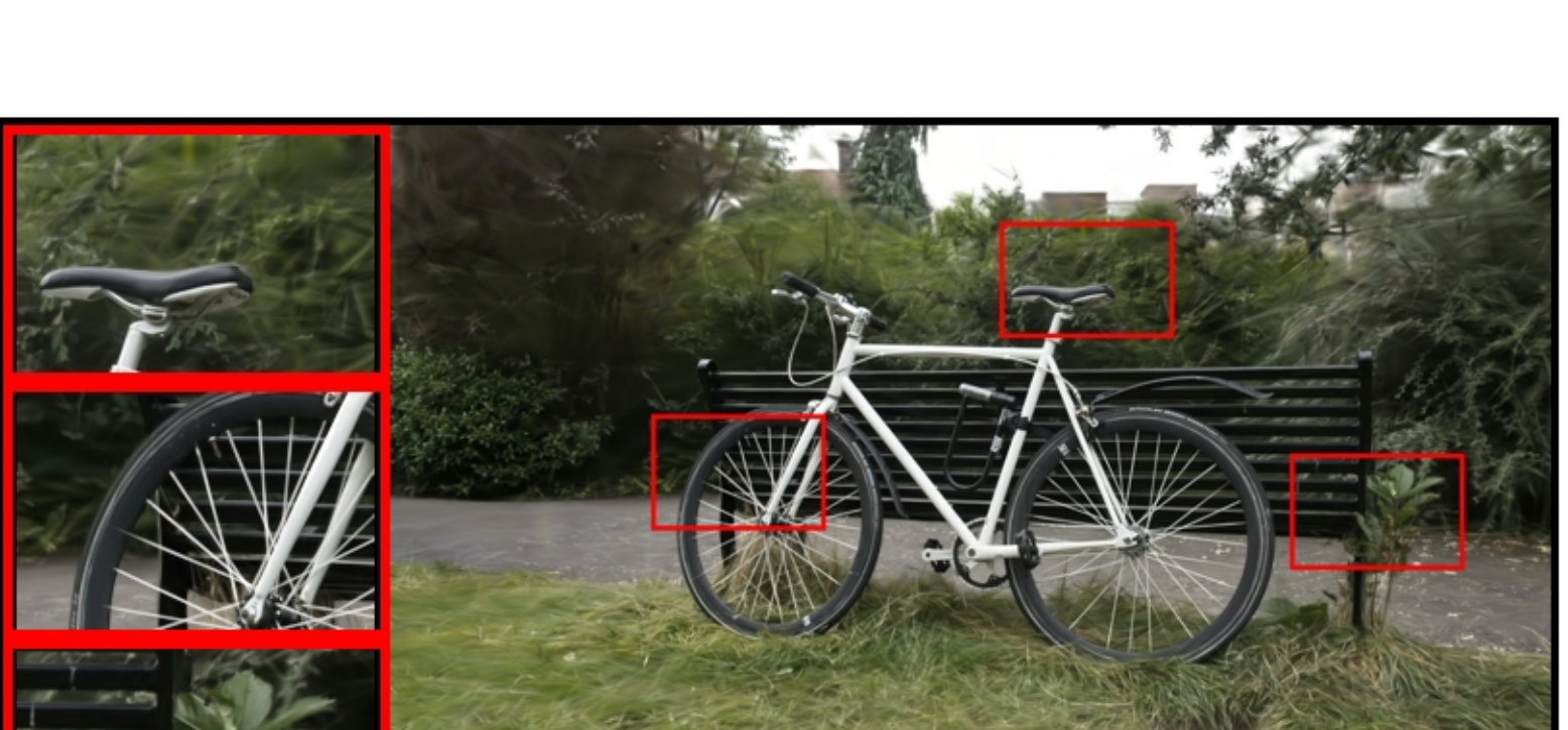
bicycle: COLMAP | num_points=17352 PSNR: 23.00 | LPIPS: 0.3495 | SSIM: 0.6104
