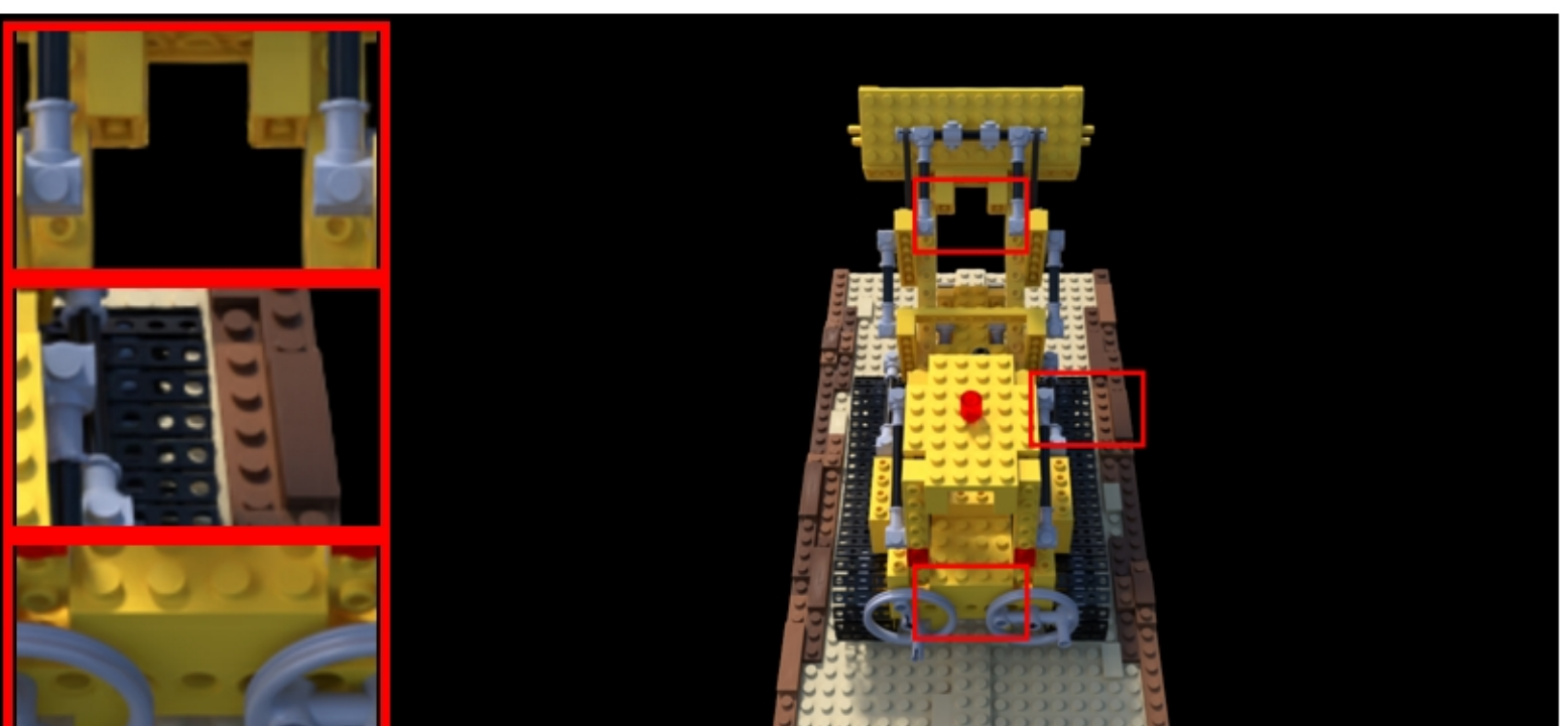
lego: COLMAP | num_points=10313 PSNR: 33.12 | LPIPS: 0.0340 | SSIM: 0.9796
