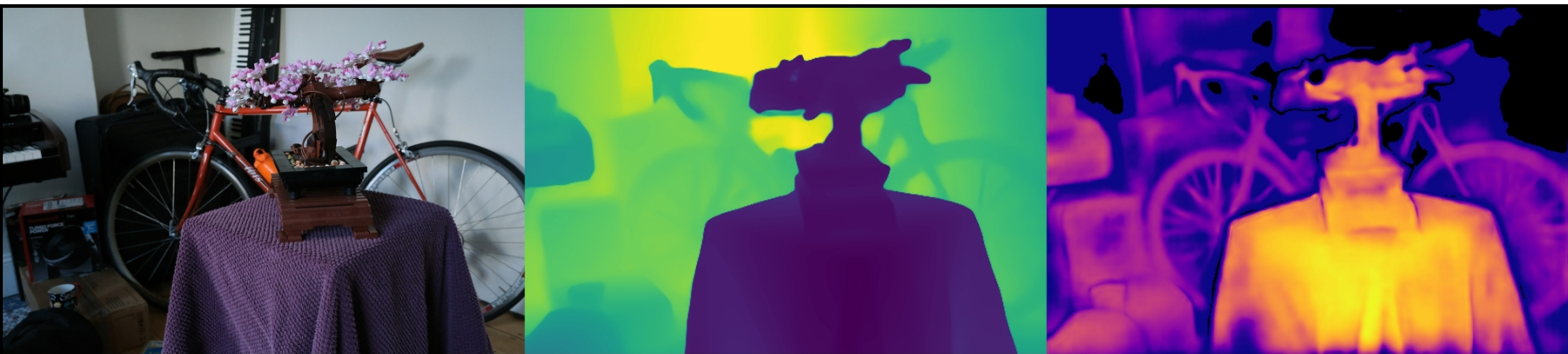
bonsai: VGGT | confidence | num_points=100000 Original | Depth (max=2.21) | Confidence (max=5.14)
