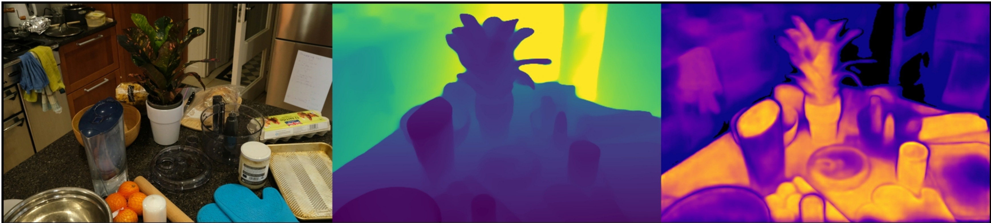
counter: VGGT | voxels | num_points=100000 Original | Depth (max=2.88) | Confidence (max=15.71)
