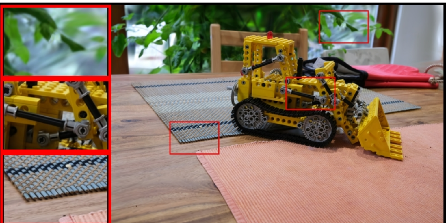
kitchen: COLMAP | num_points=92853 PSNR: 27.95 | LPIPS: 0.1216 | SSIM: 0.9019
