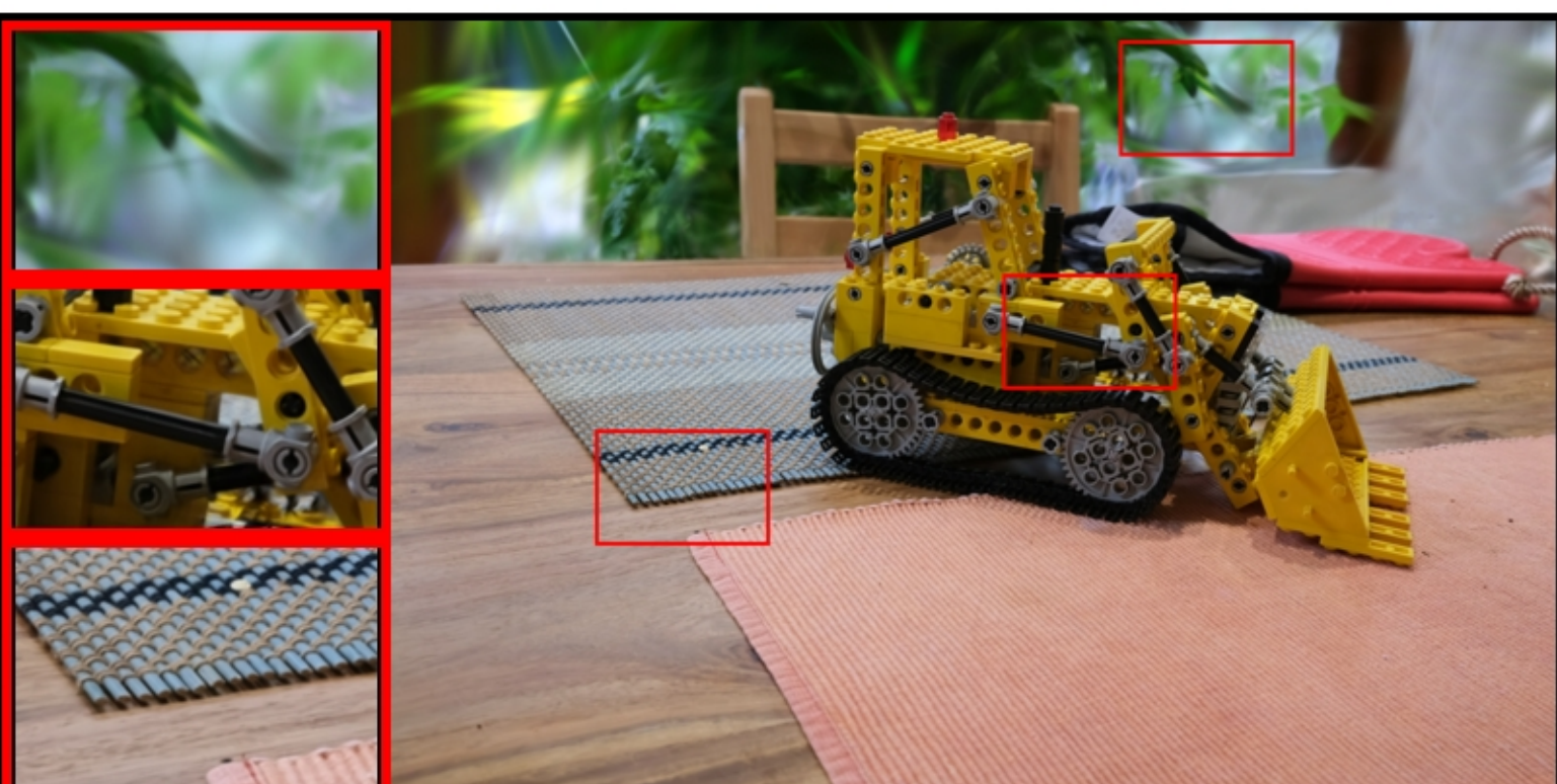
kitchen: VGGT | voxels | num_points=100000 PSNR: 25.26 | LPIPS: 0.1443 | SSIM: 0.8857
