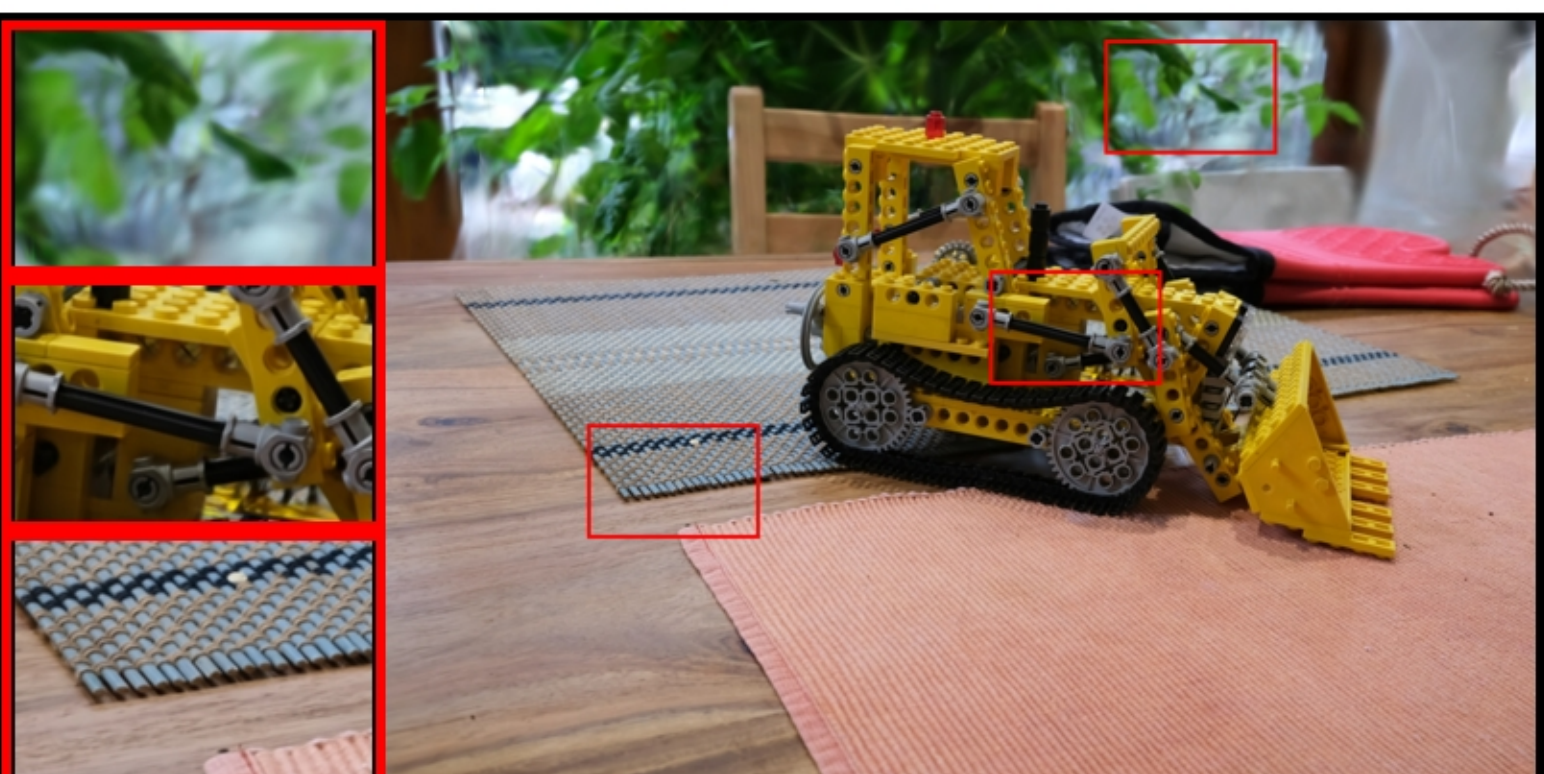
kitchen: VGGT | random | num_points=100000 PSNR: 25.89 | LPIPS: 0.1295 | SSIM: 0.8895
