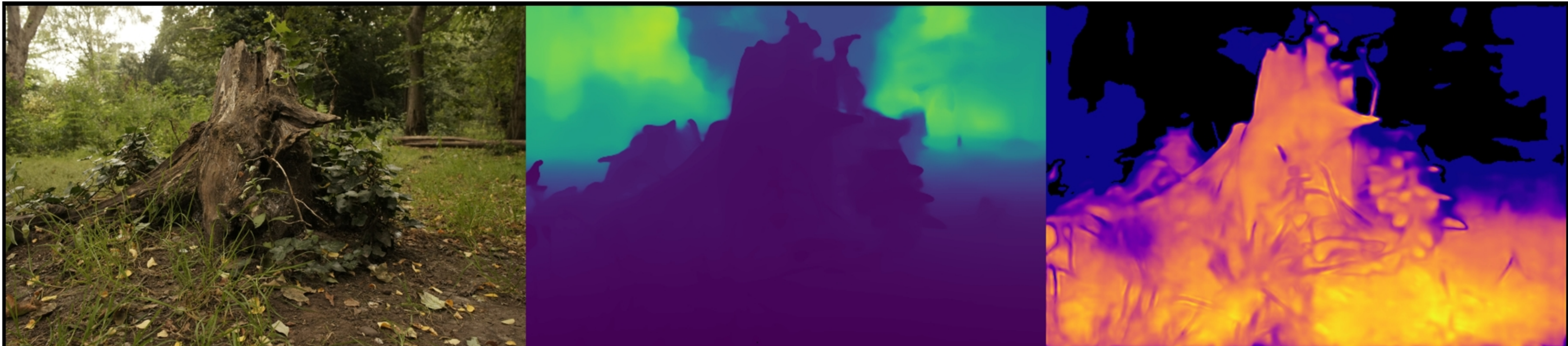
stump: VGGT | voxels | num_points=100000 Original | Depth (max=6.21) | Confidence (max=3.47)
