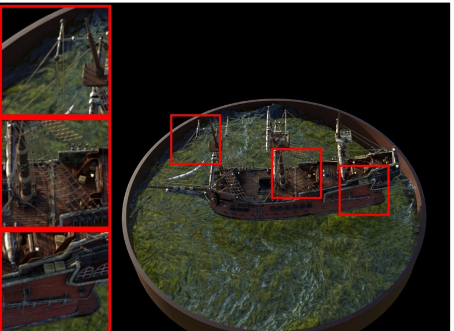
ship: VGGT | random | num_points=87000 PSNR: 29.87 | LPIPS: 0.0942 | SSIM: 0.8939
