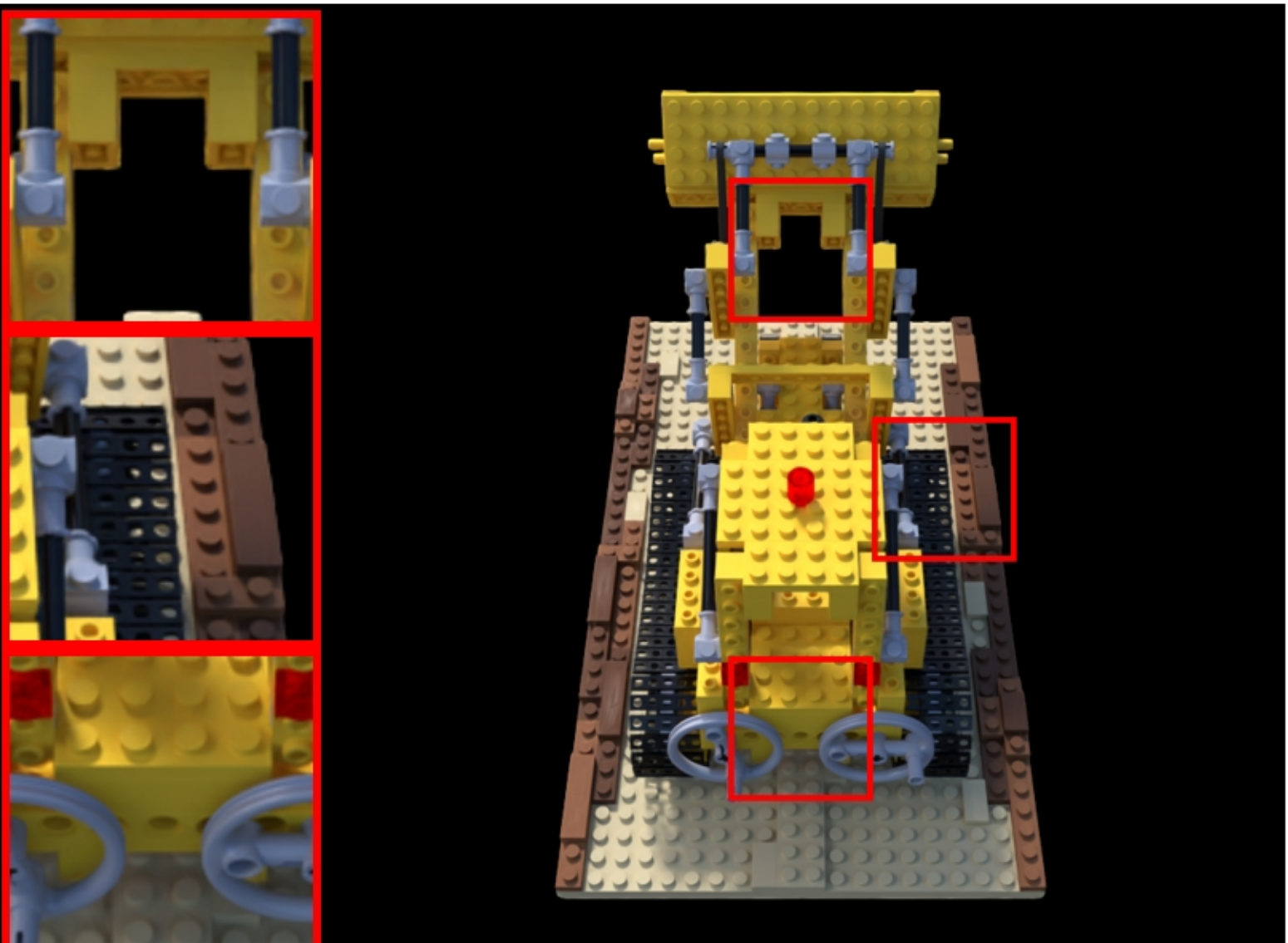
lego: COLMAP | | num_points=10313 PSNR: 33.12 | LPIPS: 0.0340 | SSIM: 0.9796
