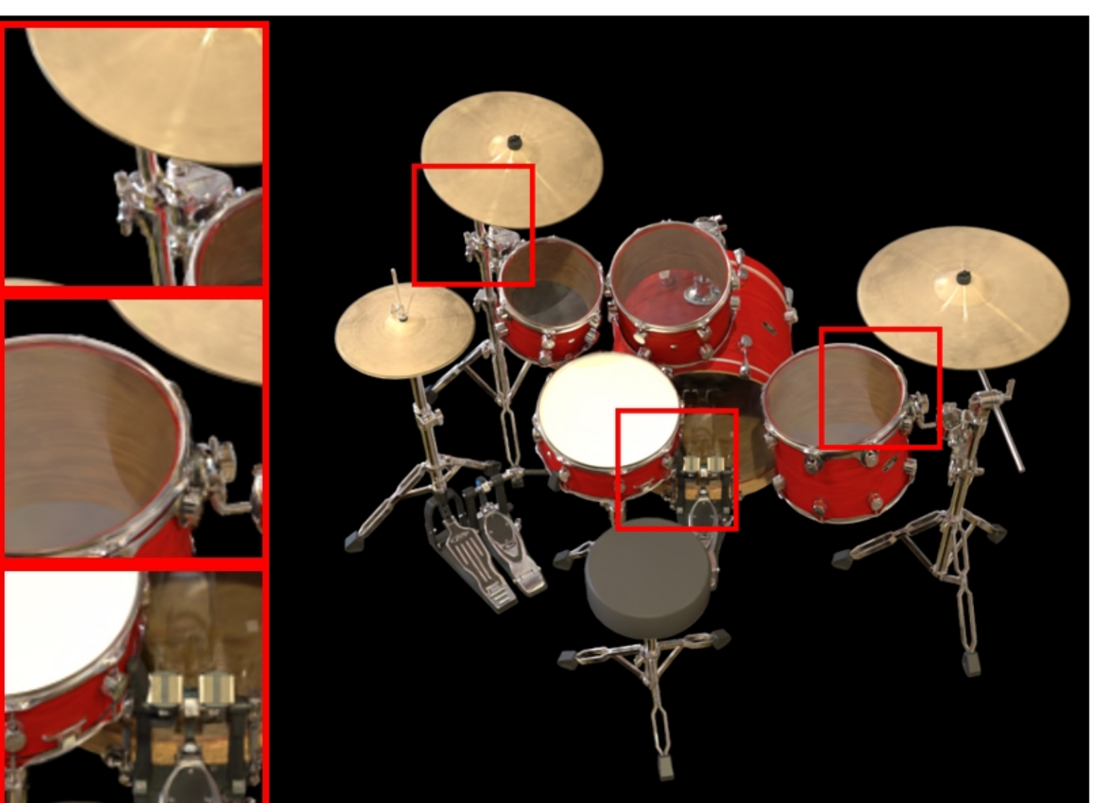
drums: VGGT | voxels | num_points=87000 PSNR: 25.07 | LPIPS: 0.0702 | SSIM: 0.9420
