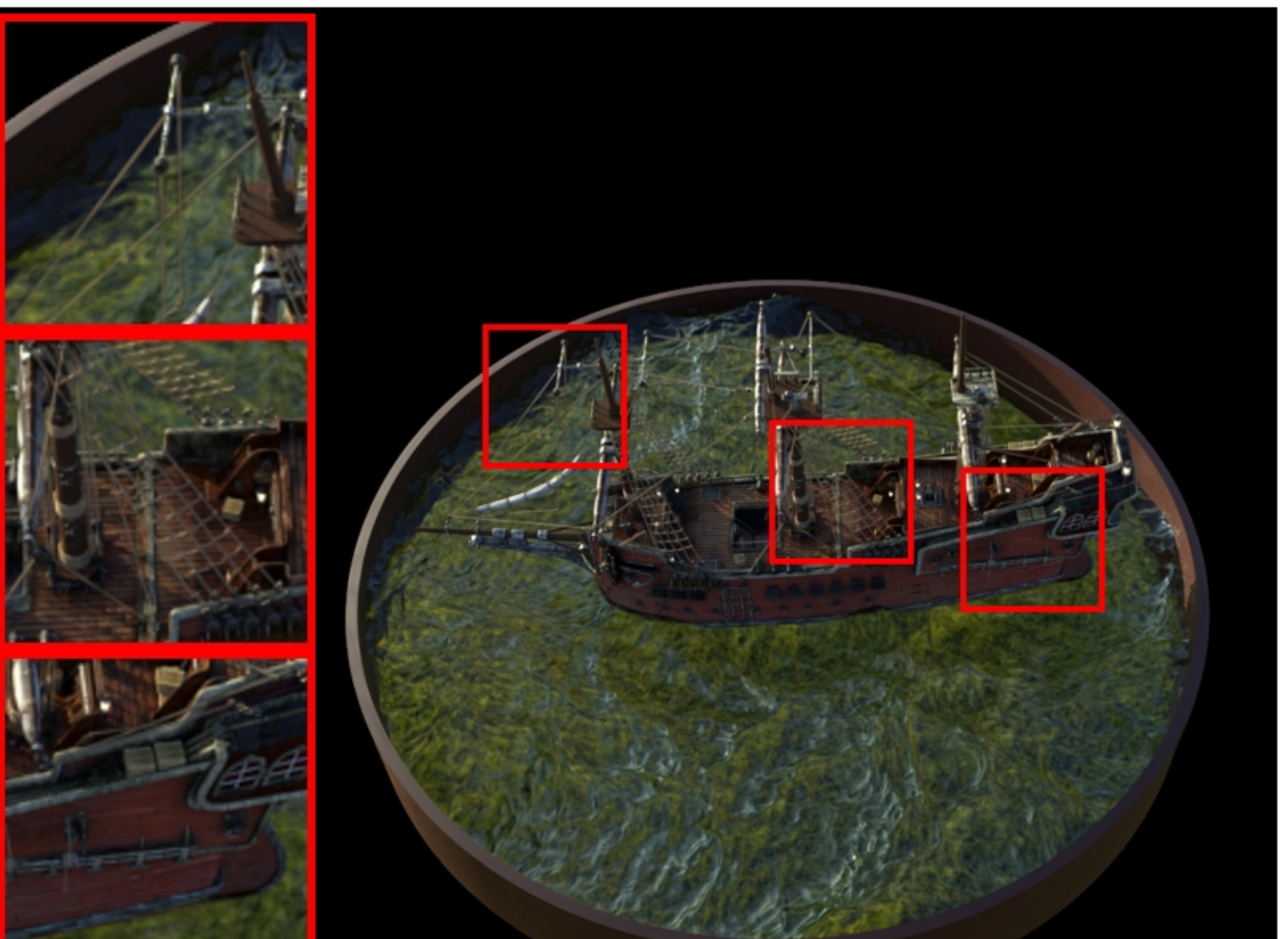
ship: VGGT | confidence | num_points=87000 PSNR: 29.86 | LPIPS: 0.0926 | SSIM: 0.8938
