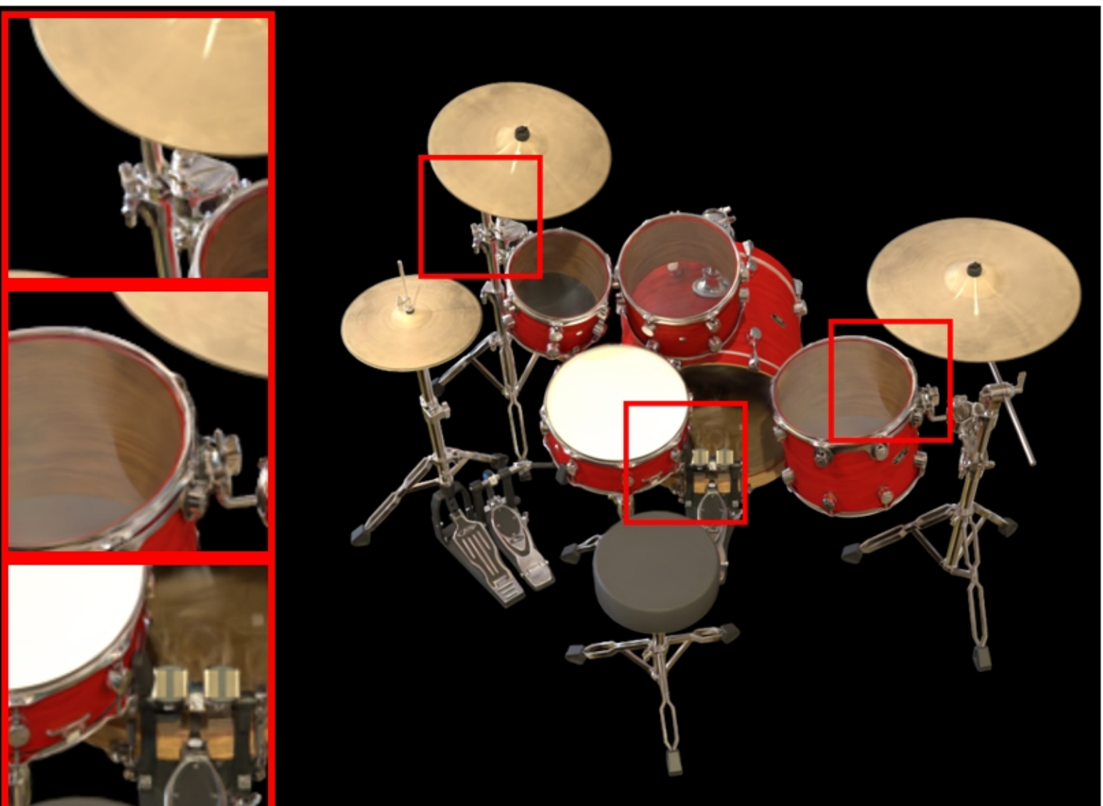
drums: COLMAP | | num_points=3866 PSNR: 24.16 | LPIPS: 0.0843 | SSIM: 0.9296
