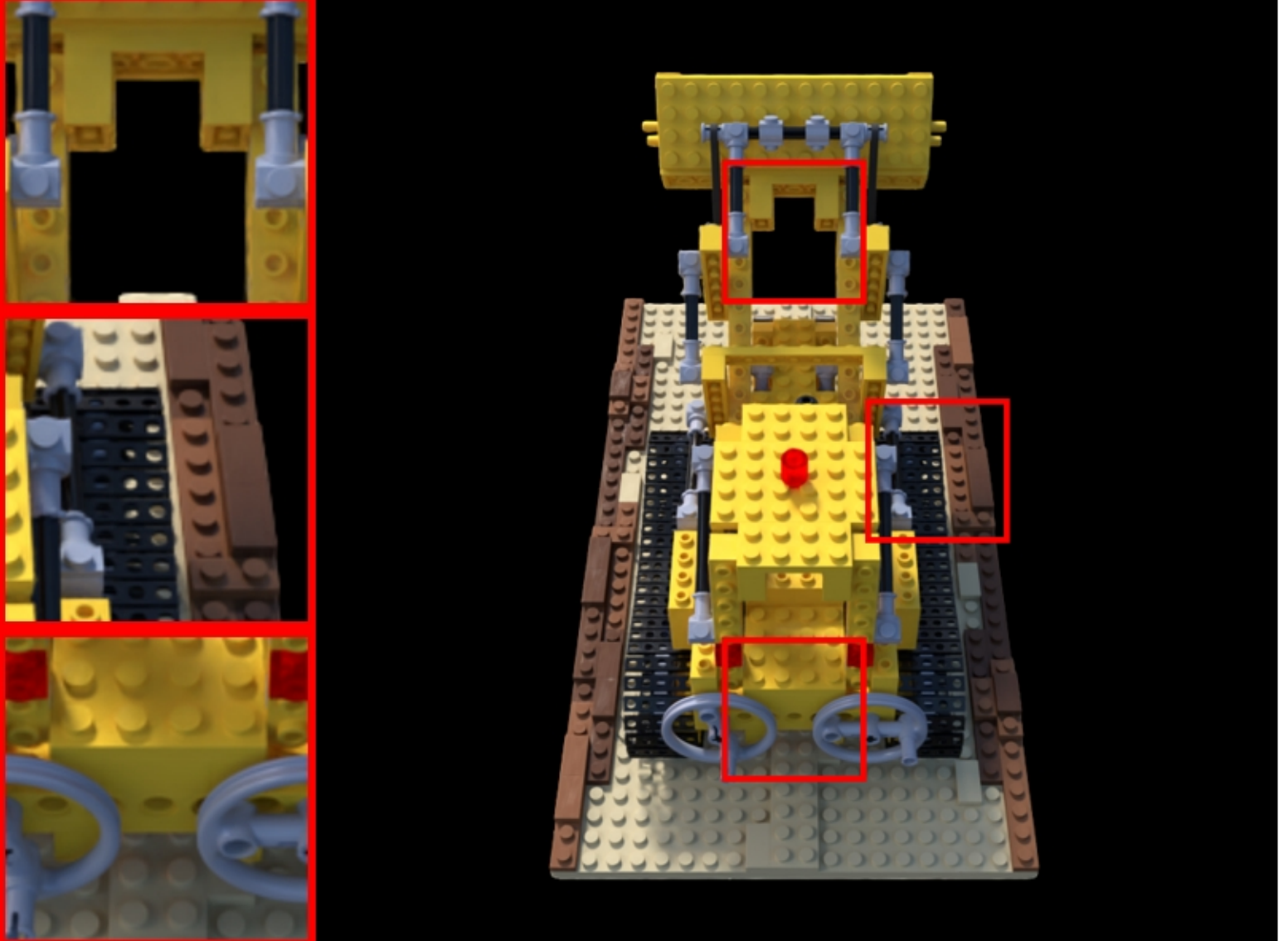
lego: VGGT | voxels | num_points=87000 PSNR: 33.30 | LPIPS: 0.0318 | SSIM: 0.9808
