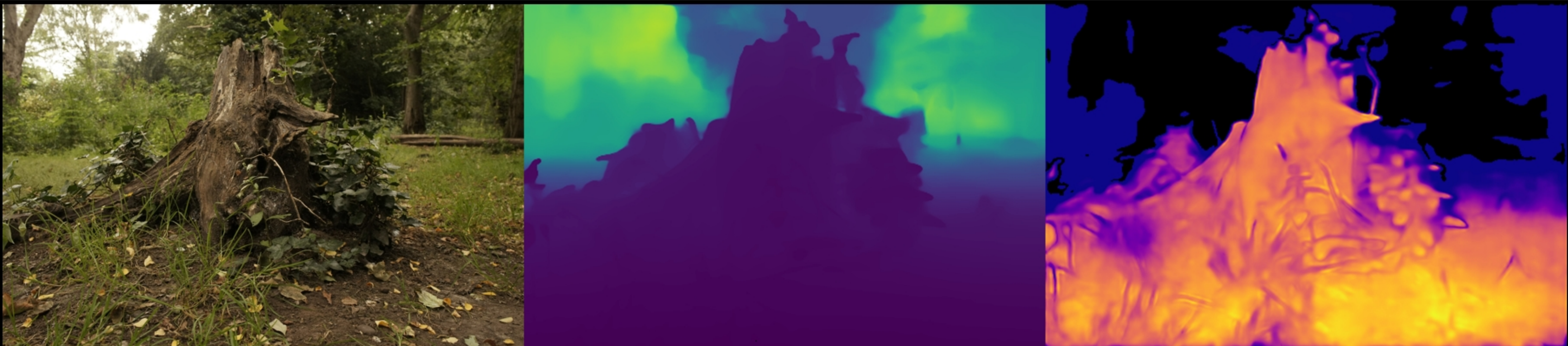
stump: VGGT | imagefps | num_points=100000 Original | Depth (max=6.21) | Confidence (max=3.47)
