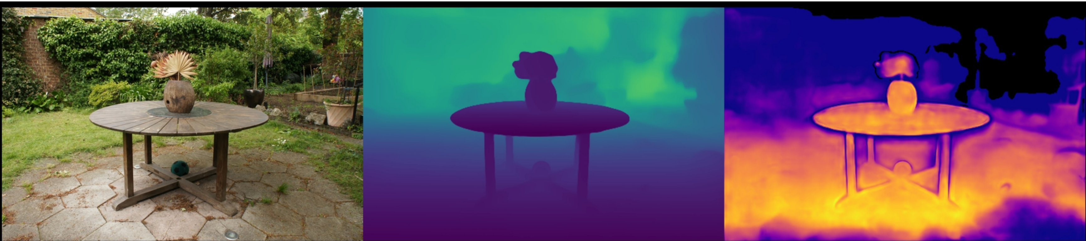
garden: VGGT | voxels | num_points=100000 Original | Depth (max=2.46) | Confidence (max=6.23)
