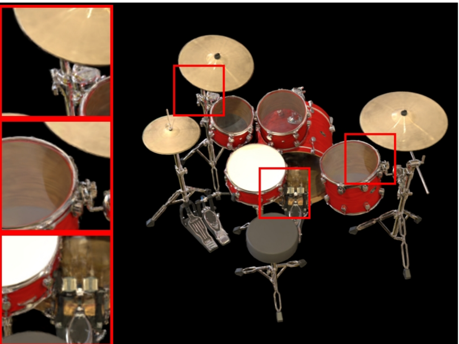
drums: VGGT | confidence | num_points=87000 PSNR: 19.68 | LPIPS: 0.1069 | SSIM: 0.8363
