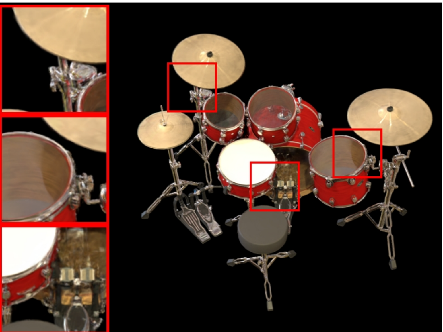
drums: VGGT | imagefps | num_points=87000 PSNR: 19.64 | LPIPS: 0.1072 | SSIM: 0.8353
