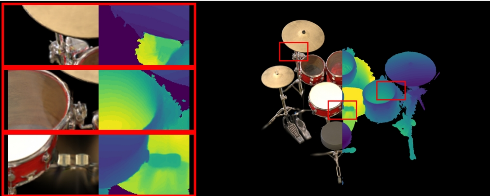
drums: VGGT | Standard Shifted | full PSNR: 20.27 | LPIPS: 0.1506 | SSIM: 0.8579
