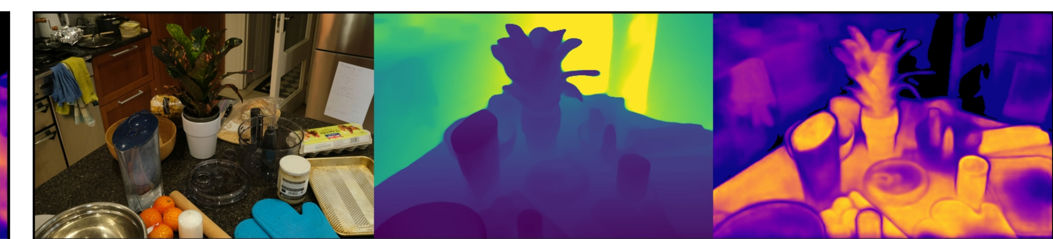
counter: VGGT | | full Original | Depth (max=2.88) | Confidence (max=15.71)
