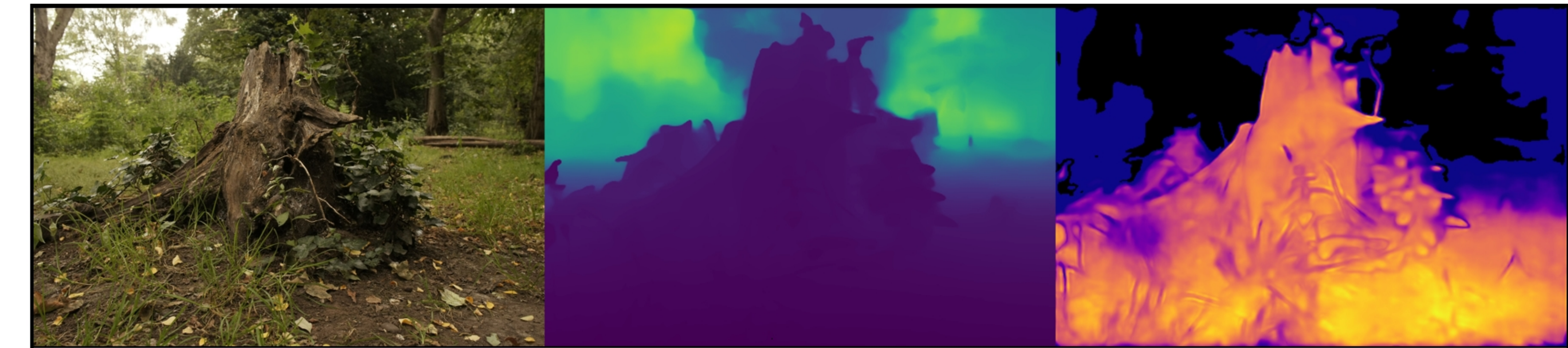
stump: VGGT | | full Original | Depth (max=6.21) | Confidence (max=3.47)
