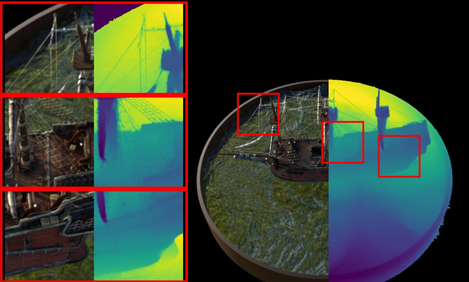
ship: VGGT | full PSNR: 23.49 | LPIPS: 0.1317 | SSIM: 0.7647
