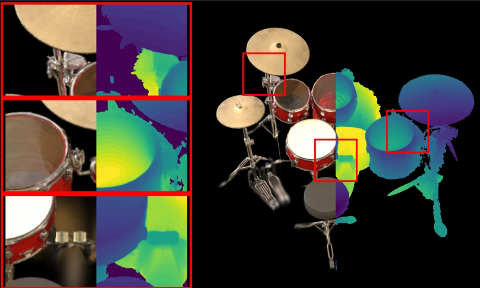
drums: VGGT | Standard Shifted | full PSNR: 20.37 | LPIPS: 0.1506 | SSIM: 0.8585
