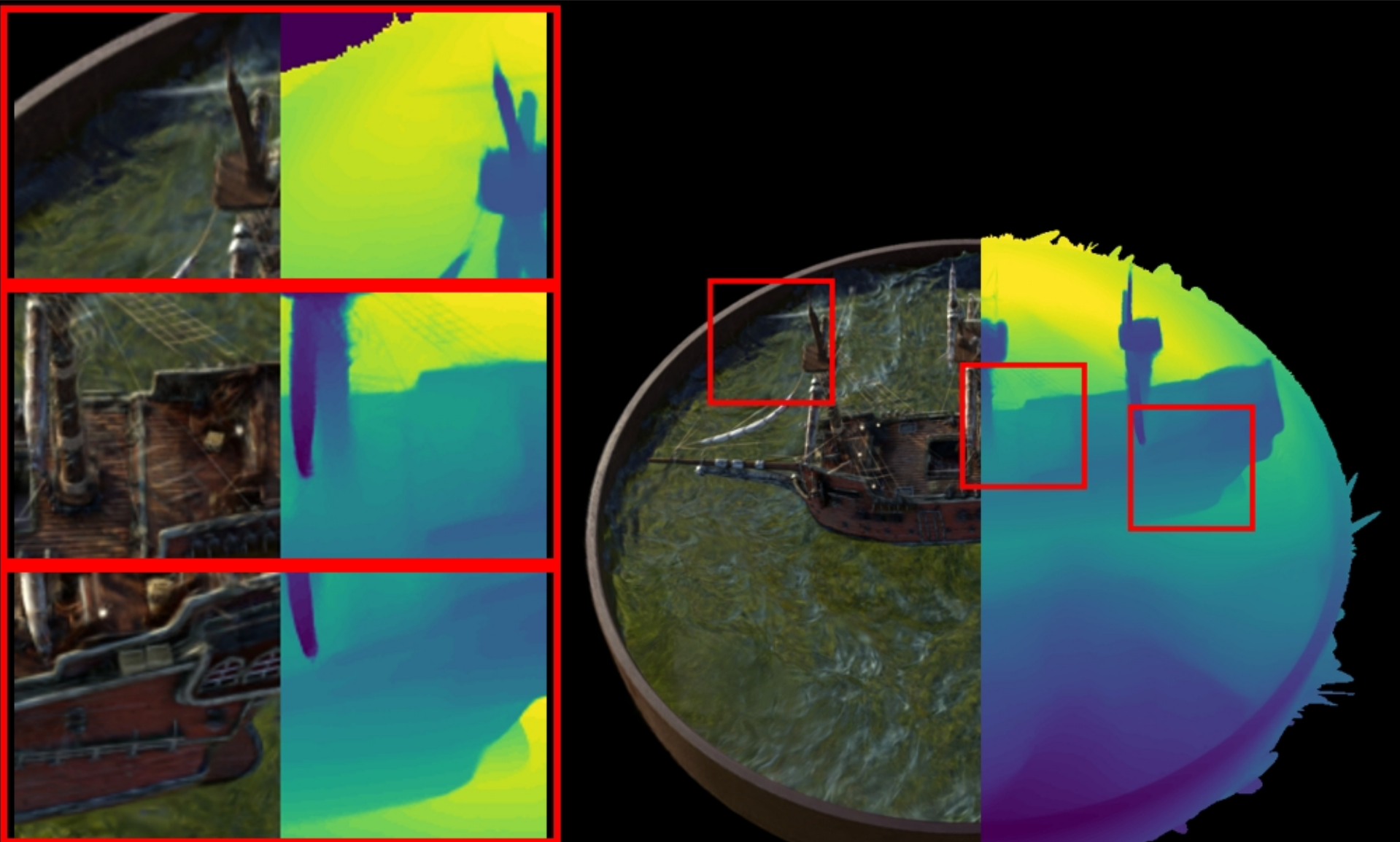
ship: VGGT | Standard | full PSNR: 23.75 | LPIPS: 0.1742 | SSIM: 0.7740
