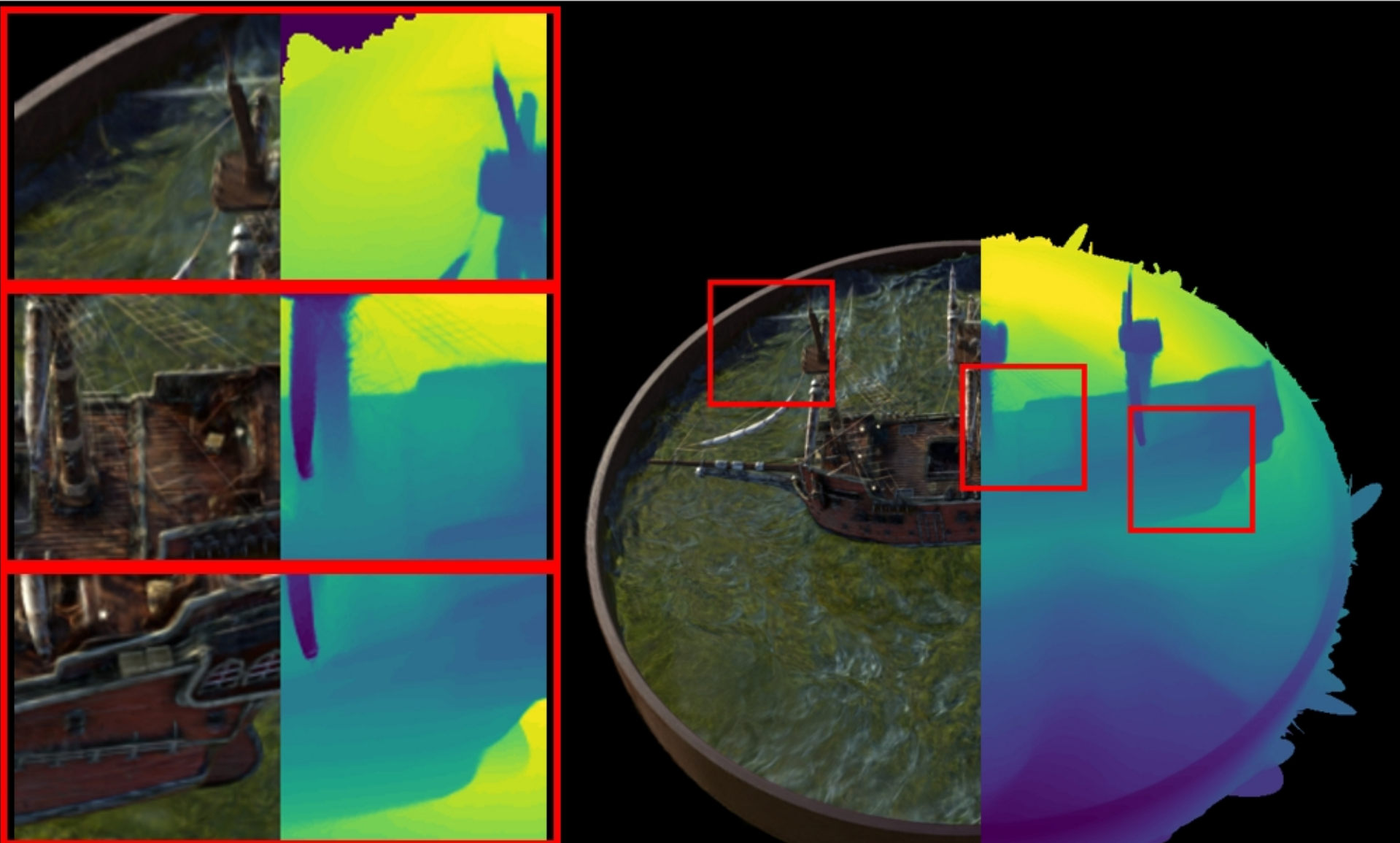
ship: VGGT | Standard Shifted | full PSNR: 23.76 | LPIPS: 0.1730 | SSIM: 0.7743
