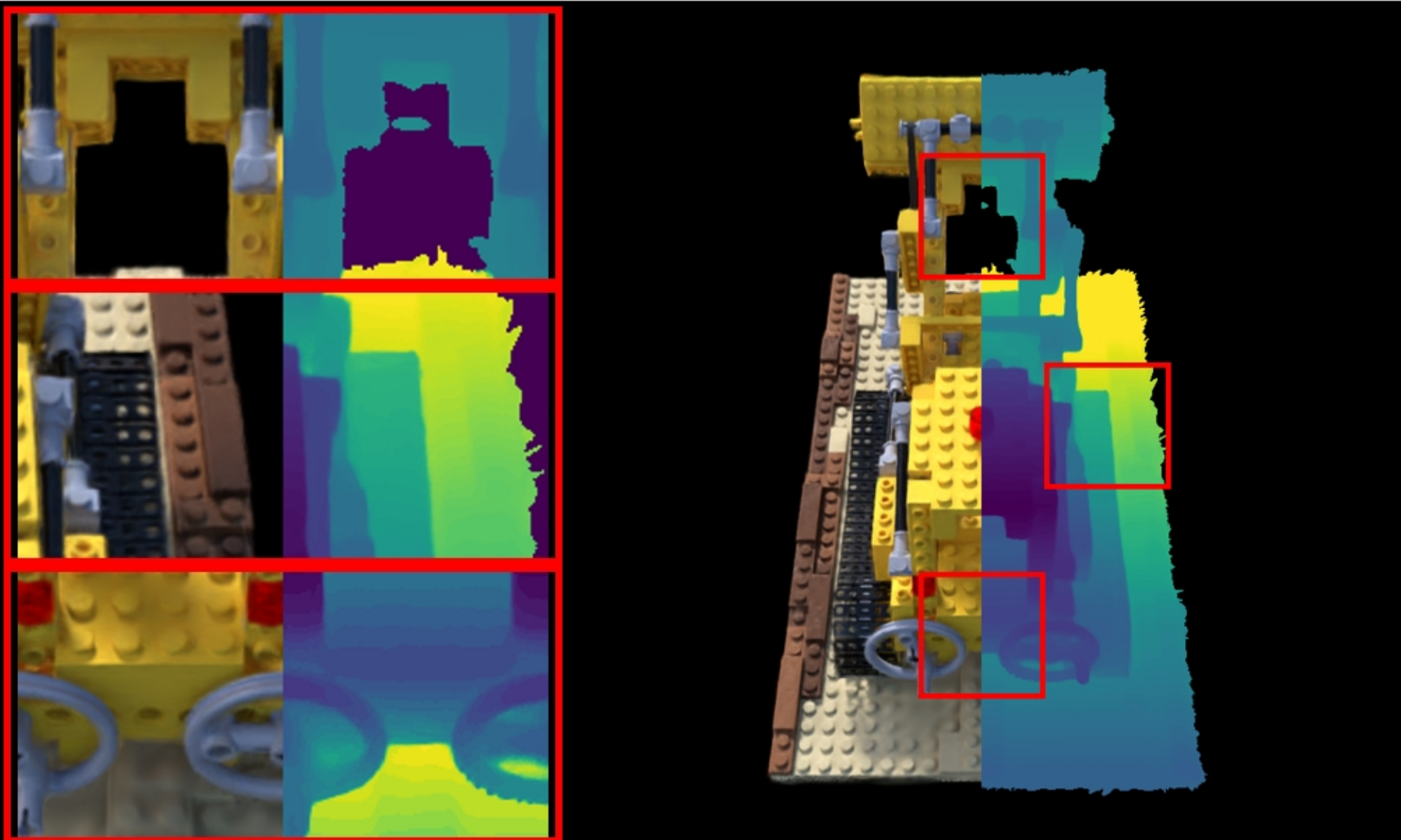
lego: VGGT | Standard Shifted | full PSNR: 23.53 | LPIPS: 0.0941 | SSIM: 0.8458
