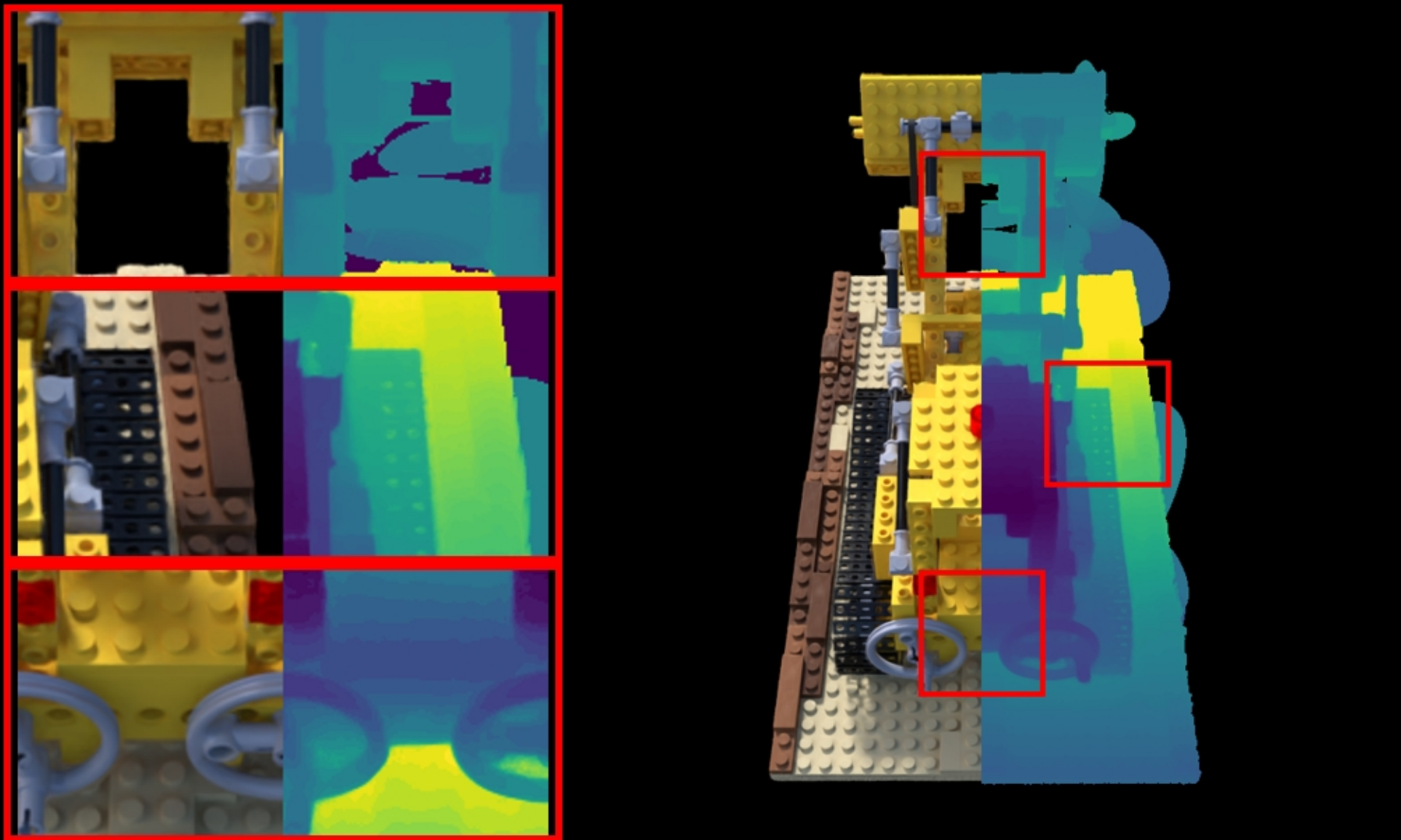
lego: VGGT | full PSNR: 21.97 | LPIPS: 0.0697 | SSIM: 0.8123
