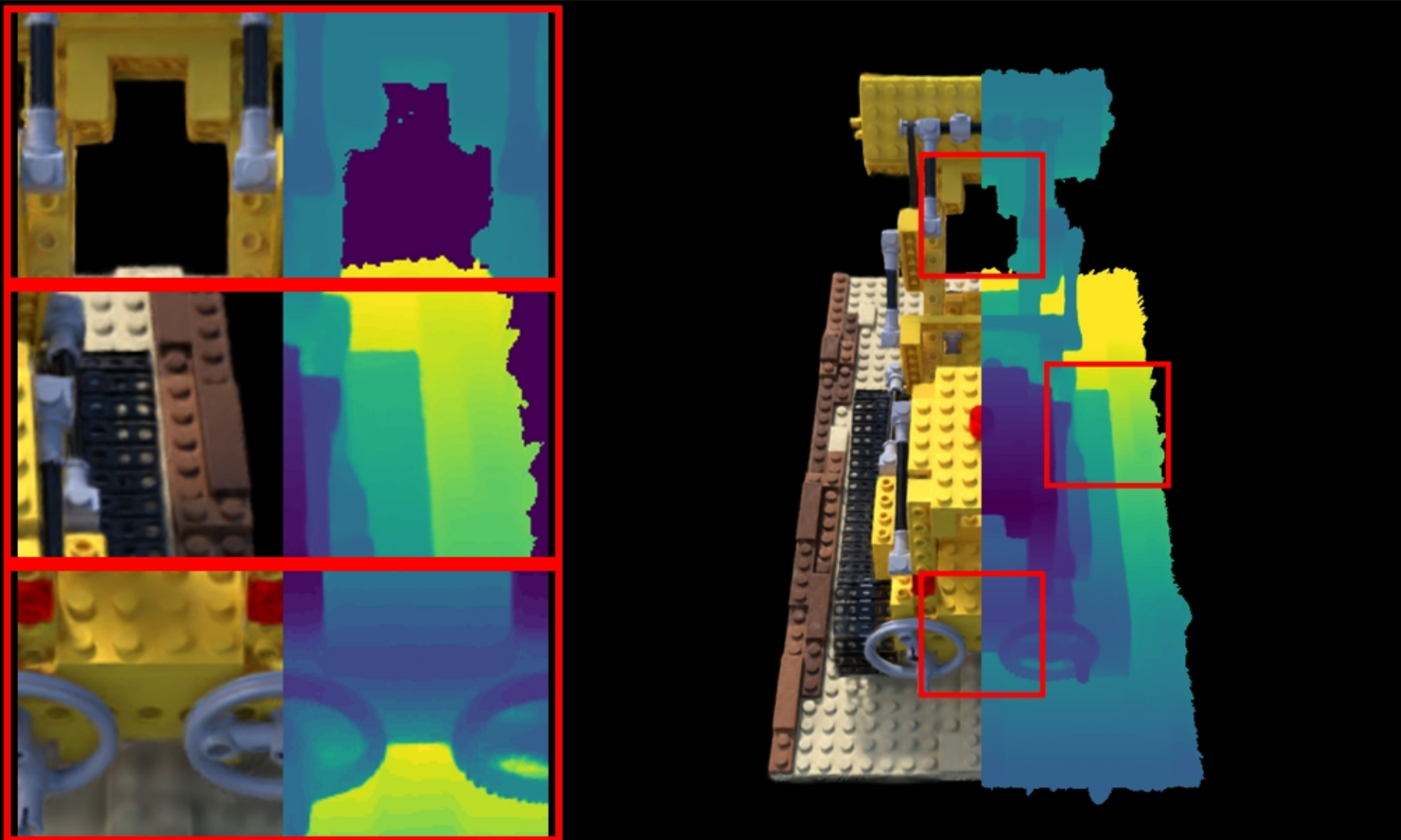
lego: VGGT | Standard | full PSNR: 23.51 | LPIPS: 0.0945 | SSIM: 0.8450
