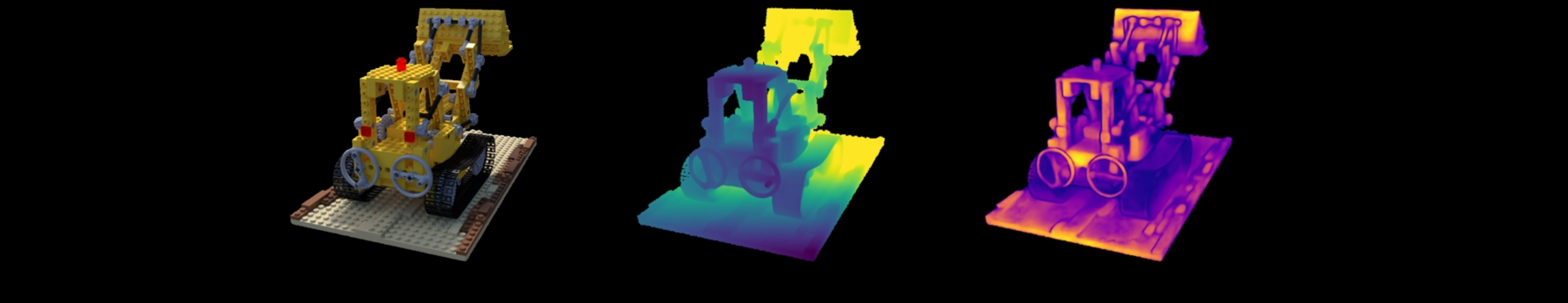
lego: VGGT | depth_lambda=0.0 Original | Depth (max=1.28) | Confidence (max=155.74)
