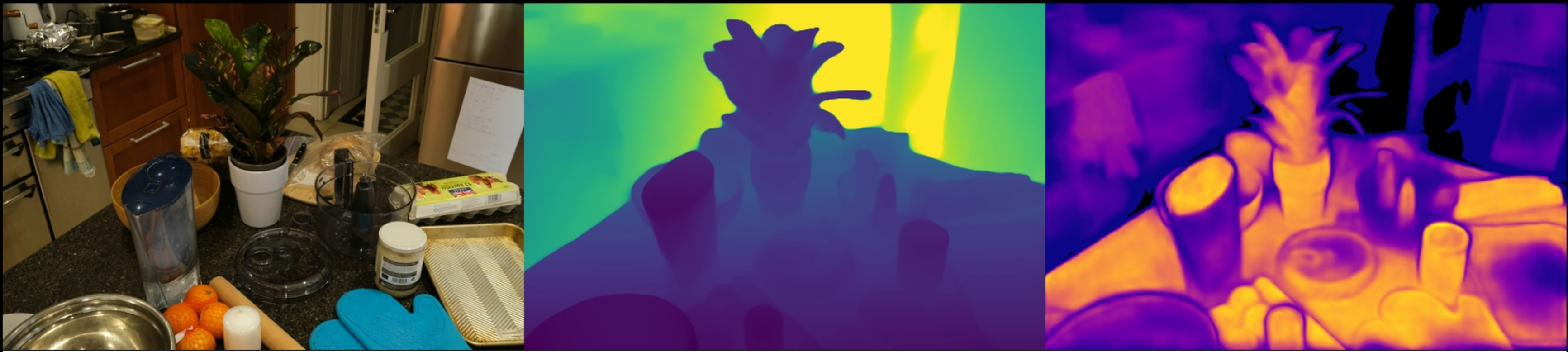
counter: VGGT | depth_lambda=0.0 Original | Depth (max=2.88) | Confidence (max=15.71)
