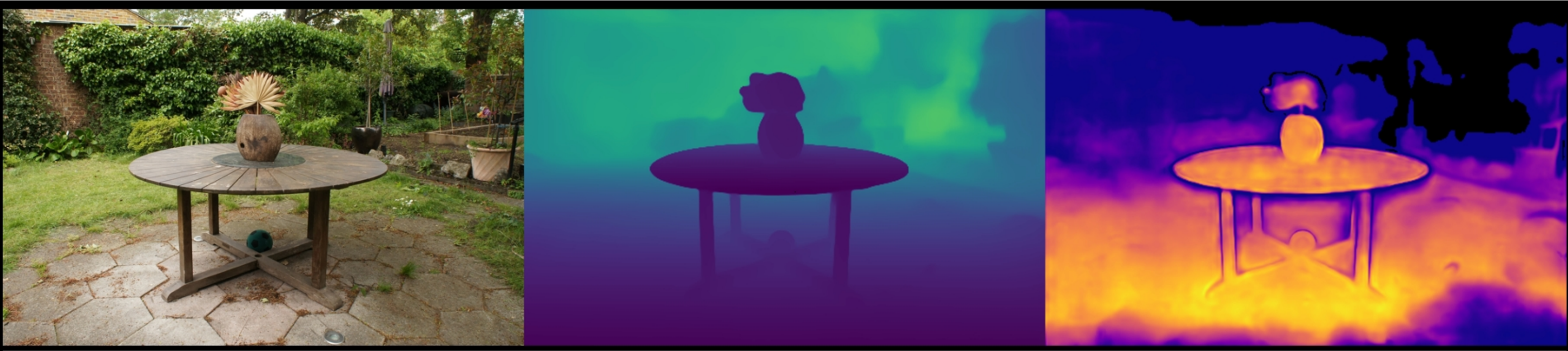
garden: VGGT | depth_lambda=0.0 Original | Depth (max=2.46) | Confidence (max=6.23)
