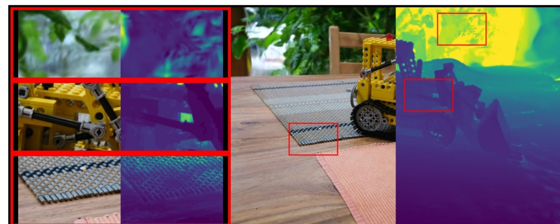
kitchen: VGGT | depth_lambda=0.1 PSNR: 19.93 | LPIPS: 0.1770 | SSIM: 0.4148
