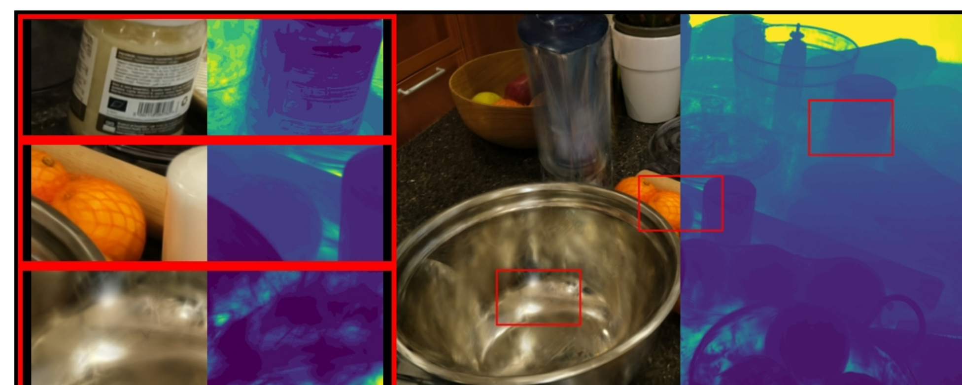
counter: VGGT | depth_lambda=0.1 PSNR: 20.87 | LPIPS: 0.2330 | SSIM: 0.6441
