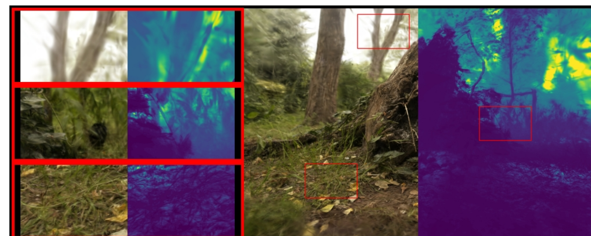
stump: VGGT | depth_lambda=1.0 PSNR: 18.34 | LPIPS: 0.4929 | SSIM: 0.3985
