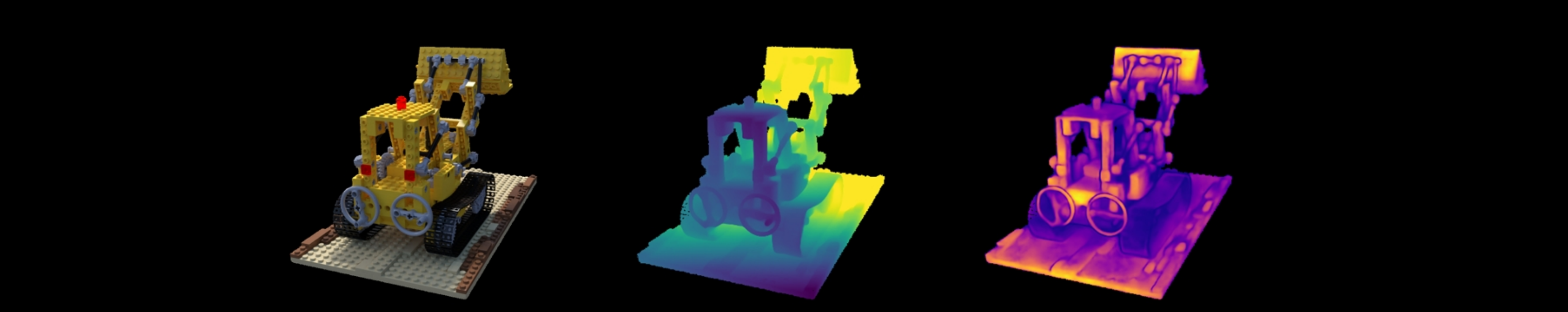
lego: VGGT | Original | Depth (max=1.28) | Confidence (max=155.74)
