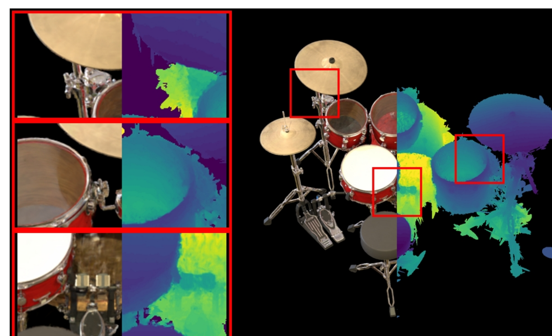
drums: VGGT | points PSNR: 20.91 | LPIPS: 0.0822 | SSIM: 0.8685
