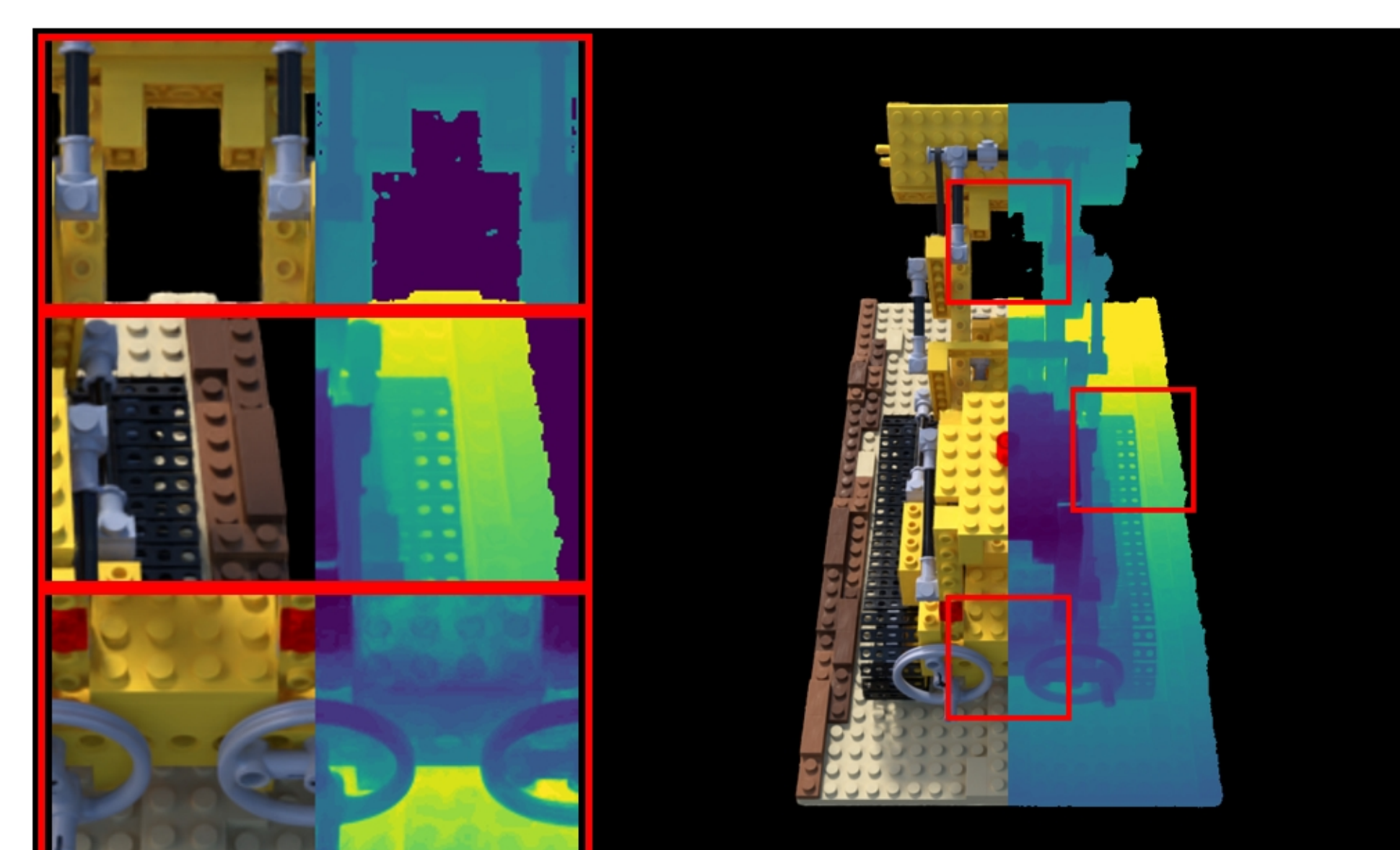
lego: VGGT | closer PSNR: 20.37 | LPIPS: 0.0786 | SSIM: 0.7747
