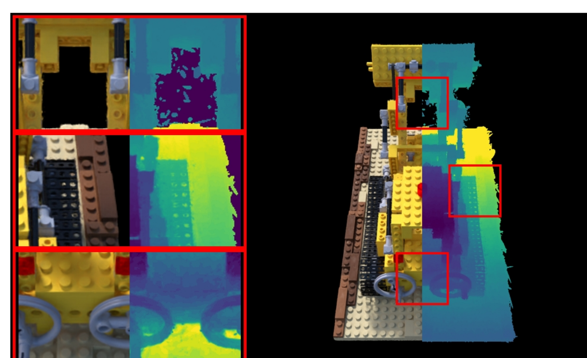
lego: VGGT | points PSNR: 21.99 | LPIPS: 0.0653 | SSIM: 0.8123
