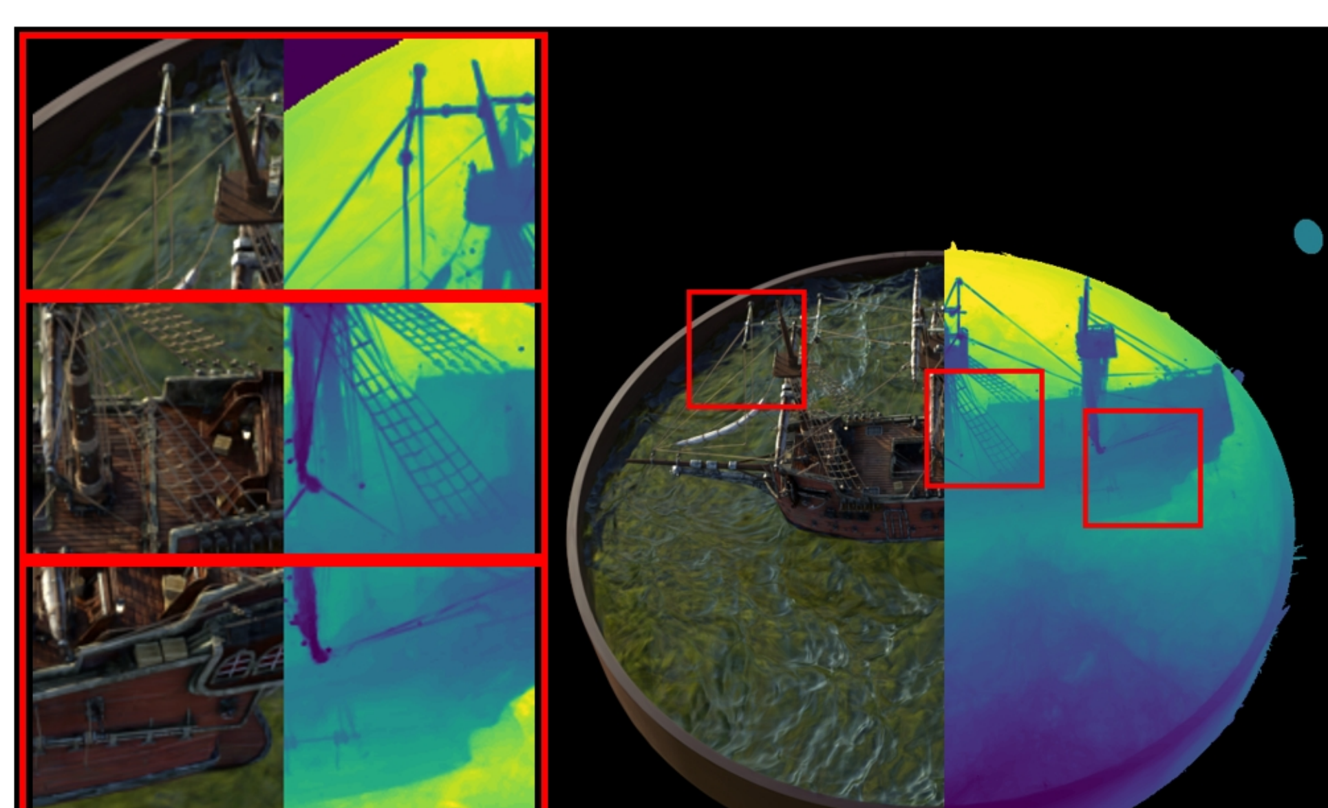
ship: COLMAP | points PSNR: 22.68 | LPIPS: 0.1487 | SSIM: 0.7591
