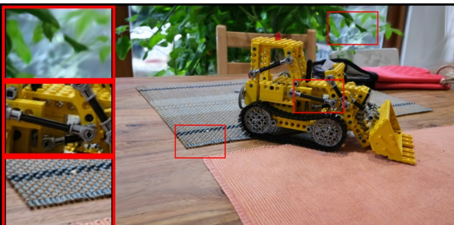
kitchen: VGGT | GT Intrinsic | GT Points PSNR: 20.27 | LPIPS: 0.2375 | SSIM: 0.4774
