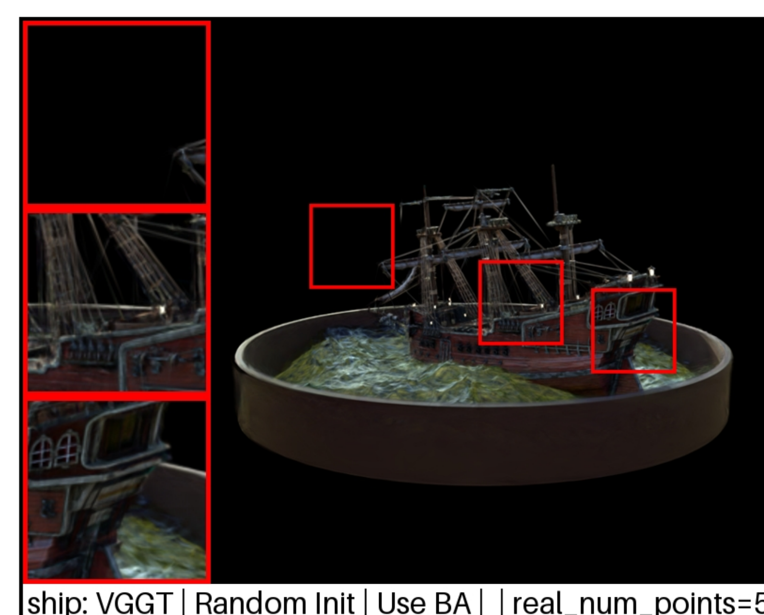
ship: VGGT | Random Init | Use BA | | real_num_points=5 PSNR: 19.13 | LPIPS: 0.2774 | SSIM: 0.6810
