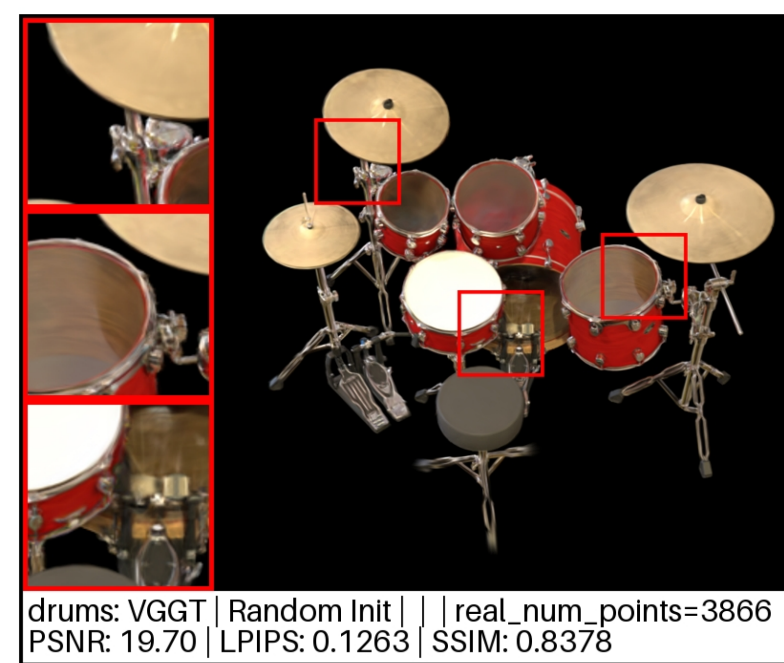
drums: VGGT | Random Init | | real_num_points=3866 PSNR: 19.70 | LPIPS: 0.1263 | SSIM: 0.8378
