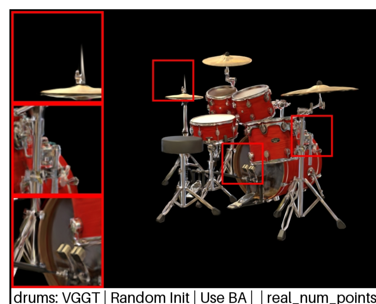
drums: VGGT | Random Init | Use BA | | real_num_points=5 PSNR: 18.61 | LPIPS: 0.1225 | SSIM: 0.8162
