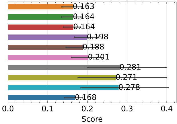
SSIM ↑ - indoor
