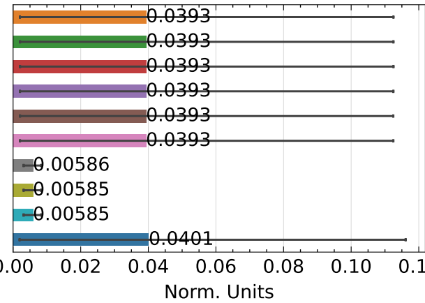
PSNR ↑ - synthetic
