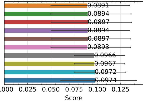
SSIM ↑ - synthetic
