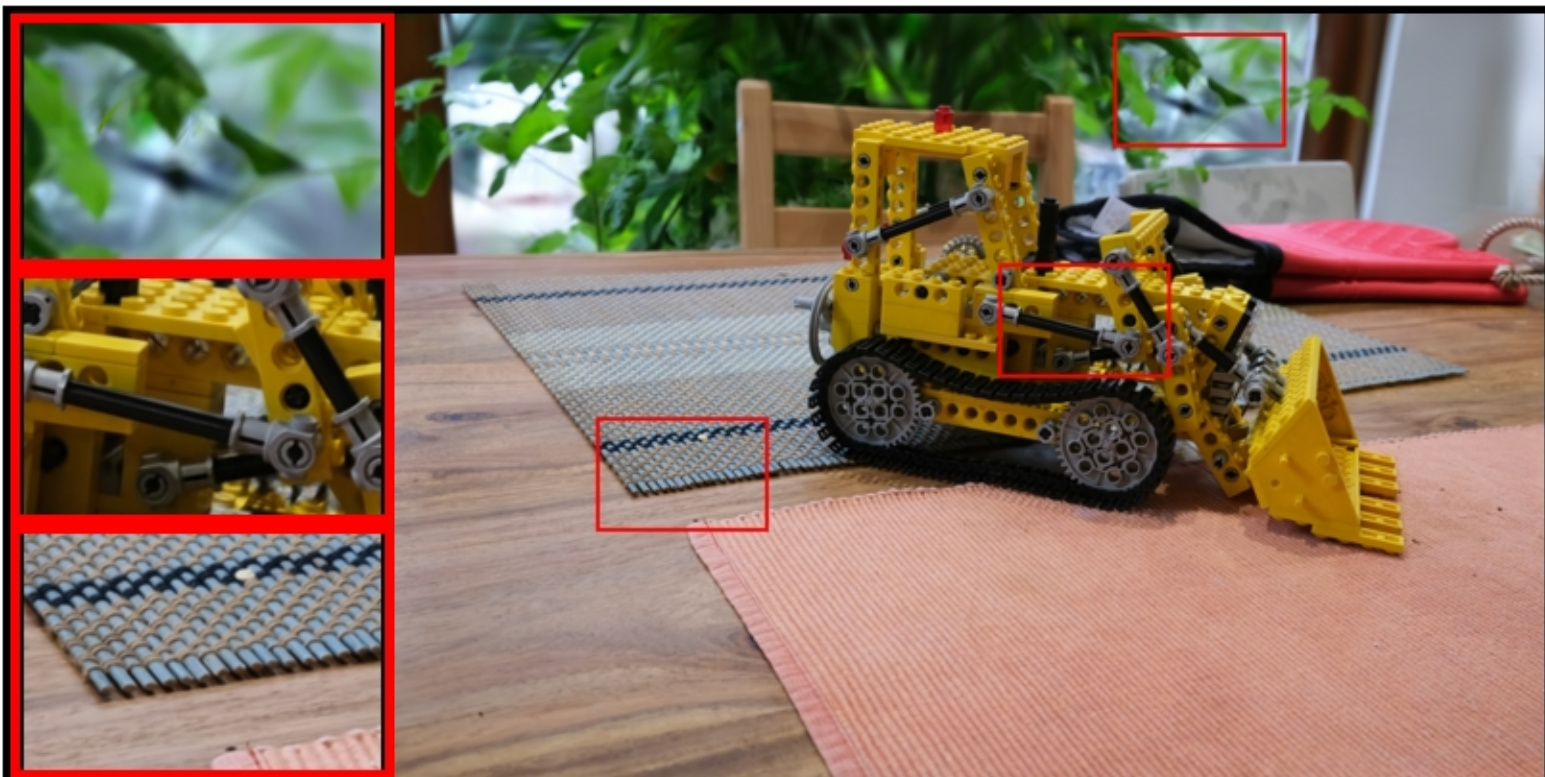
kitchen: Combined | COLMAP Cams | Both Pcds | confide PSNR: 22.17 | LPIPS: 0.1359 | SSIM: 0.5457
