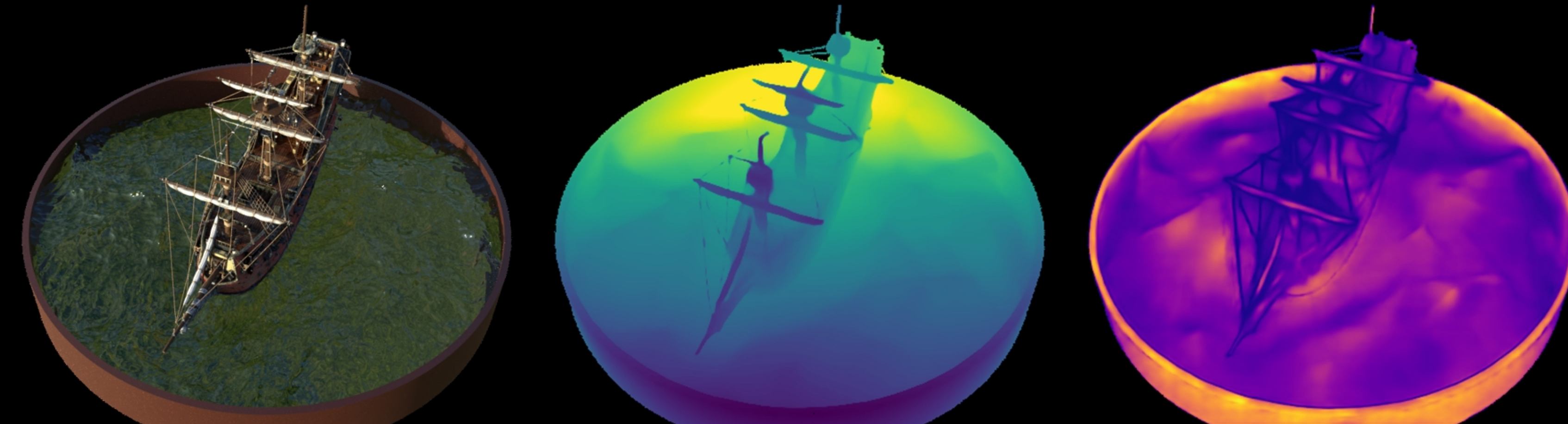
ship: Combined | COLMAP Cams | VGGT Pcd | confidence Original | Depth (max=6.66) | Confidence (max=793.41)
