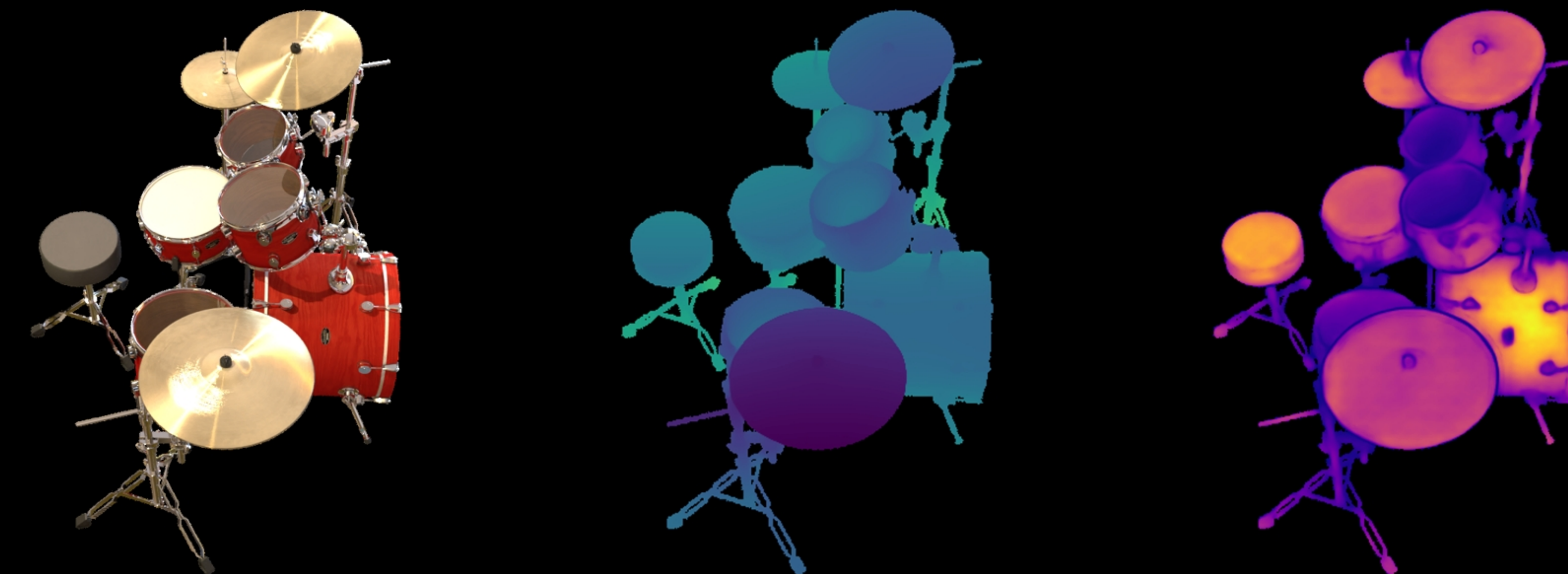
drums: Combined | COLMAP Cams | VGGT Pcd | confidence Original | Depth (max=5.54) | Confidence (max=1405.01)
