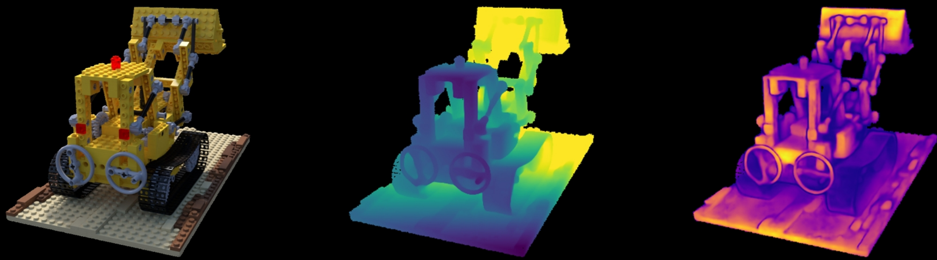
lego: Combined | COLMAP Cams | VGGT Pcd | confidence Original | Depth (max=5.88) | Confidence (max=713.75)
