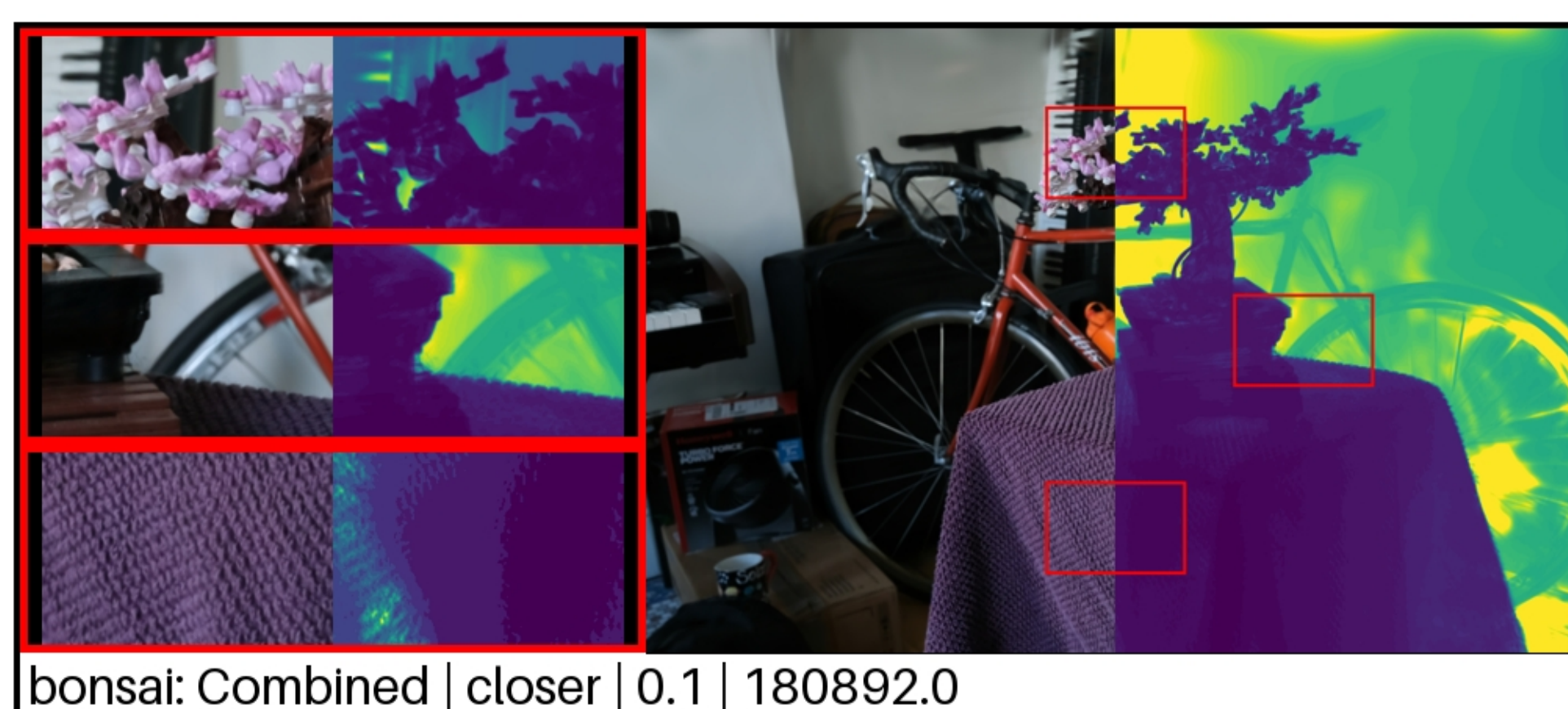
bonsai: Combined | closer | 0.1 | 180892.0 PSNR: 24.52 | LPIPS: 0.1712 | SSIM: 0.7662
