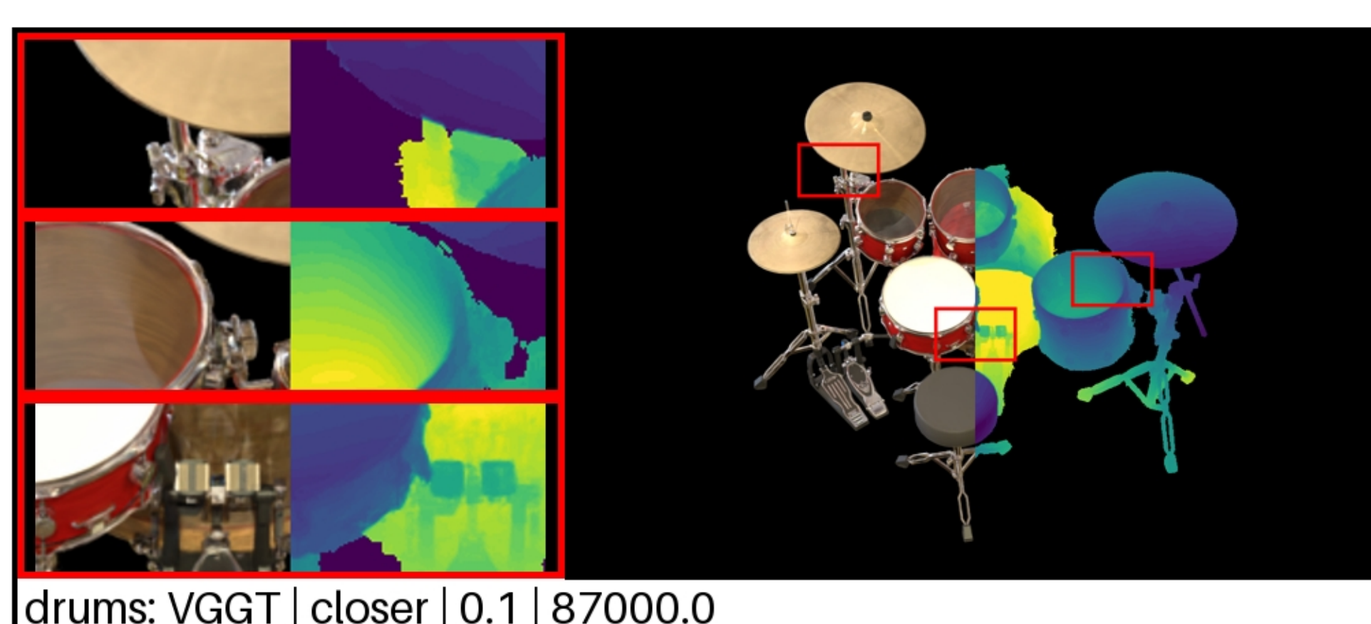
drums: VGGT | closer | 0.1 | 87000.0 PSNR: 19.48 | LPIPS: 0.0953 | SSIM: 0.8387
