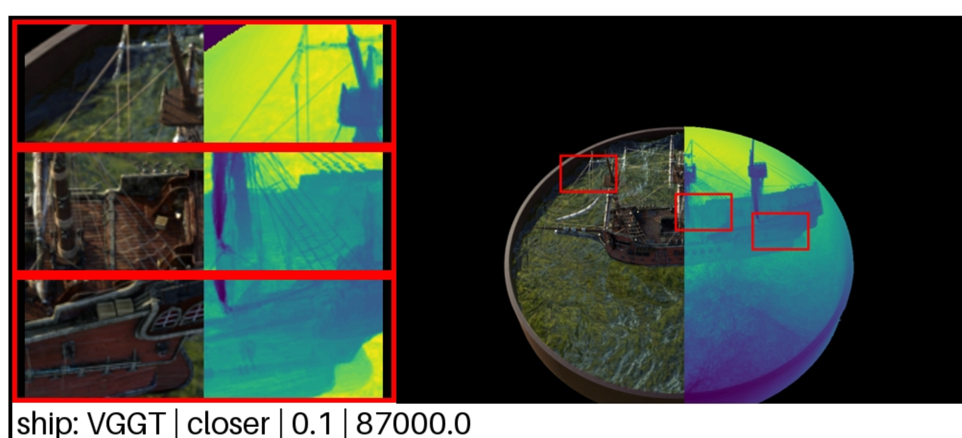
ship: VGGT | closer | 0.1 | 87000.0 PSNR: 22.43 | LPIPS: 0.1392 | SSIM: 0.7386
