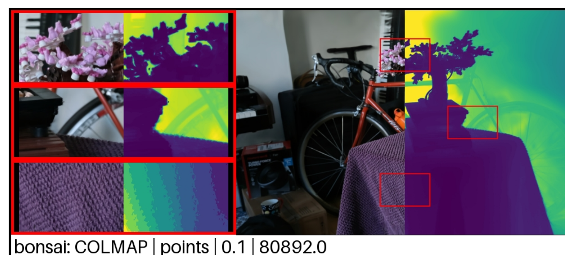
bonsai: COLMAP | points | 0.1 | 80892.0 PSNR: 26.85 | LPIPS: 0.1693 | SSIM: 0.8499
