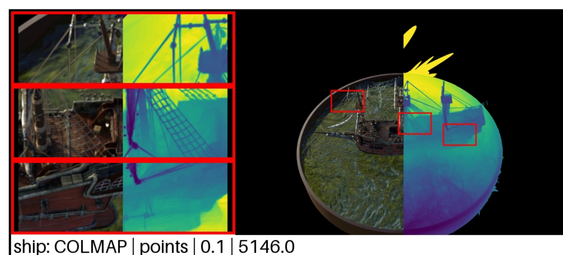
ship: COLMAP | points | 0.1 | 5146.0 PSNR: 22.71 | LPIPS: 0.1424 | SSIM: 0.7608
