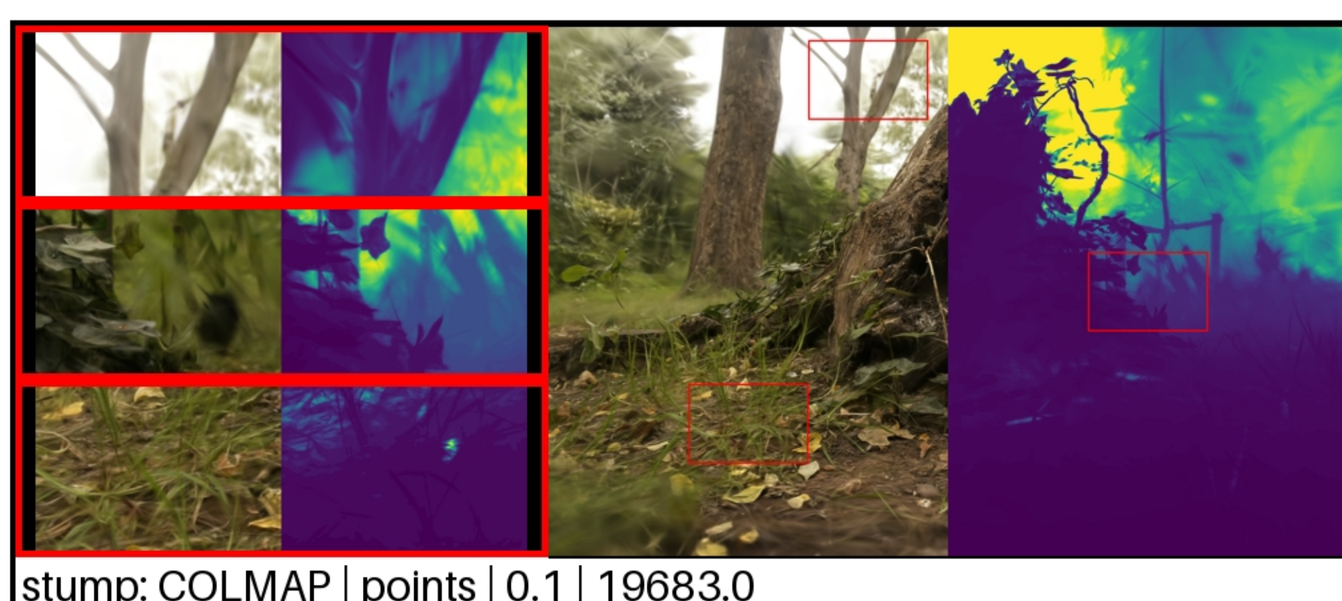
stump: COLMAP | points | 0.1 | 19683.0 PSNR: 25.16 | LPIPS: 0.3472 | SSIM: 0.7144
