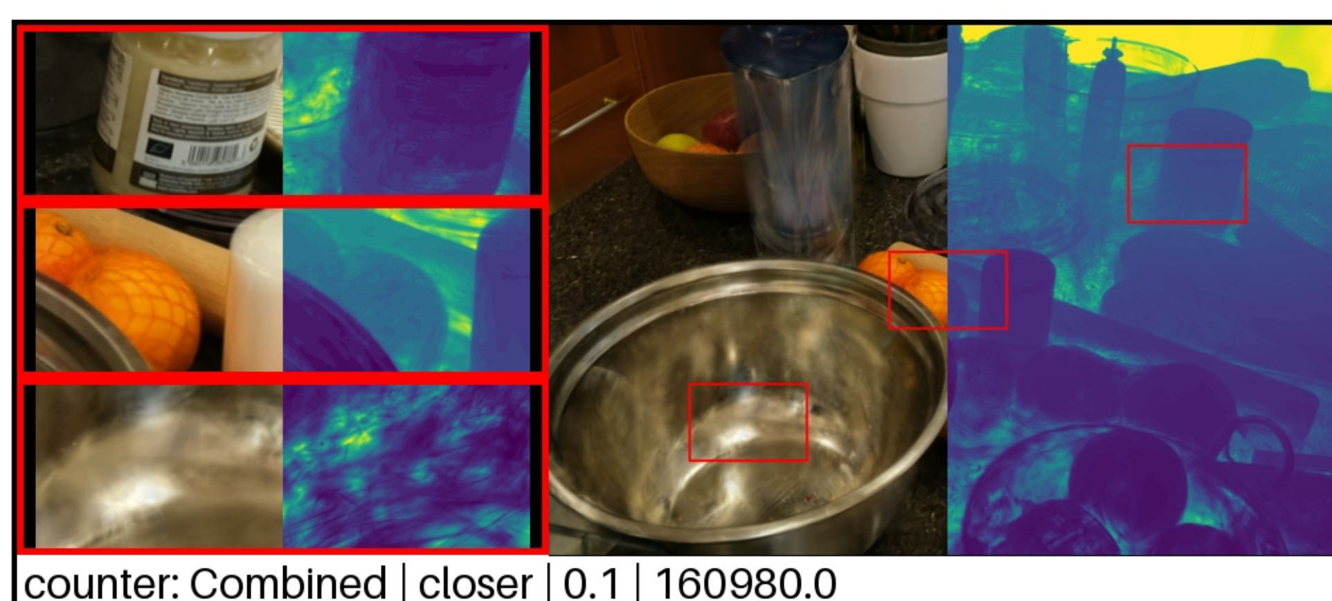
counter: Combined | closer | 0.1 | 160980.0 PSNR: 24.97 | LPIPS: 0.1880 | SSIM: 0.8449
