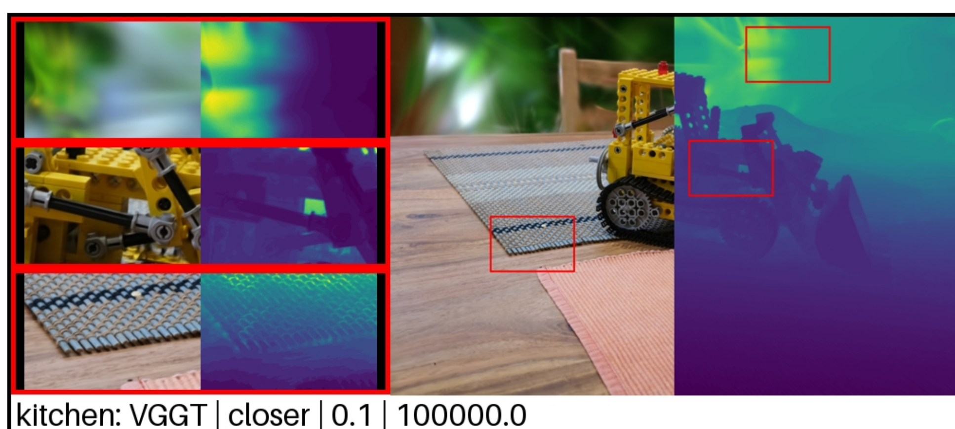
kitchen: VGGT | closer | 0.1 | 100000.0 PSNR: 19.86 | LPIPS: 0.1998 | SSIM: 0.4151
