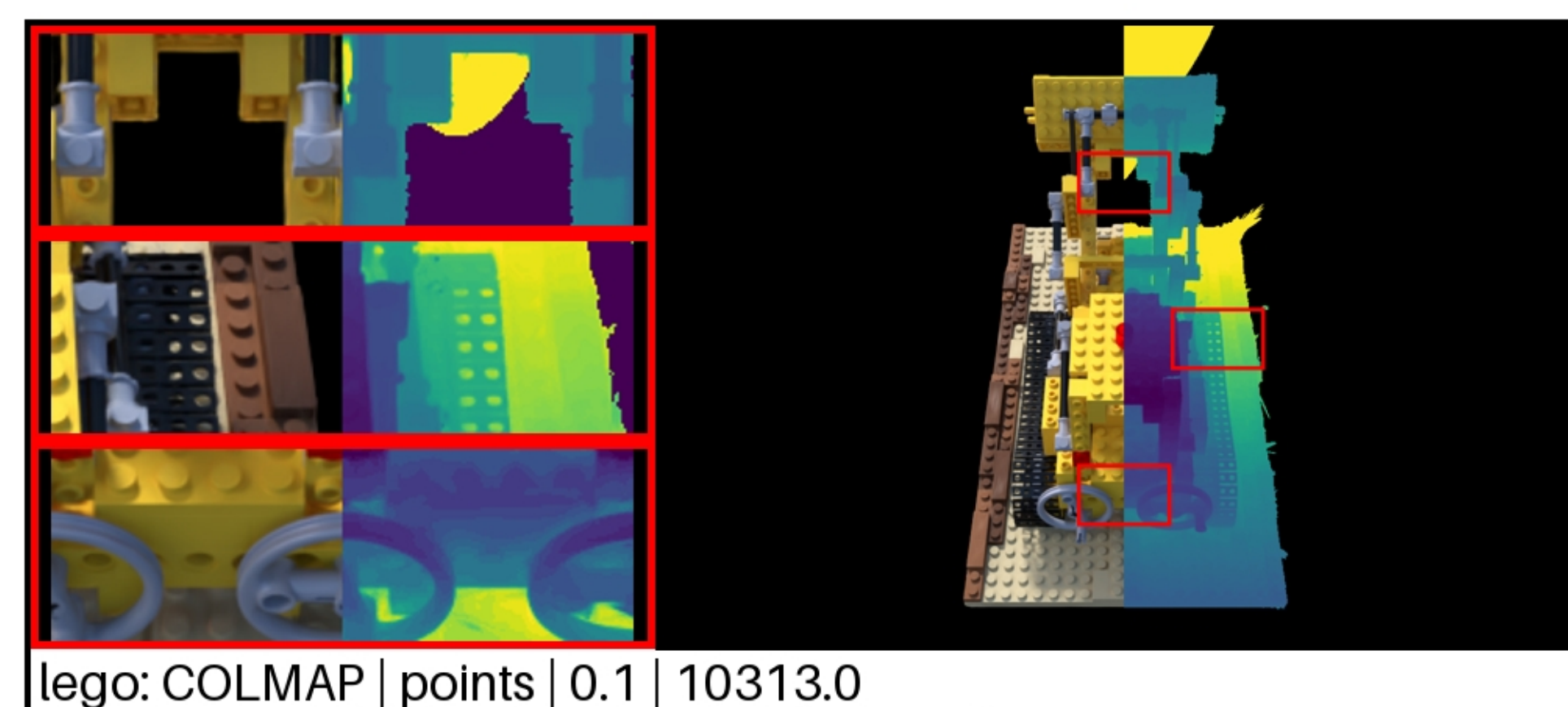
lego: COLMAP | points | 0.1 | 10313.0 PSNR: 23.40 | LPIPS: 0.0611 | SSIM: 0.8649
