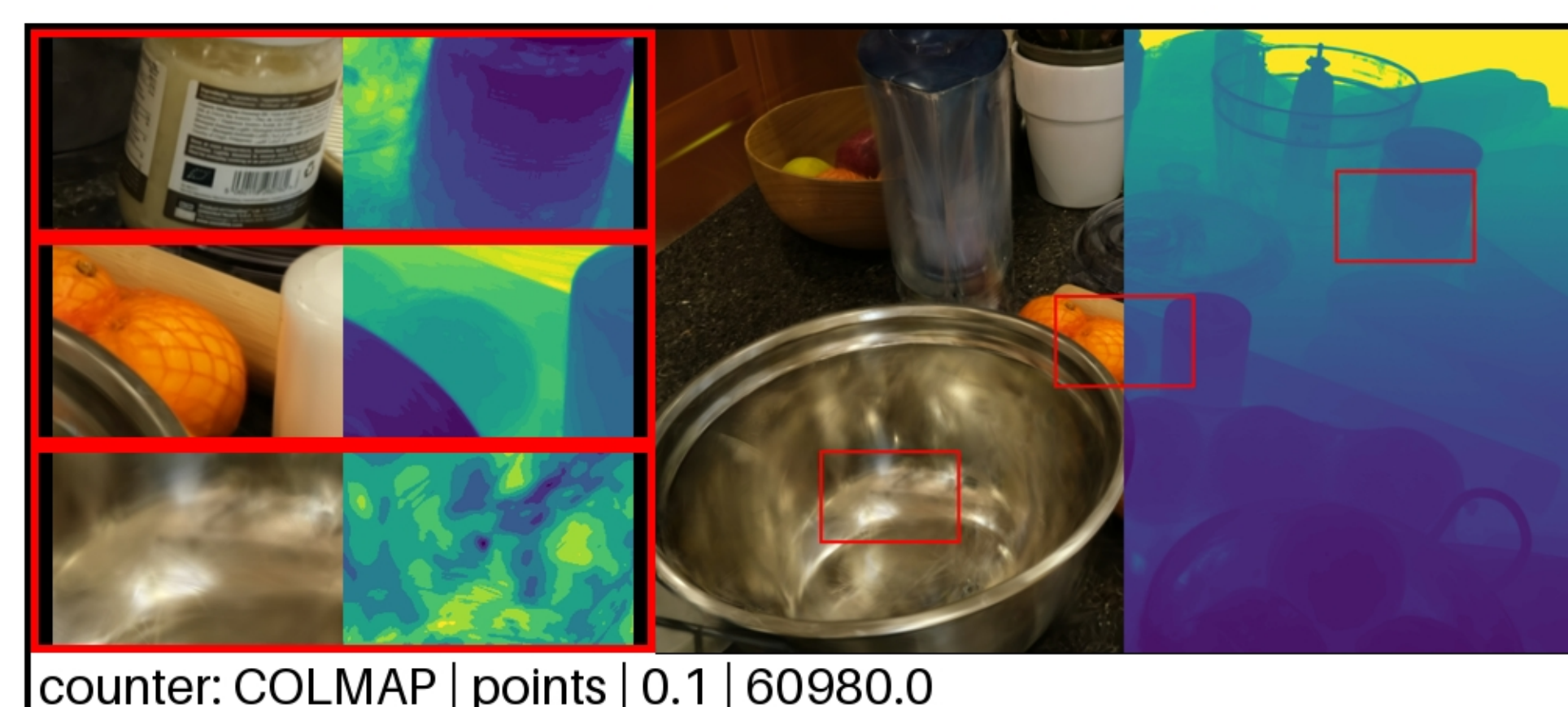
counter: COLMAP | points | 0.1 | 60980.0 PSNR: 25.12 | LPIPS: 0.1878 | SSIM: 0.8470
