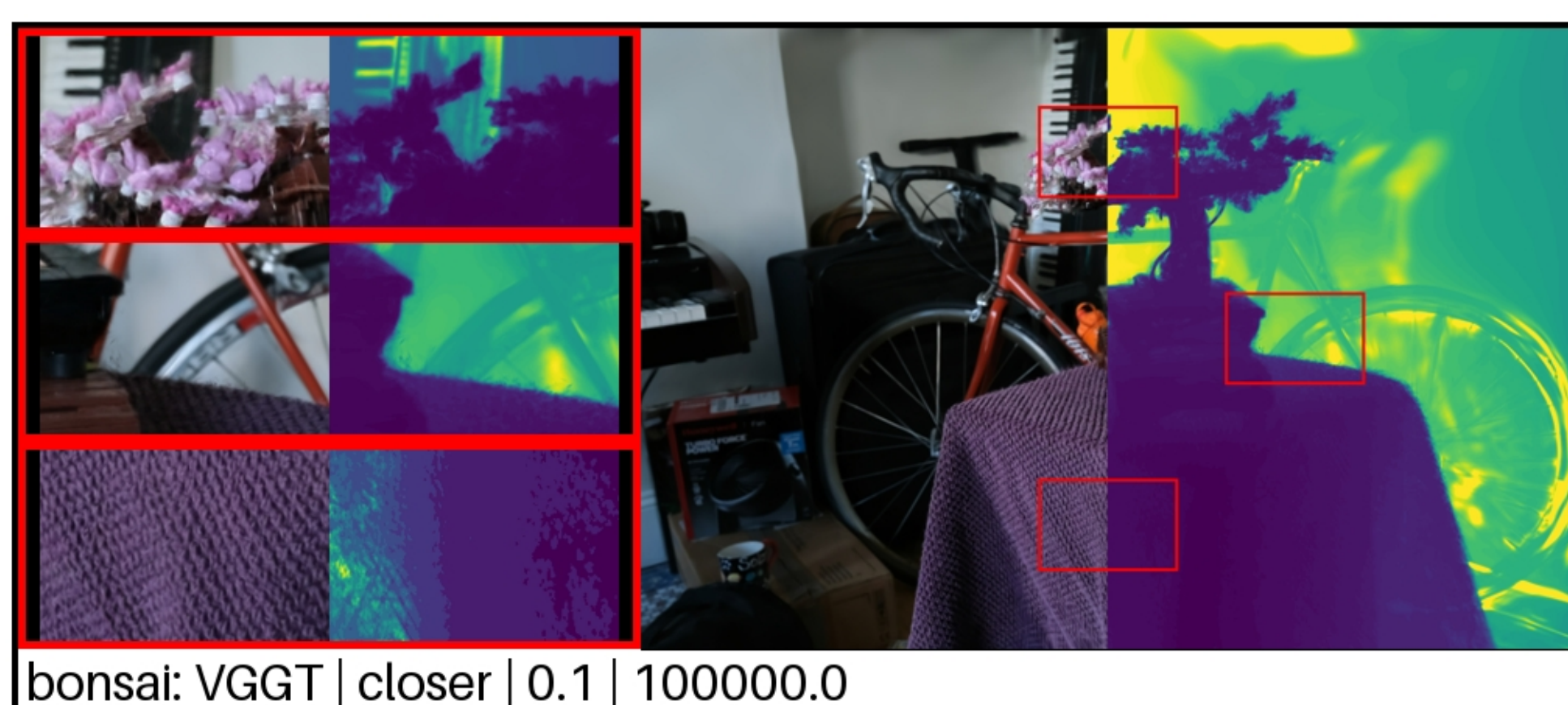
bonsai: VGGT | closer | 0.1 | 100000.0 PSNR: 17.41 | LPIPS: 0.4003 | SSIM: 0.5601
