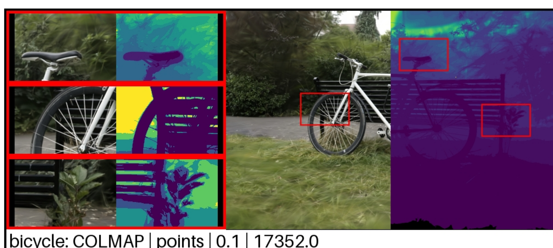
bicycle: COLMAP | points | 0.1 | 17352.0 PSNR: 21.97 | LPIPS: 0.3727 | SSIM: 0.5258
