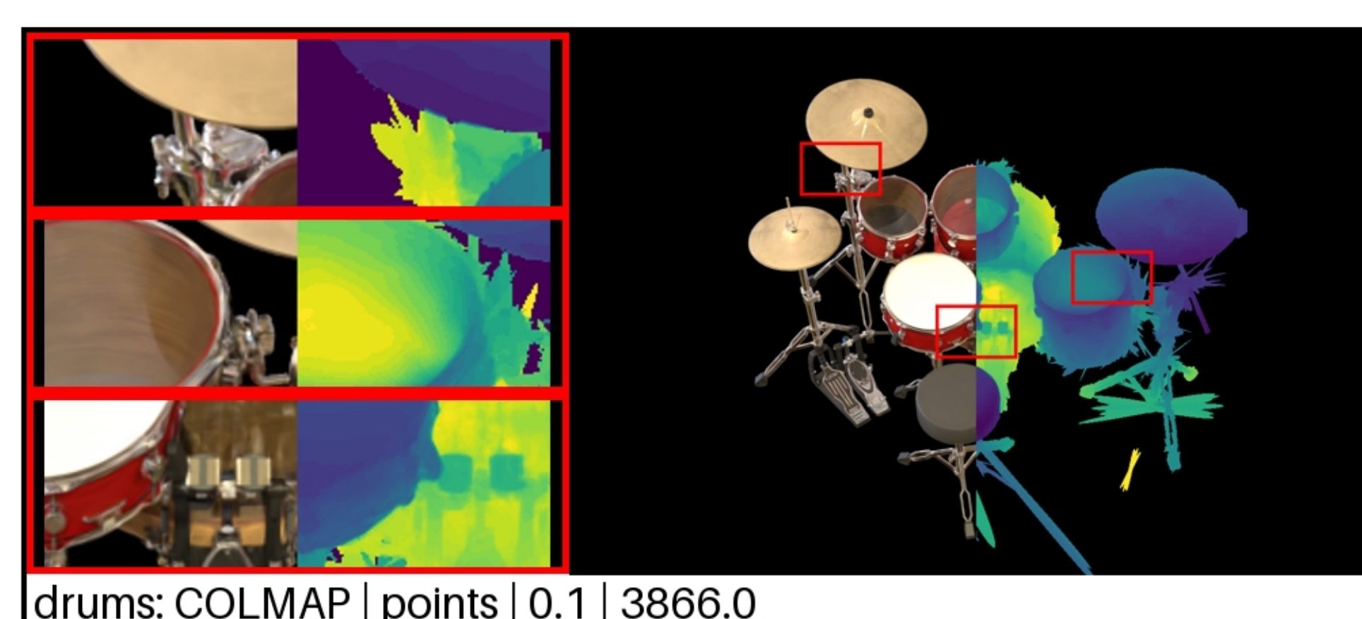
drums: COLMAP | points | 0.1 | 3866.0 PSNR: 22.90 | LPIPS: 0.0897 | SSIM: 0.9056
