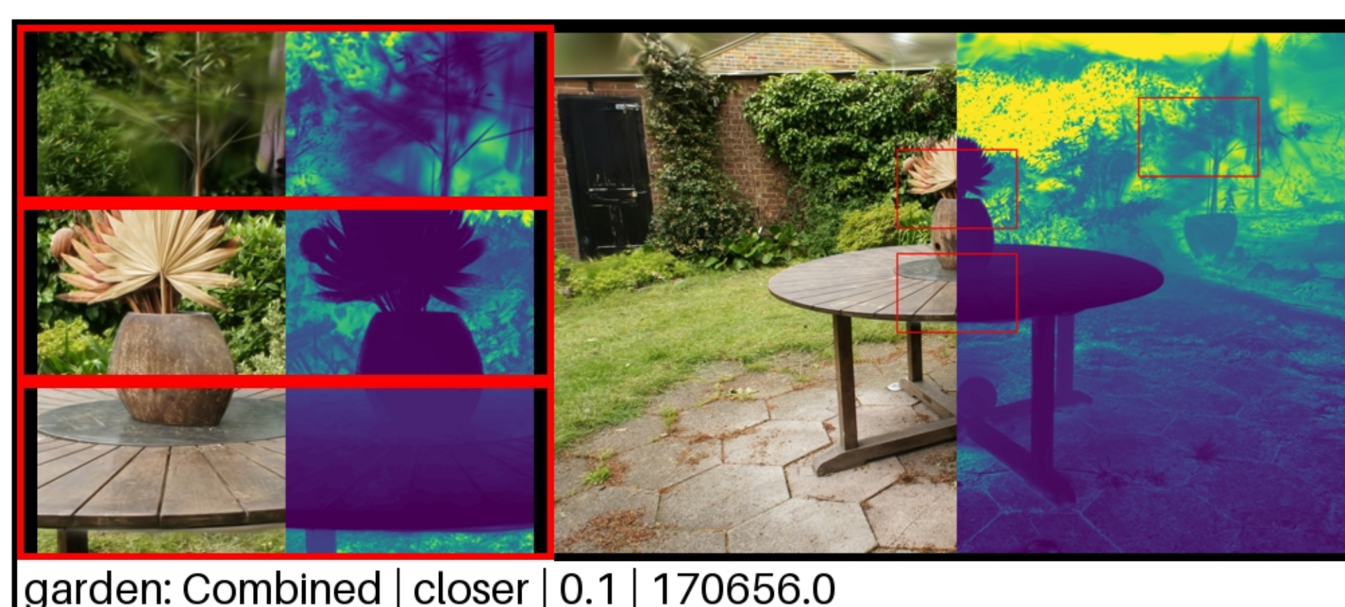
garden: Combined | closer | 0.1 | 170656.0 PSNR: 22.78 | LPIPS: 0.2462 | SSIM: 0.5662
