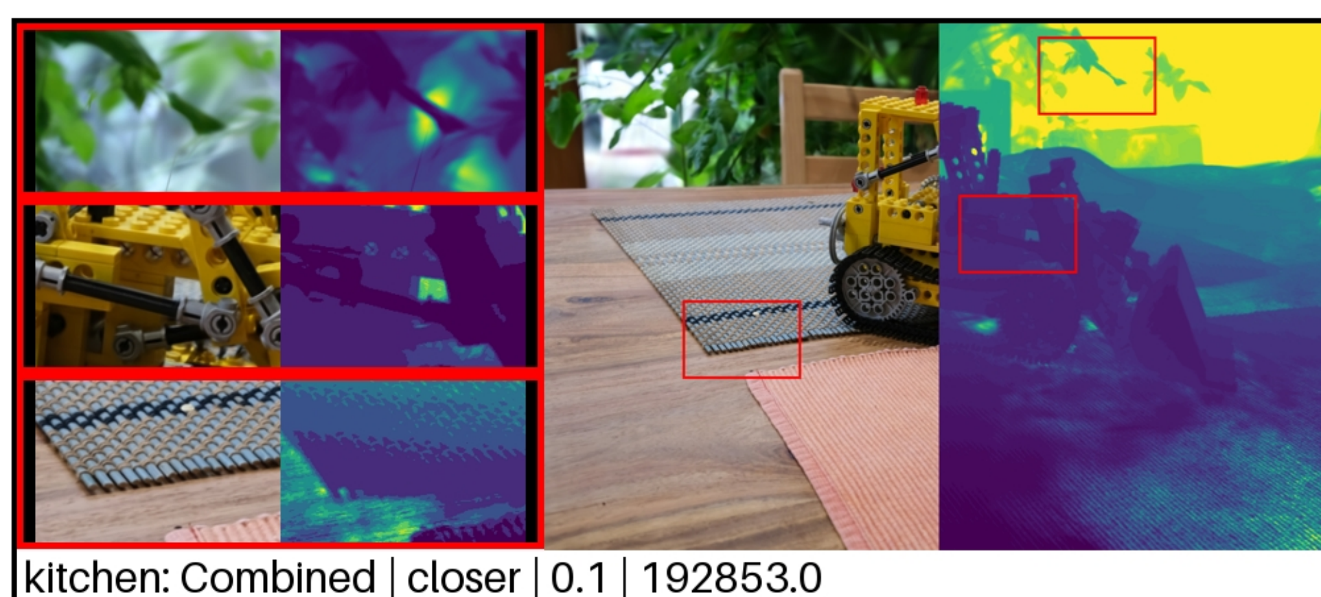
kitchen: Combined | closer | 0.1 | 192853.0 PSNR: 23.09 | LPIPS: 0.1317 | SSIM: 0.6298
