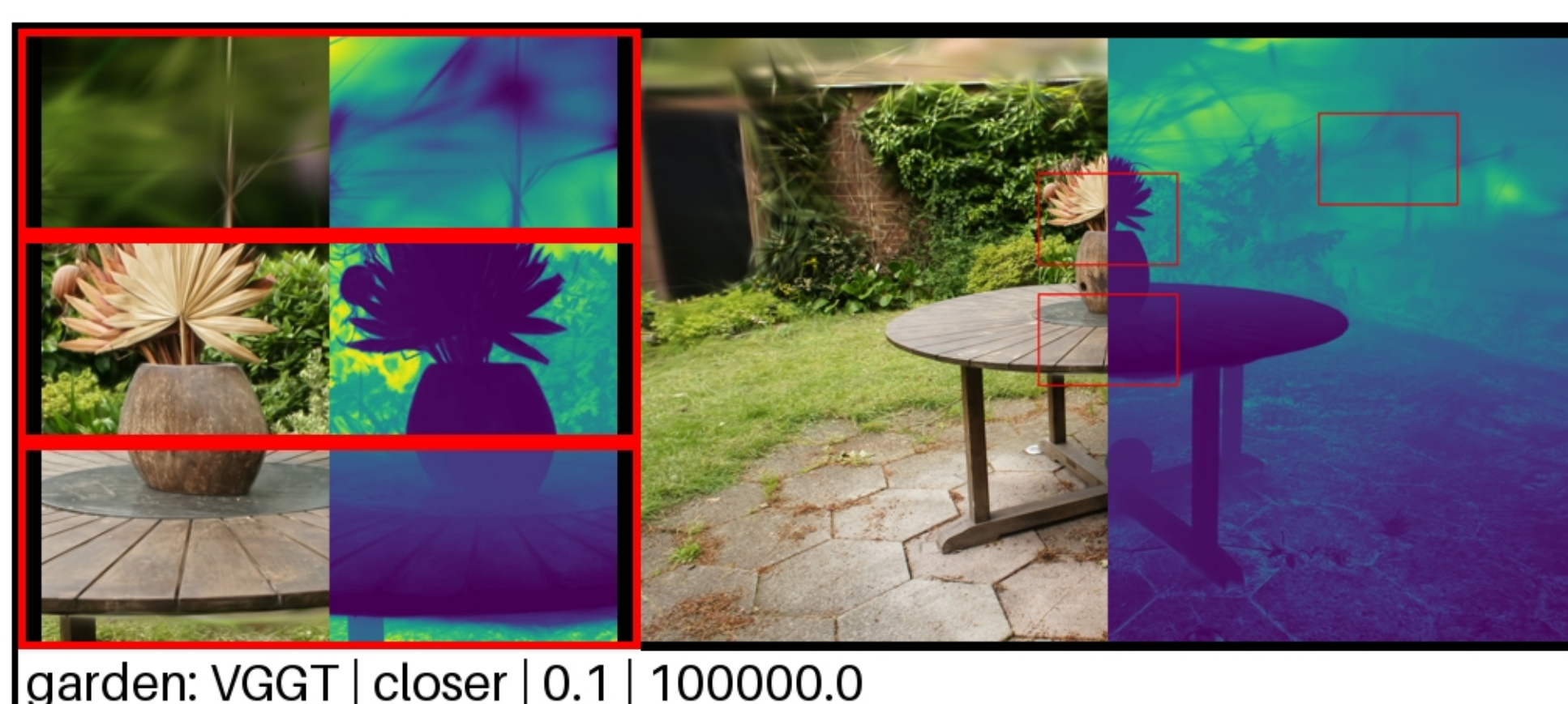
garden: VGGT | closer | 0.1 | 100000.0 PSNR: 19.54 | LPIPS: 0.3812 | SSIM: 0.3658
