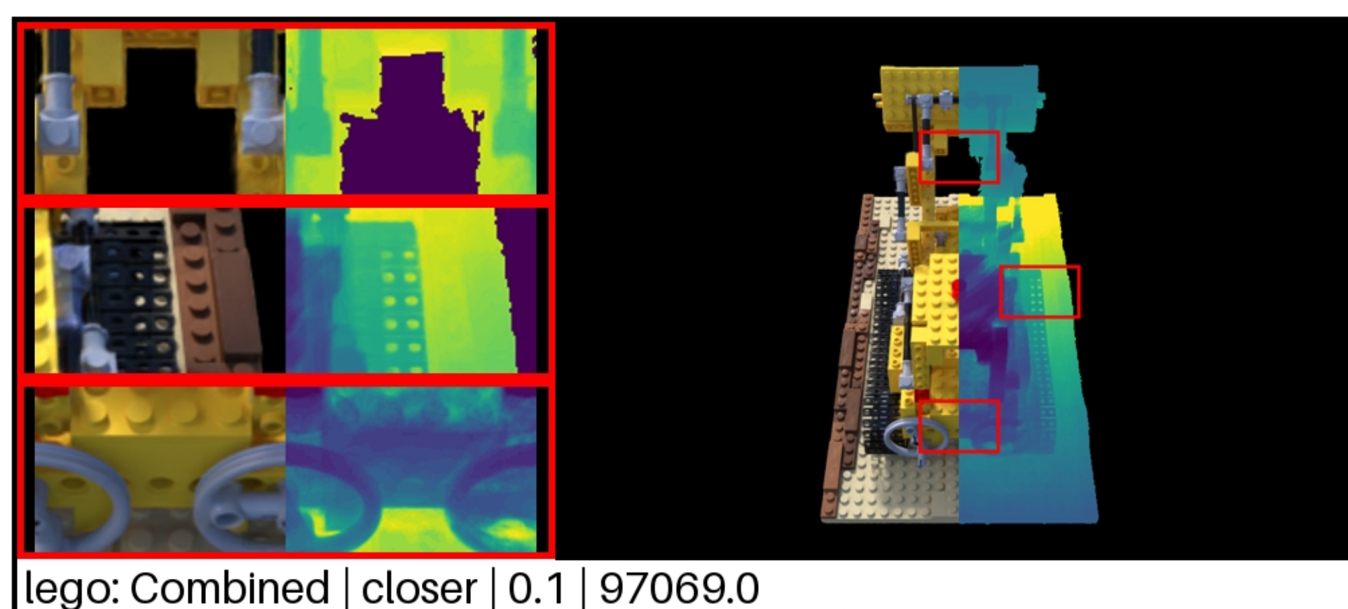
lego: Combined | closer | 0.1 | 97069.0 PSNR: 25.06 | LPIPS: 0.0625 | SSIM: 0.8942
