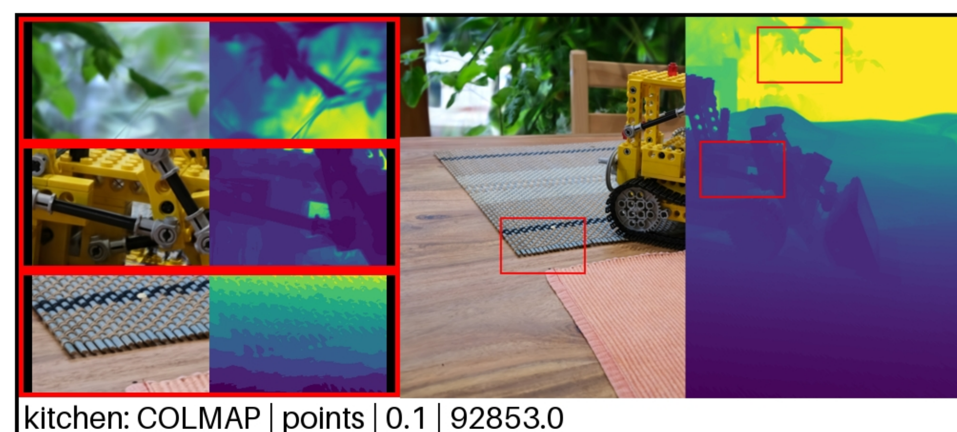
kitchen: COLMAP | points | 0.1 | 92853.0 PSNR: 21.63 | LPIPS: 0.1450 | SSIM: 0.5155
