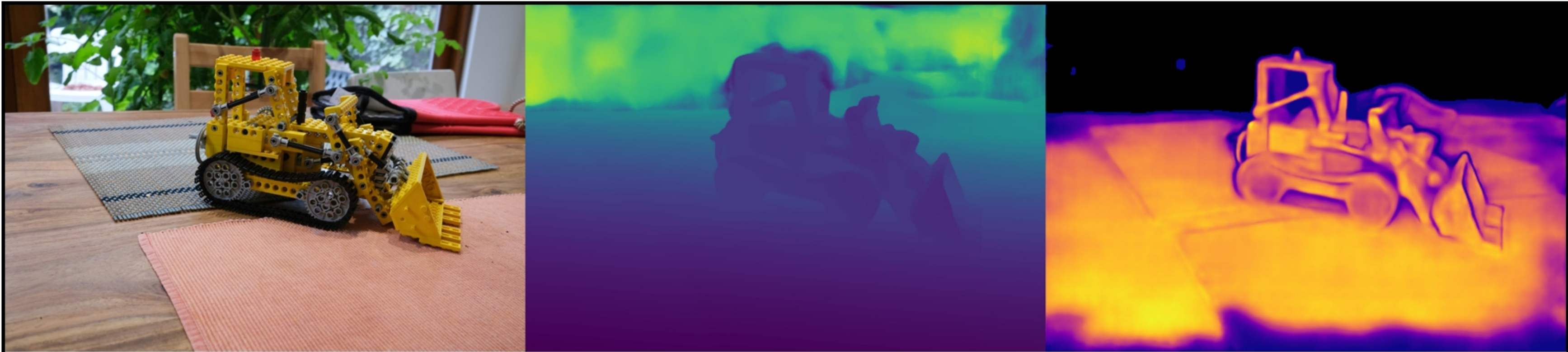
kitchen: VGGT | closer | 0.1 | 100000 Original | Depth (max=2.43) | Confidence (max=30.80)
