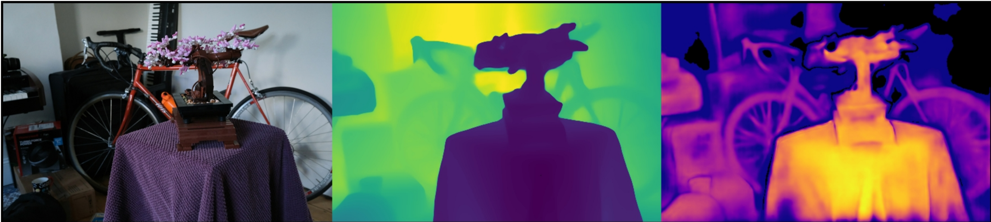
bonsai: VGGT | closer | 0.1 | 100000 Original | Depth (max=2.21) | Confidence (max=5.14)
