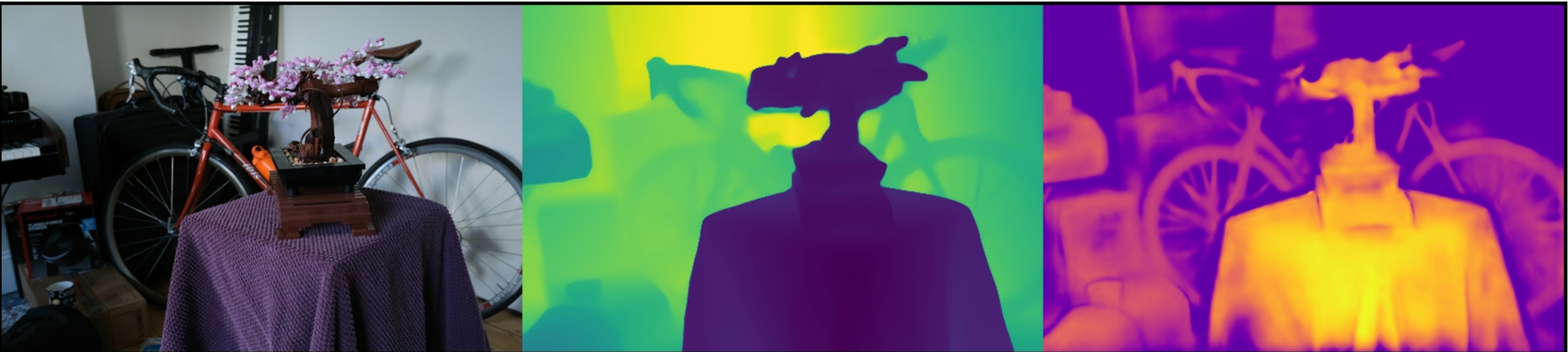
bonsai: Combined | closer | 0.1 | 180892 Original | Depth (max=15.46) | Confidence (max=35.95)
