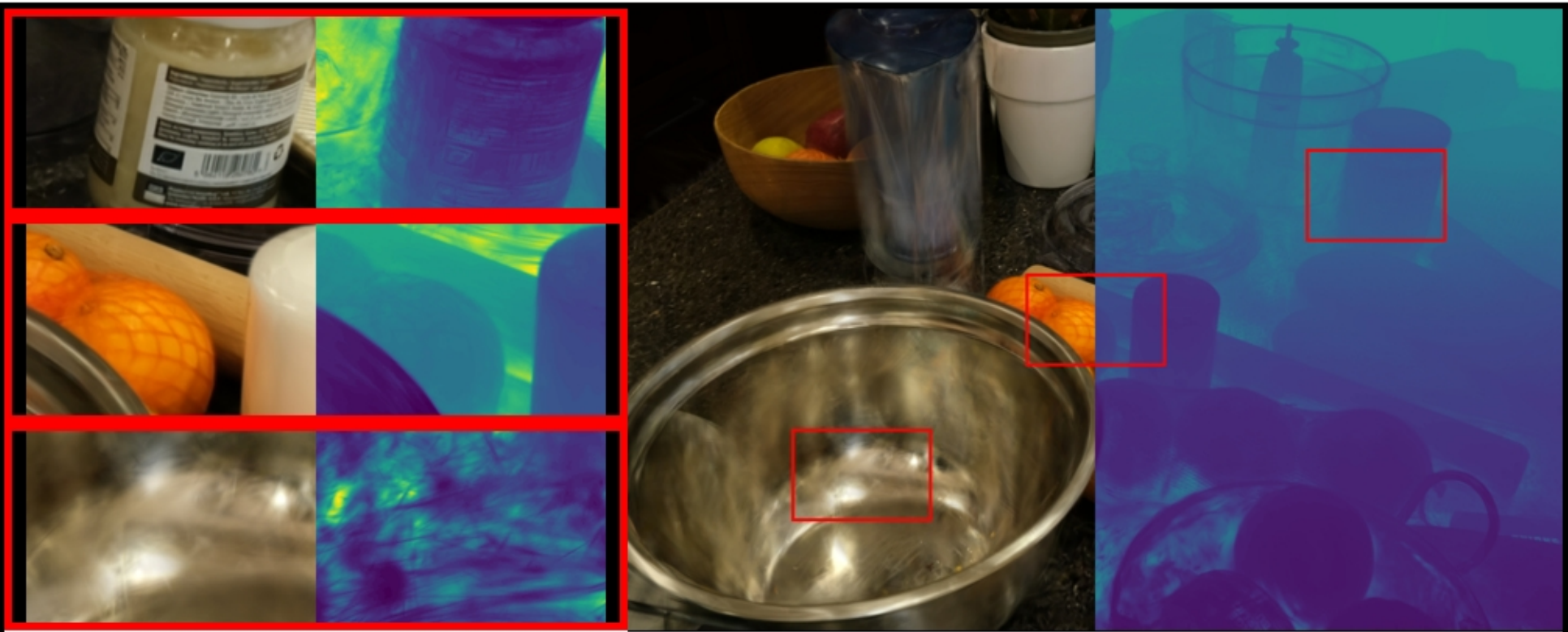
counter: VGGT | closer | 0.1 | 100000 PSNR: 20.51 | LPIPS: 0.2588 | SSIM: 0.6339
