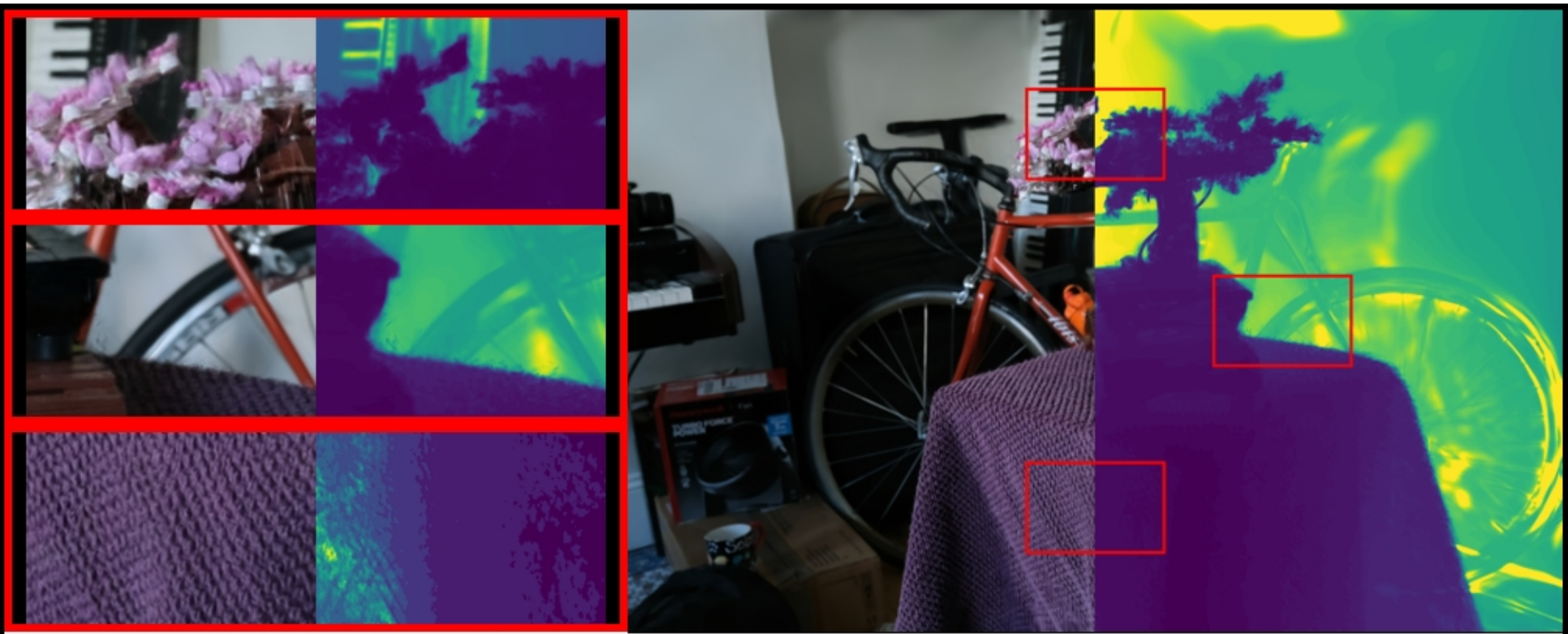
bonsai: VGGT | closer | 0.1 | 100000 PSNR: 17.41 | LPIPS: 0.4003 | SSIM: 0.5601
