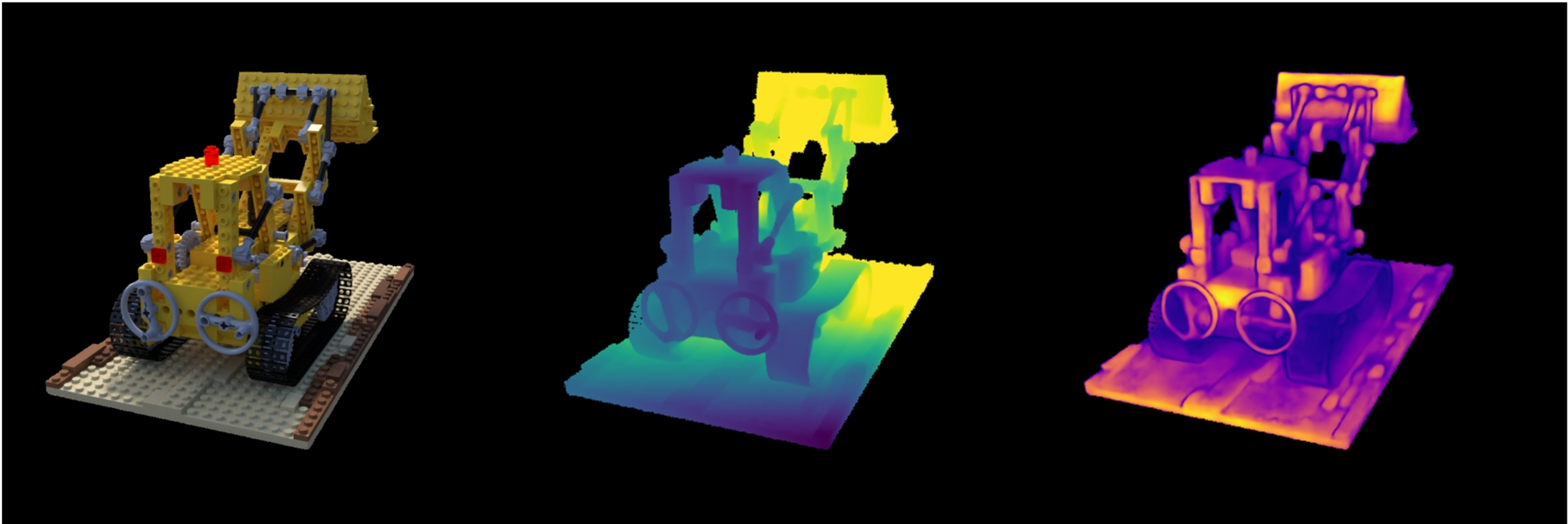
lego: VGGT | closer | 0.1 | 87000 Original | Depth (max=1.28) | Confidence (max=155.74)
