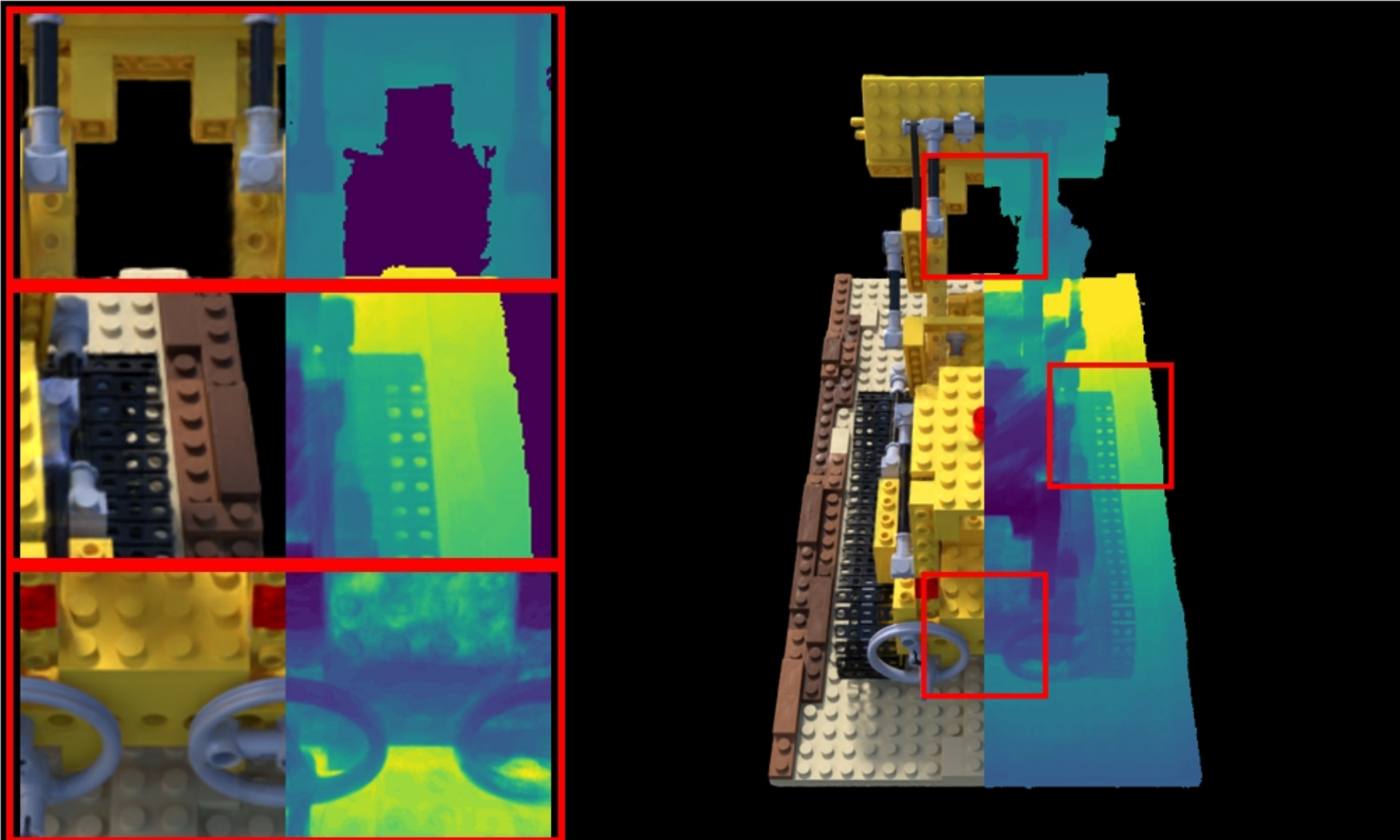
lego: Combined | closer | 0.1 | 97069 PSNR: 25.06 | LPIPS: 0.0625 | SSIM: 0.8942
