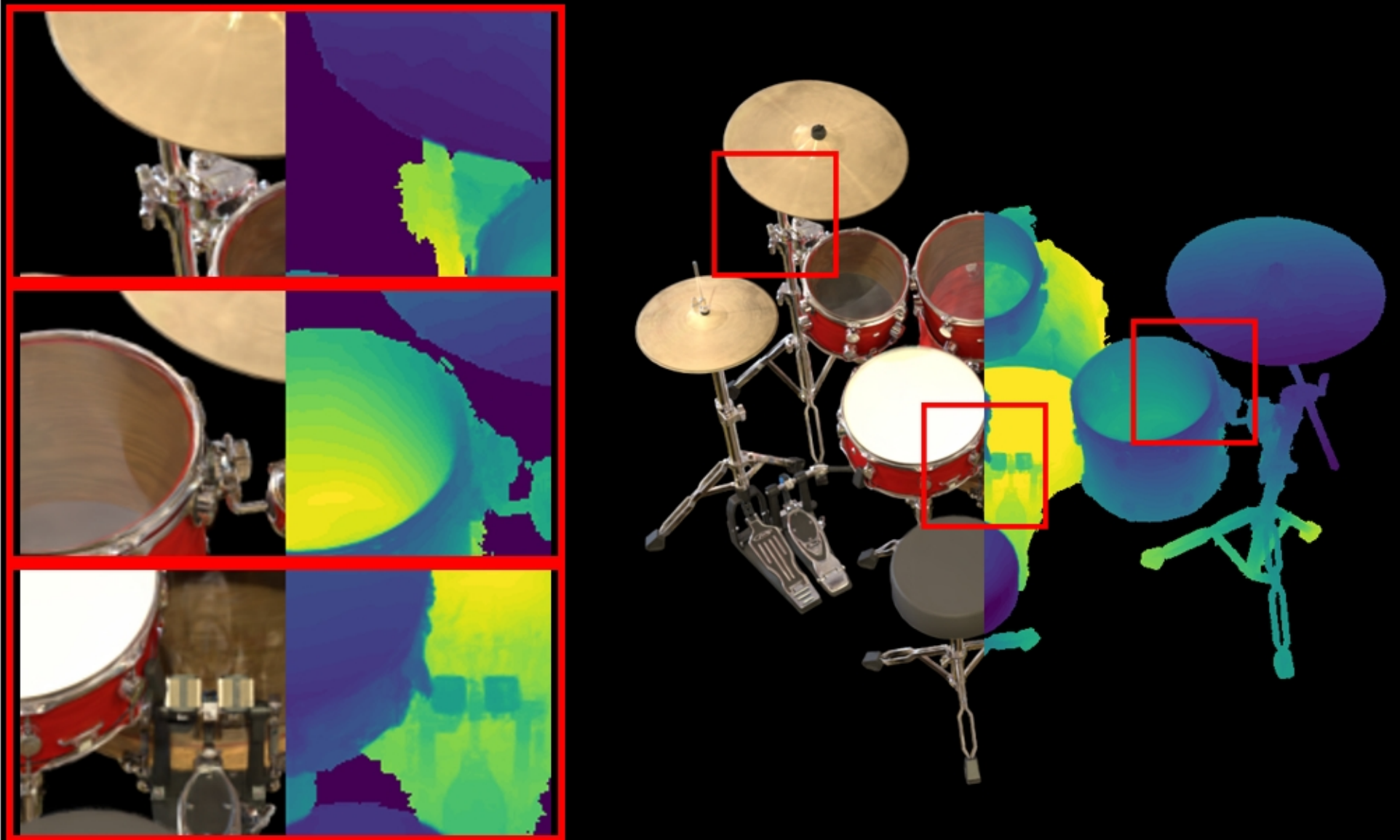
drums: VGGT | closer | 0.1 | 87000 PSNR: 19.48 | LPIPS: 0.0953 | SSIM: 0.8387
