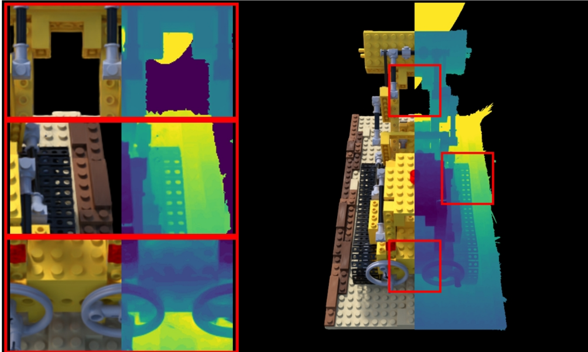
lego: COLMAP | points | 0.1 | 10313 PSNR: 23.40 | LPIPS: 0.0611 | SSIM: 0.8649
