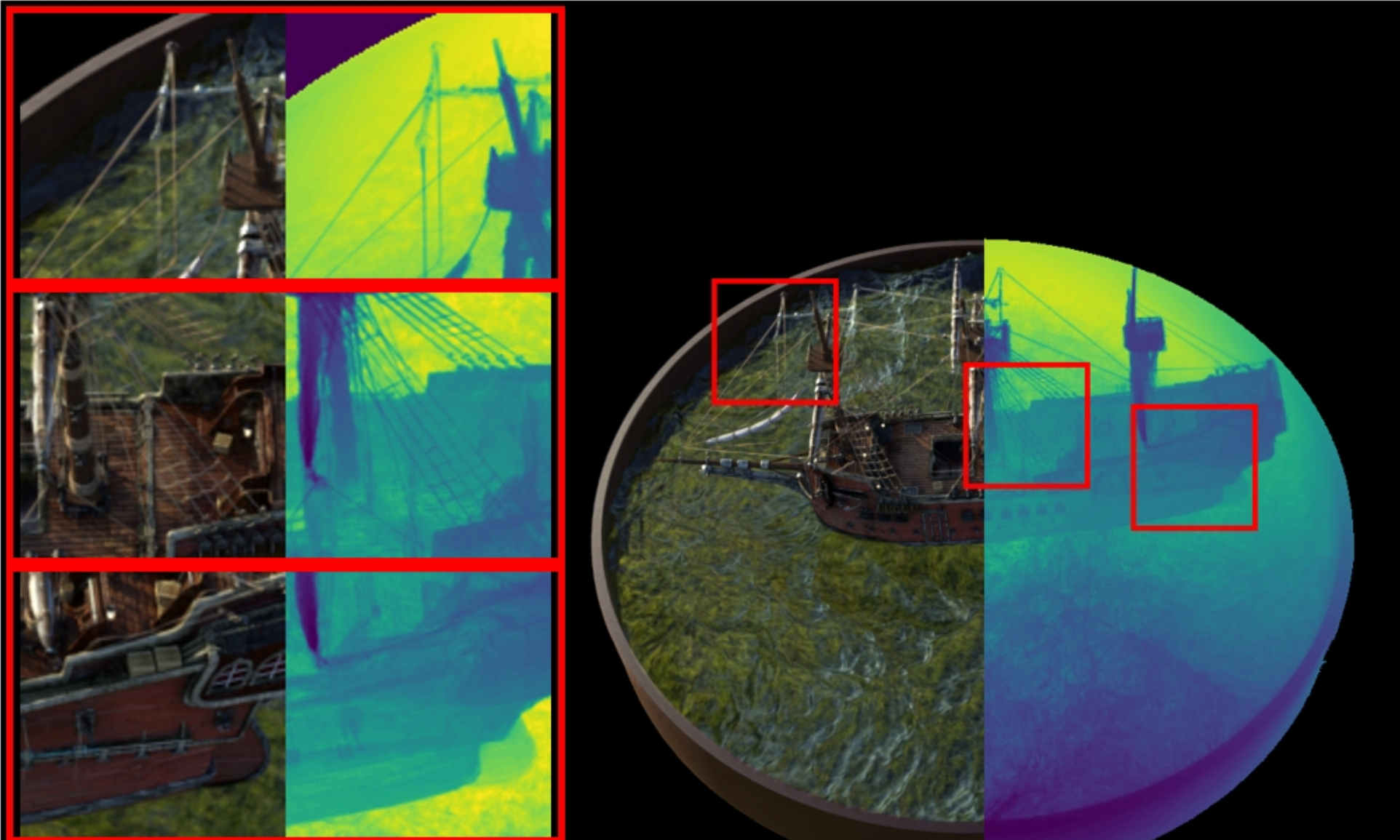
ship: VGGT | closer | 0.1 | 87000 PSNR: 22.43 | LPIPS: 0.1392 | SSIM: 0.7386
