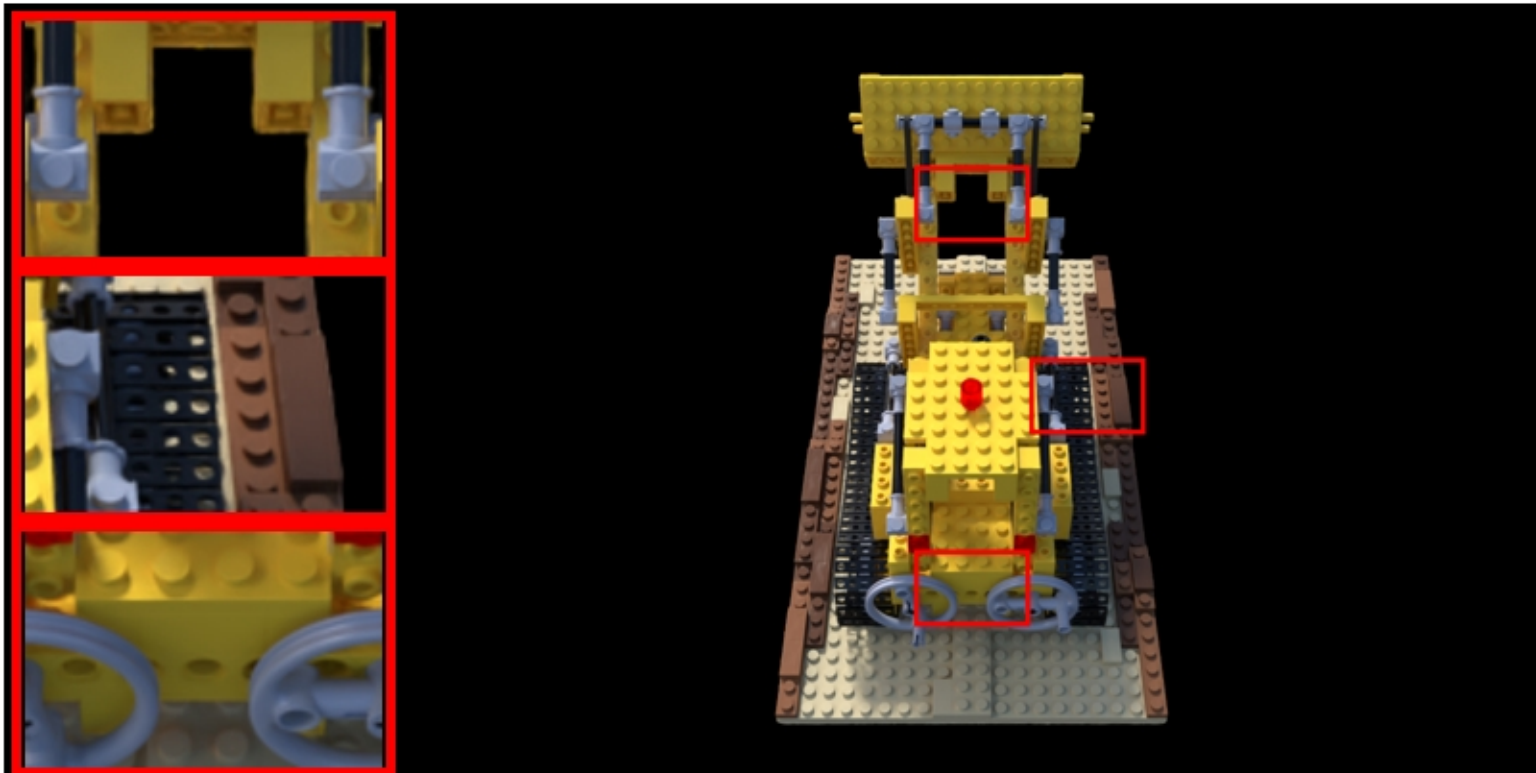
lego: VGGT | 0 | Pose Opt PSNR: 20.35 | LPIPS: 0.0759 | SSIM: 0.7735
