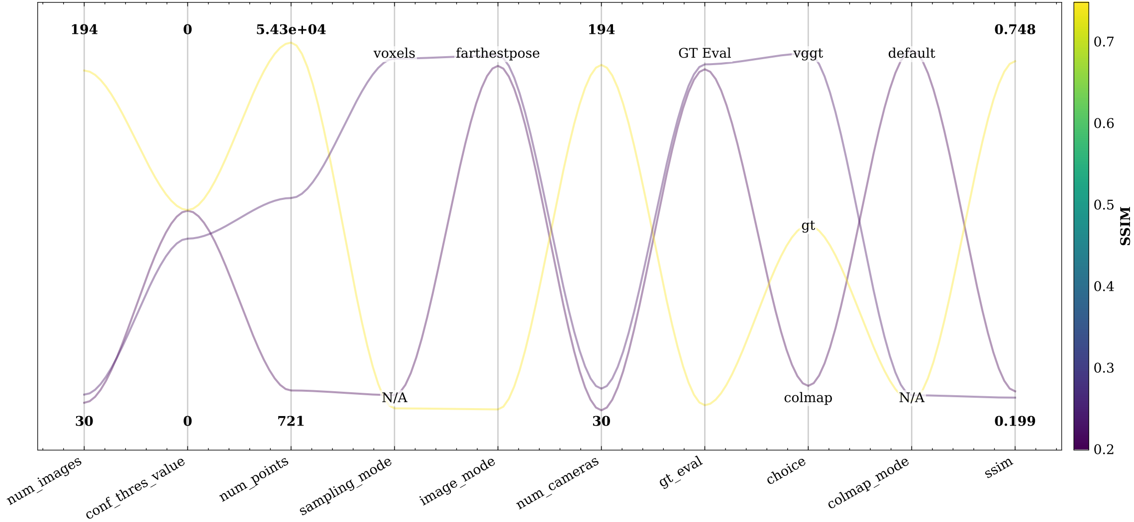
Parallel Coordinate Plot: Parameters vs SSIM
