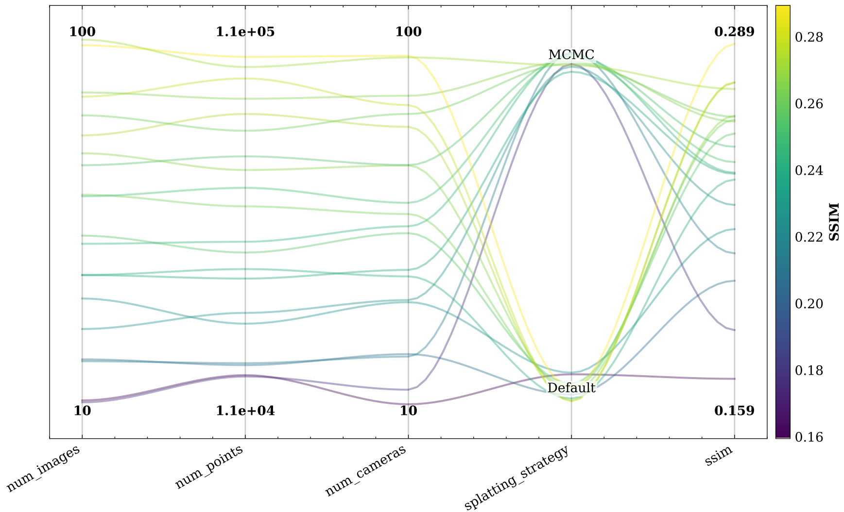
Parallel Coordinate Plot: Parameters vs SSIM
