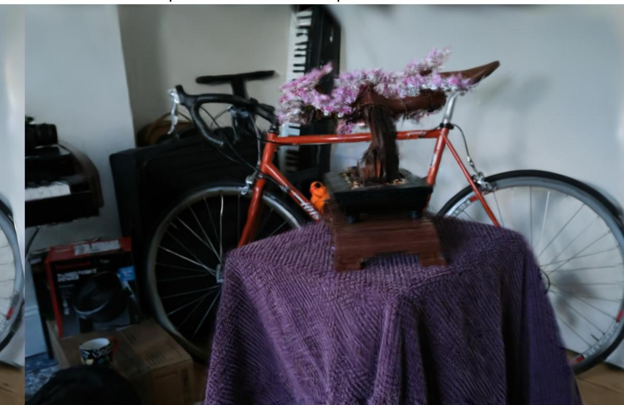
Config: VGGT | num_images=100 PSNR: 17.73 | LPIPS: 0.3776 | SSIM: 0.5716
