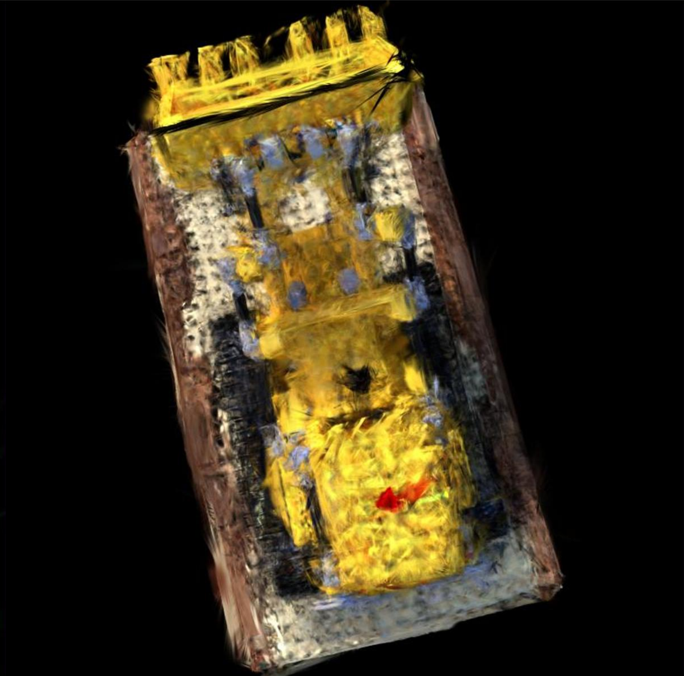
Config: VGGT | Pose Opt | num_images=30 PSNR: 13.54 | LPIPS: 0.3251 | SSIM: 0.6138
