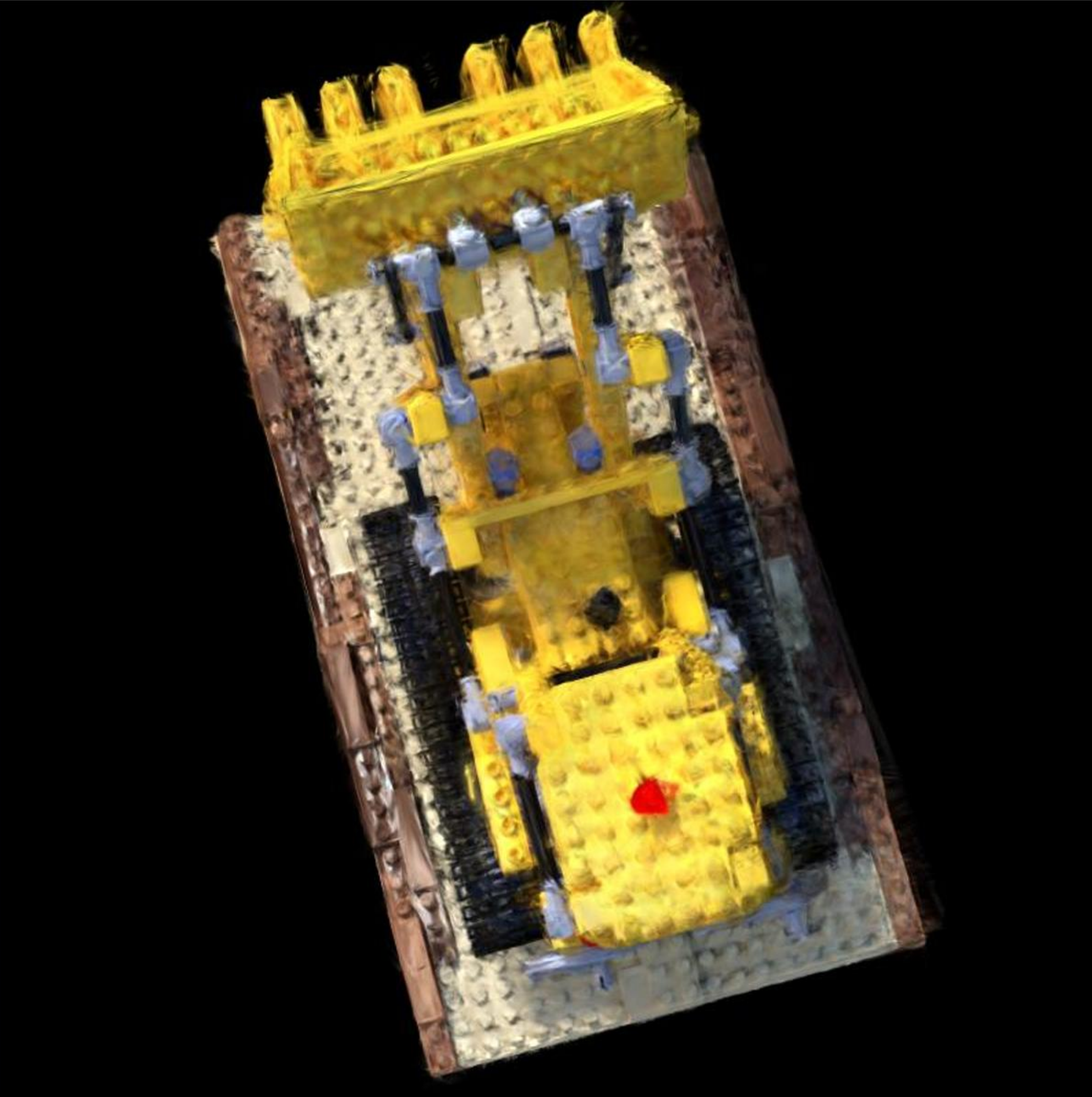
Config: VGGT | Pose Opt | num_images=40 PSNR: 14.47 | LPIPS: 0.2686 | SSIM: 0.6444
