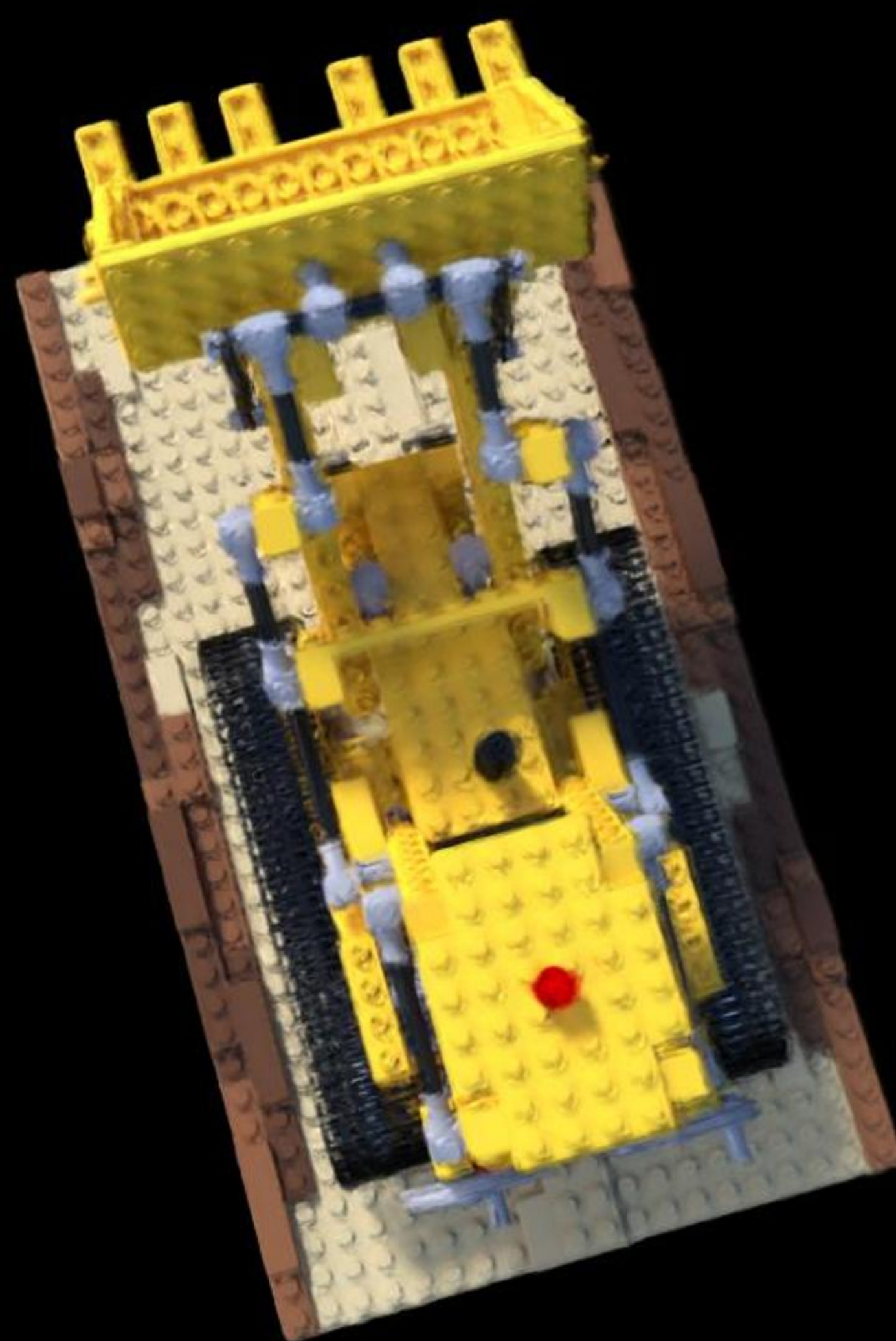
Config: VGGT | num_points=87000 PSNR: 19.05 | LPIPS: 0.1211 | SSIM: 0.7407
