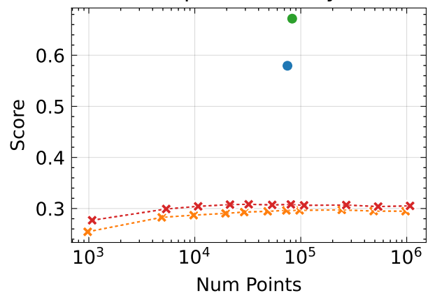
Composite Quality ↑
