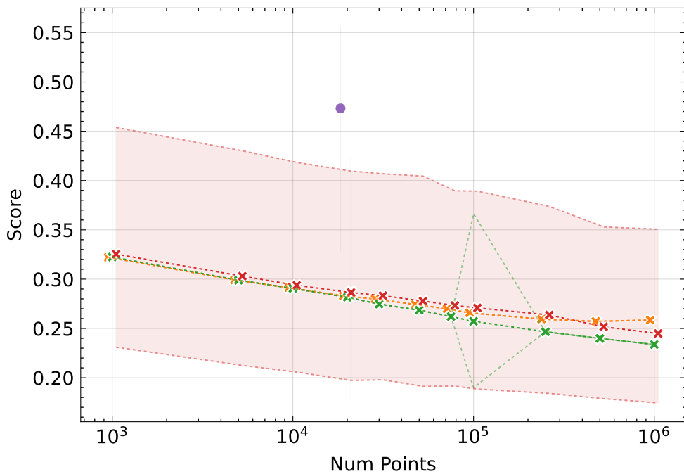
SSIM \uparrow
