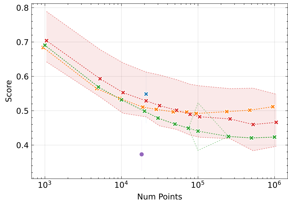
LPIPS \downarrow
