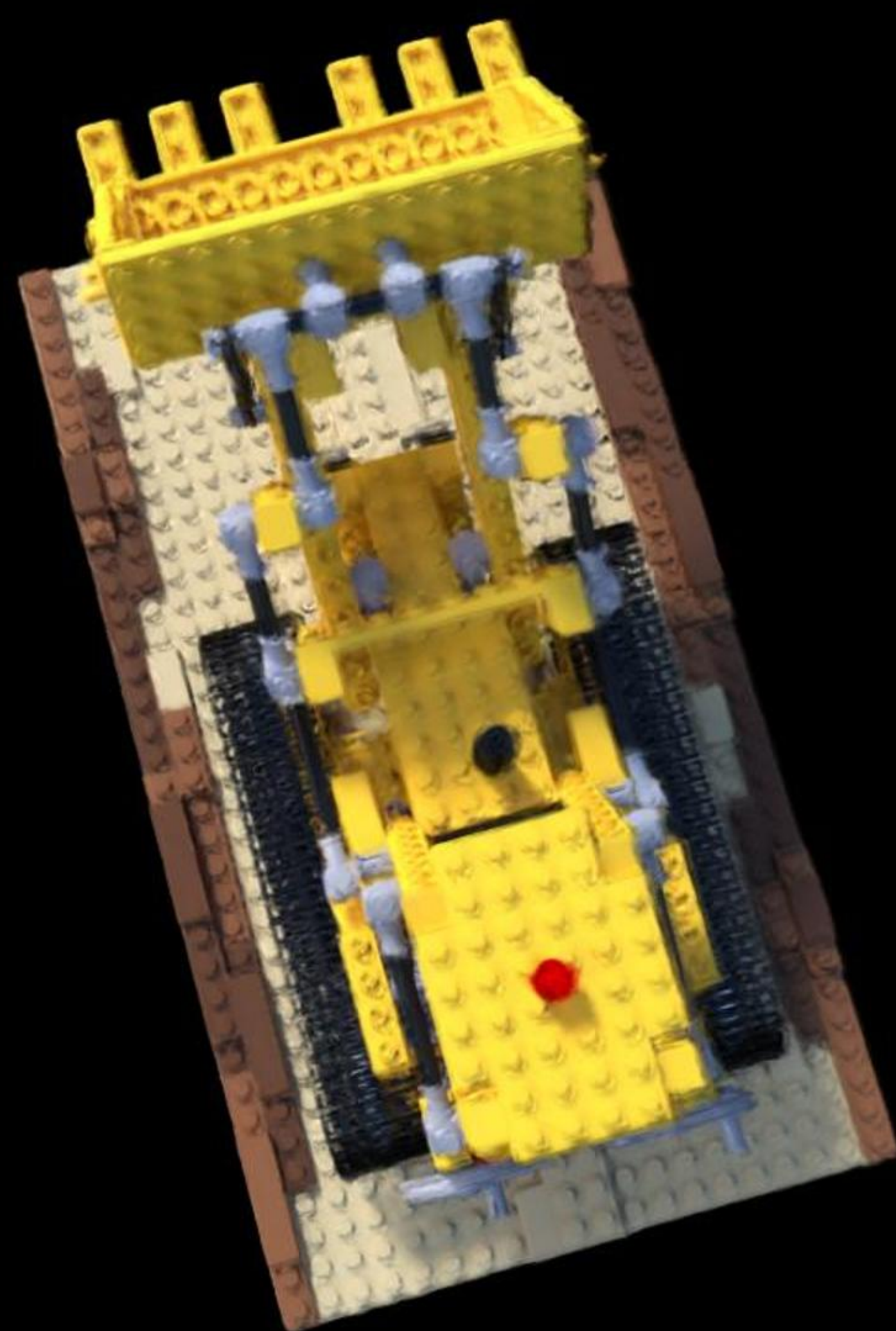
Config: VGGT | voxels | num_points=87000 PSNR: 19.05 | LPIPS: 0.1211 | SSIM: 0.7407
