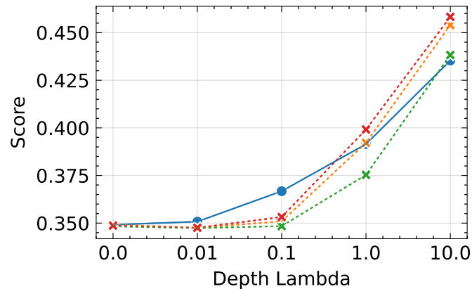
LPIPS \downarrow
