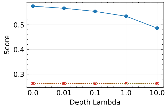
SSIM \uparrow
