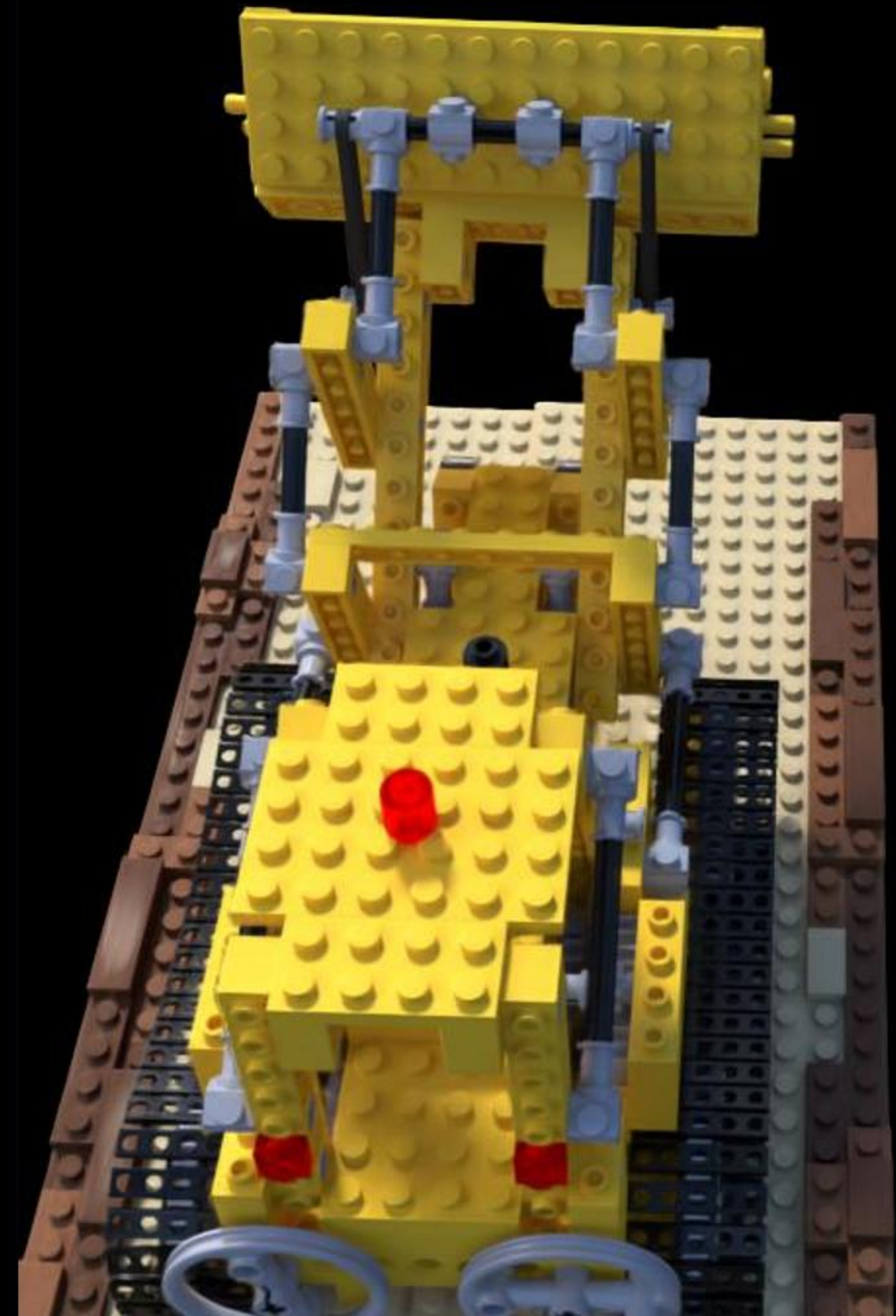
Config: COLMAP | | | 10092.0 PSNR: 10.64 | LPIPS: 0.5840 | SSIM: 0.5065
