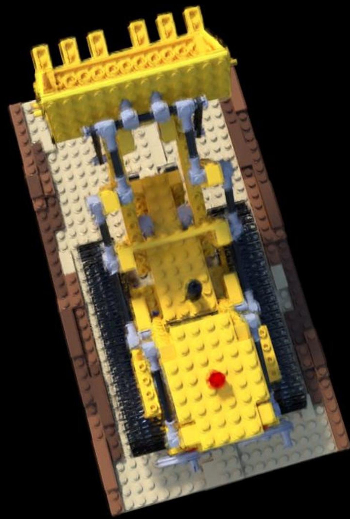
Config: VGGT | 95700.0 | Use BA PSNR: 21.92 | LPIPS: 0.0942 | SSIM: 0.8063
