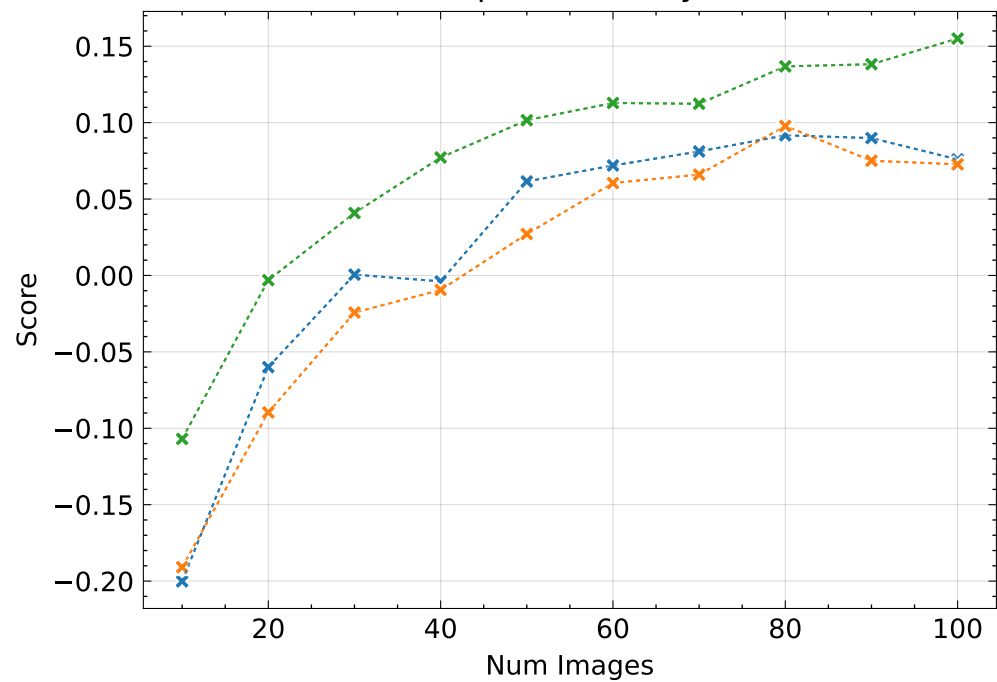
Composite Quality ↑
