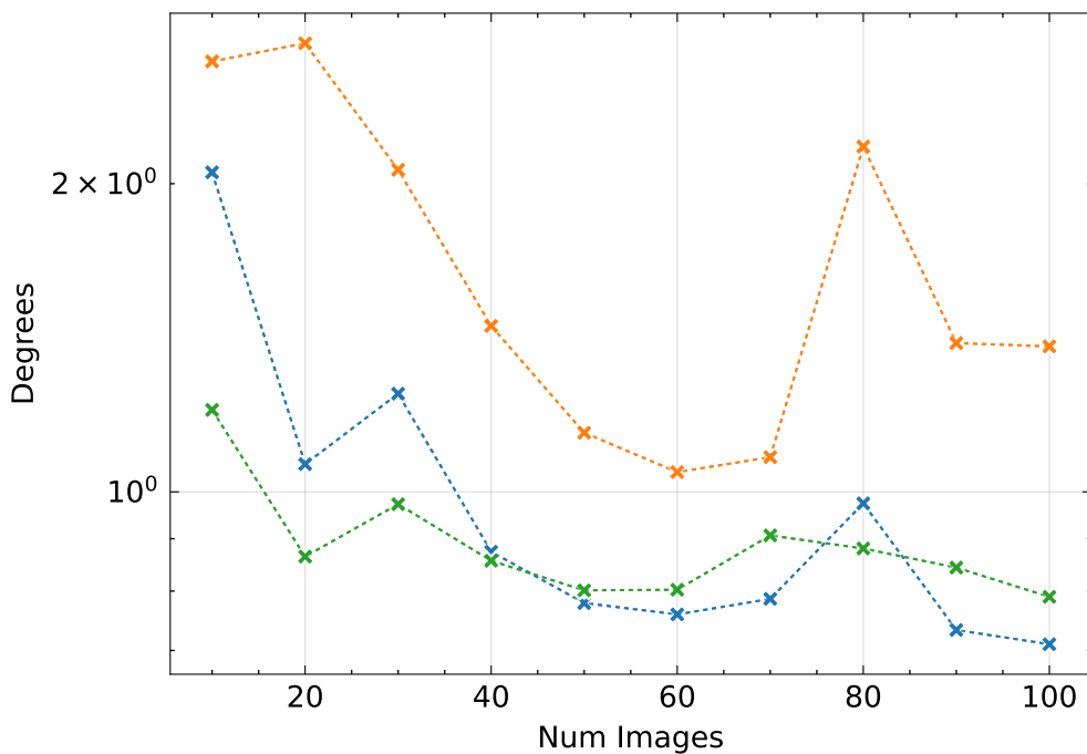
Aligned Cameras ↑
