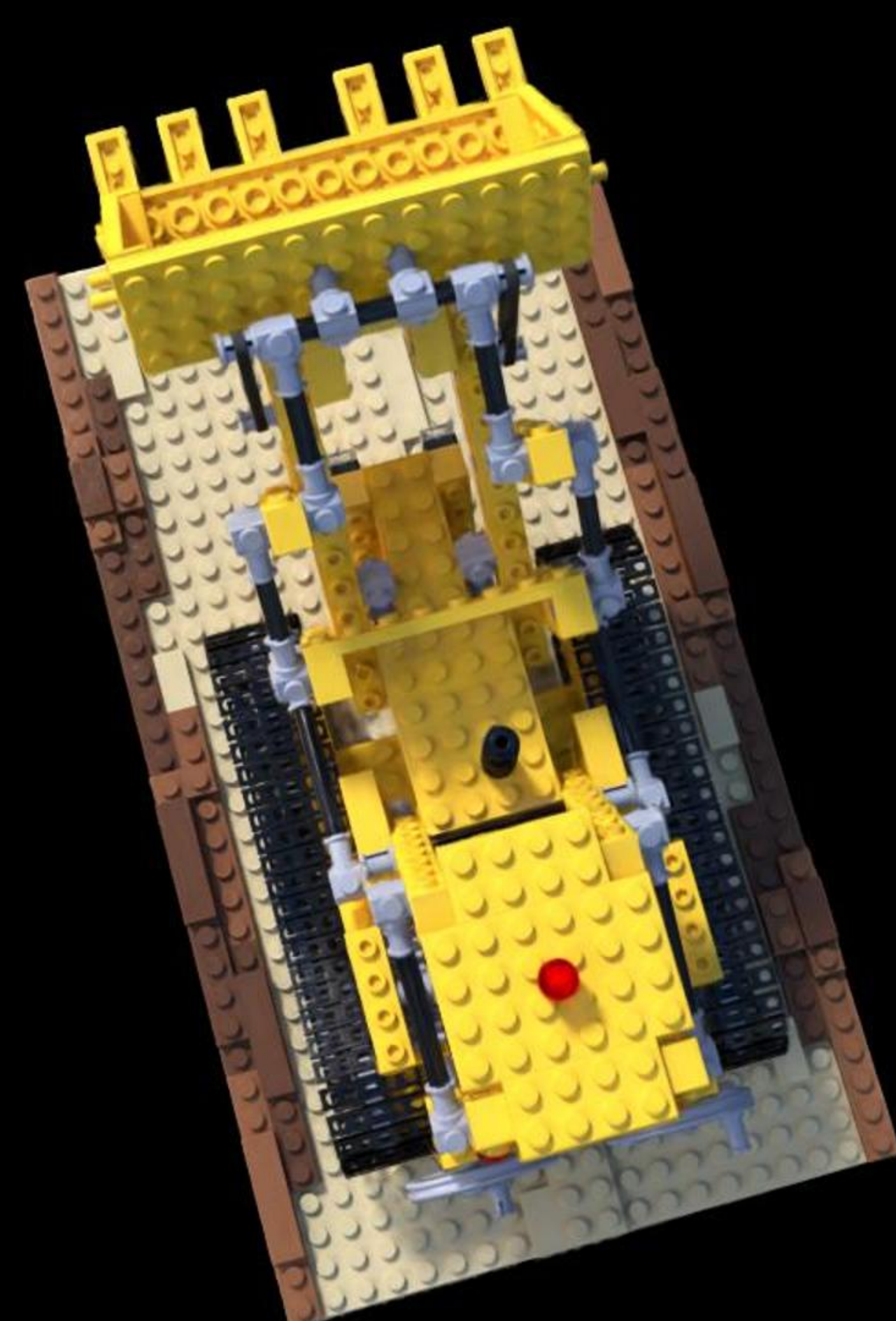
Config: VGGT | | ba | num_images=70 PSNR: 17.69 | LPIPS: 0.1025 | SSIM: 0.7199
