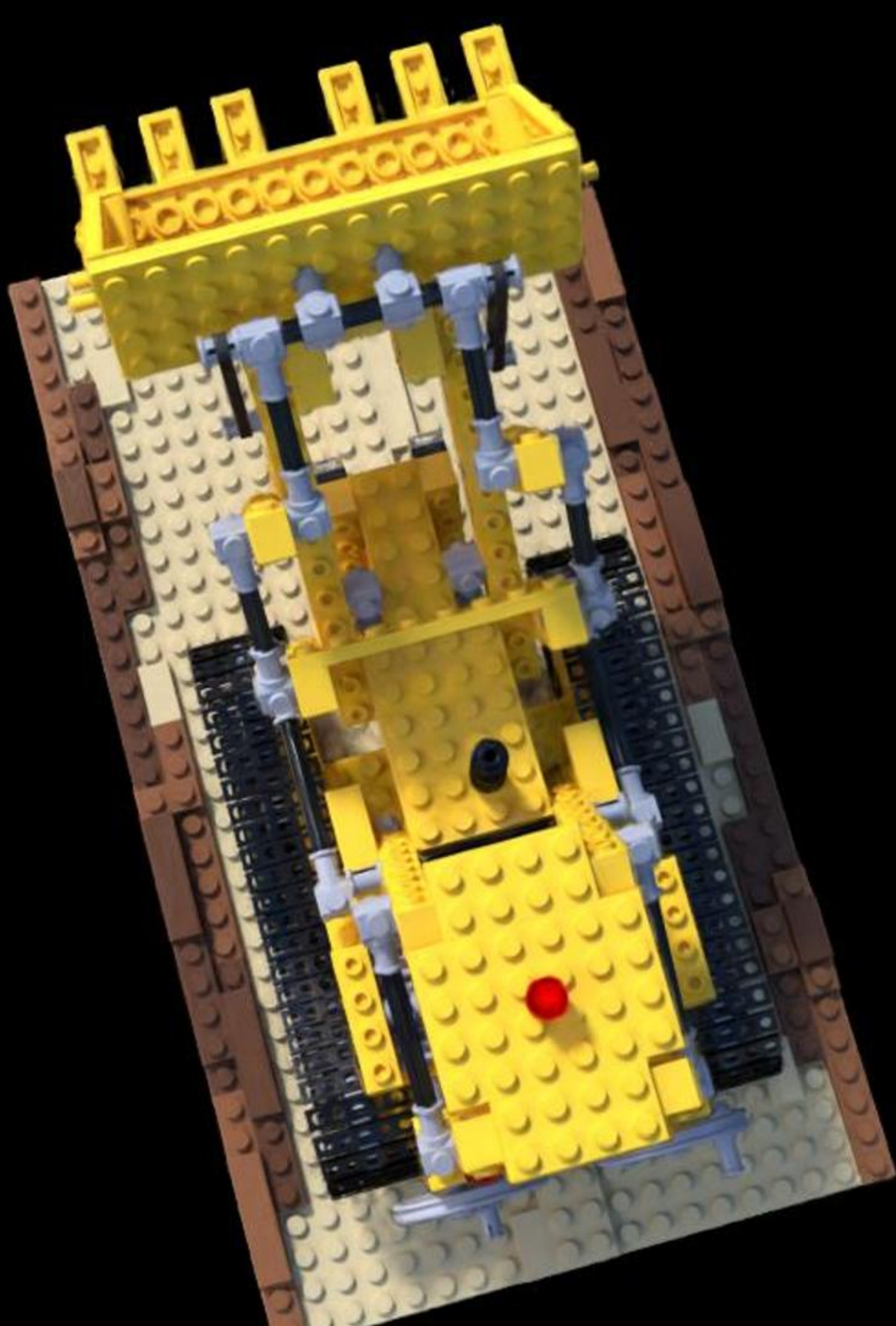
Config: VGGT | | voxels | num_images=70 PSNR: 19.28 | LPIPS: 0.0874 | SSIM: 0.7710
