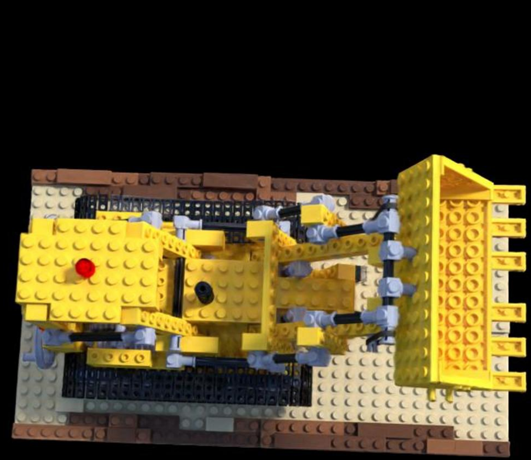
Config: VGGT | Shared Cam | ba | num_images=70 PSNR: 23.67 | LPIPS: 0.0525 | SSIM: 0.8592
