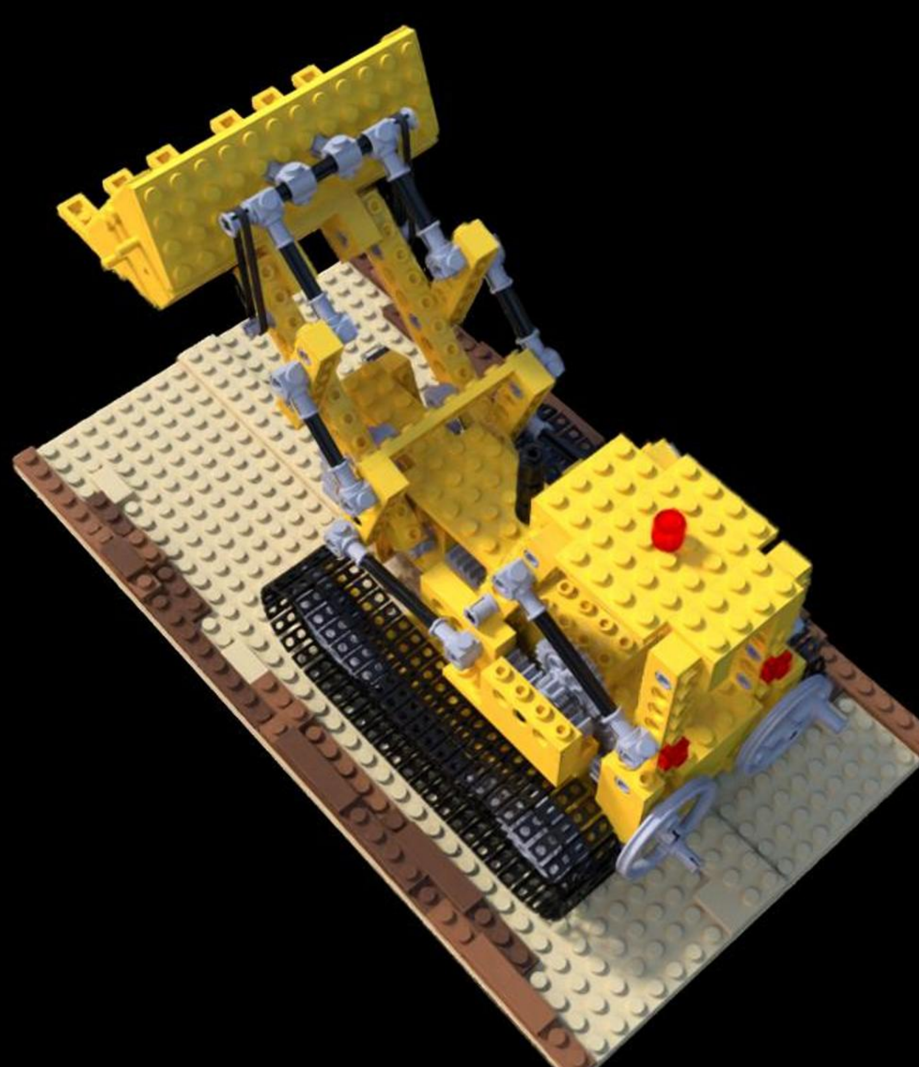
Config: VGGT | | voxels | num_images=70 PSNR: 18.27 | LPIPS: 0.0865 | SSIM: 0.7439
