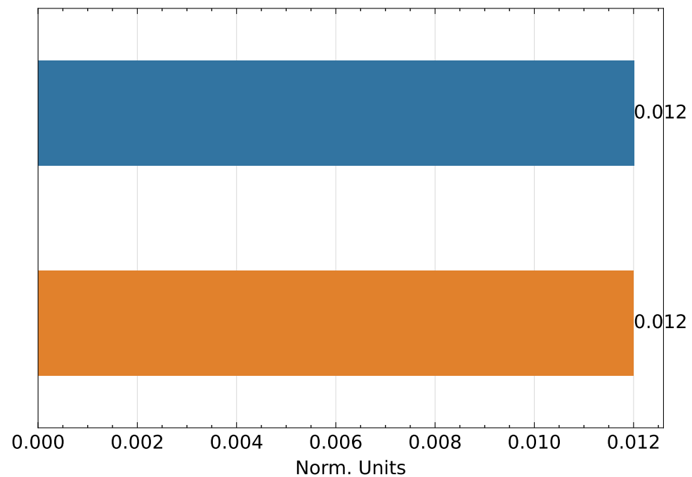
Composite Quality ↑
